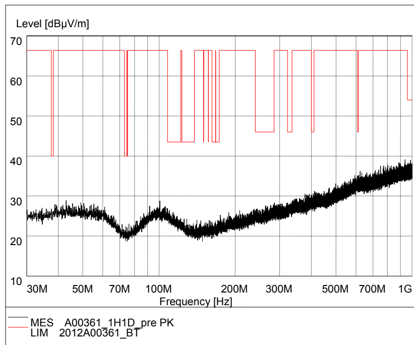
Fig.64. Radiated emission: GFSK, Channel 78, 30 MHz - 1 GHz
