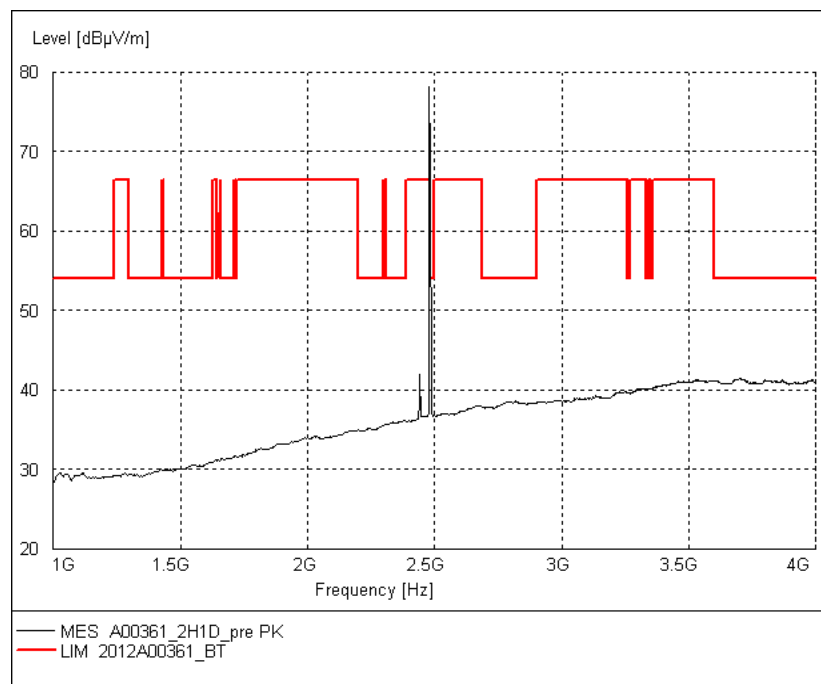
Fig.65. Radiated emission: GFSK, Channel 78, 1 GHz - 4 GHz
