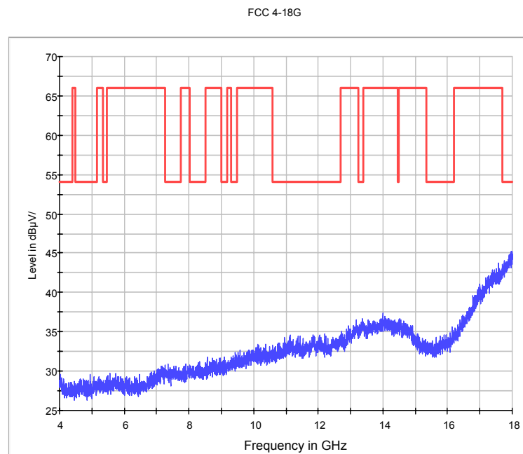
Fig.75. Radiated emission: \pi/4 DQPSK, Channel 39, 4 GHz - 18 GHz
