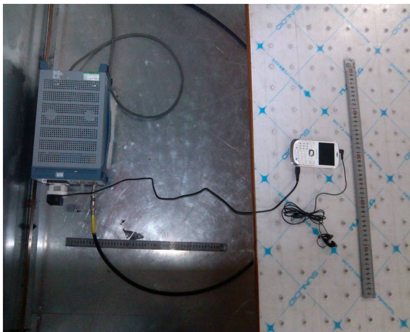
Conducted Emissions Test Setup
