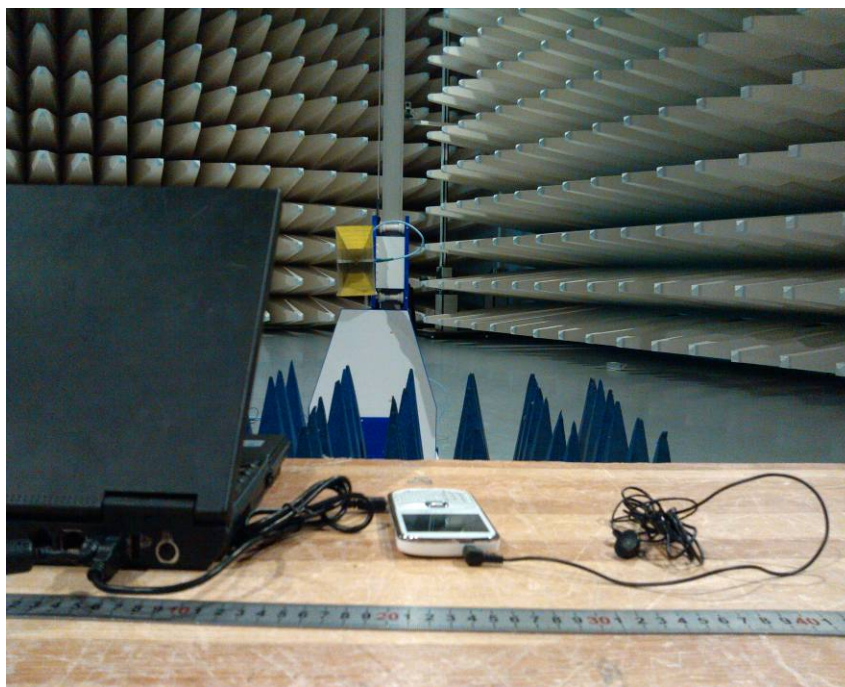
Radiated Emissions Test Setup
