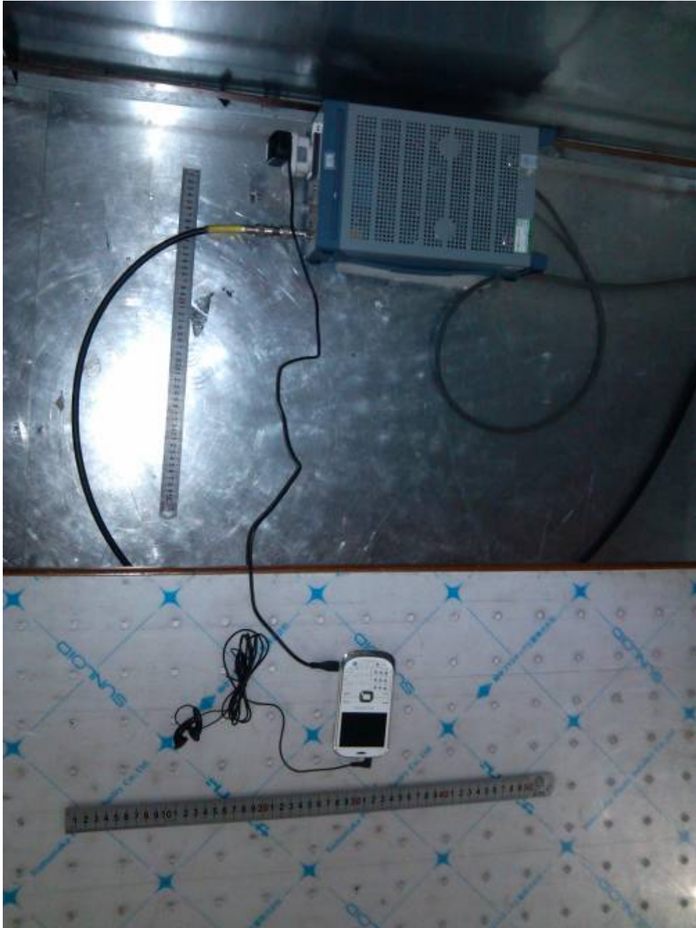
AC Power Line Conducted Emission Test setup
