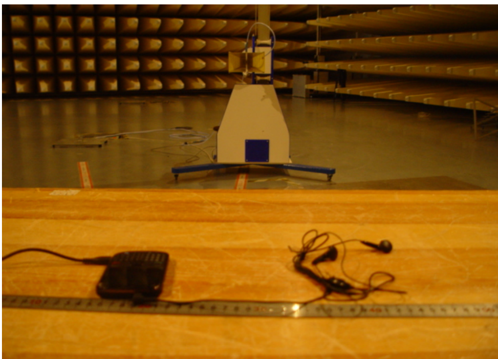
Receiver Spurious Emissions Test Setup
