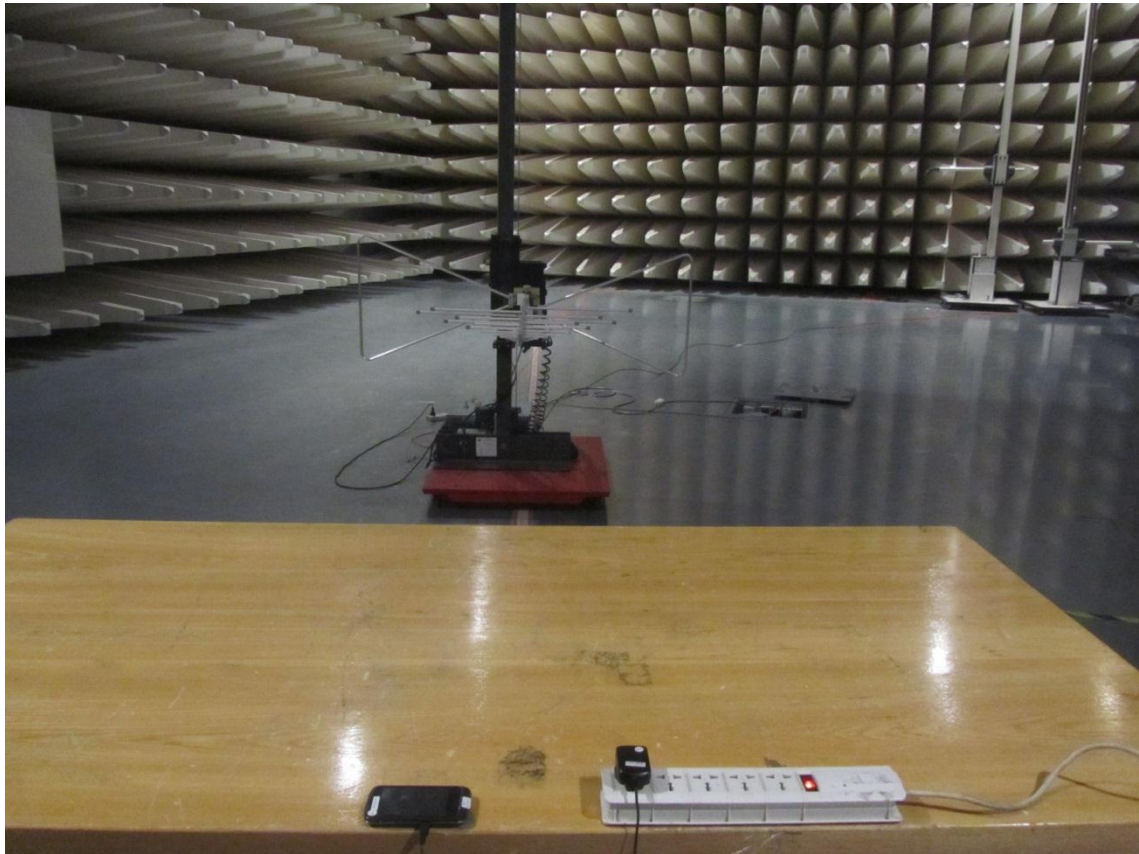
Part15C Radiated Emission
