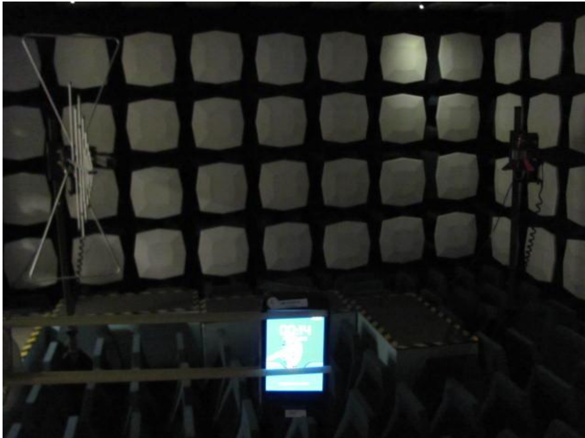
Part22/24/27 radiated spurious emission
