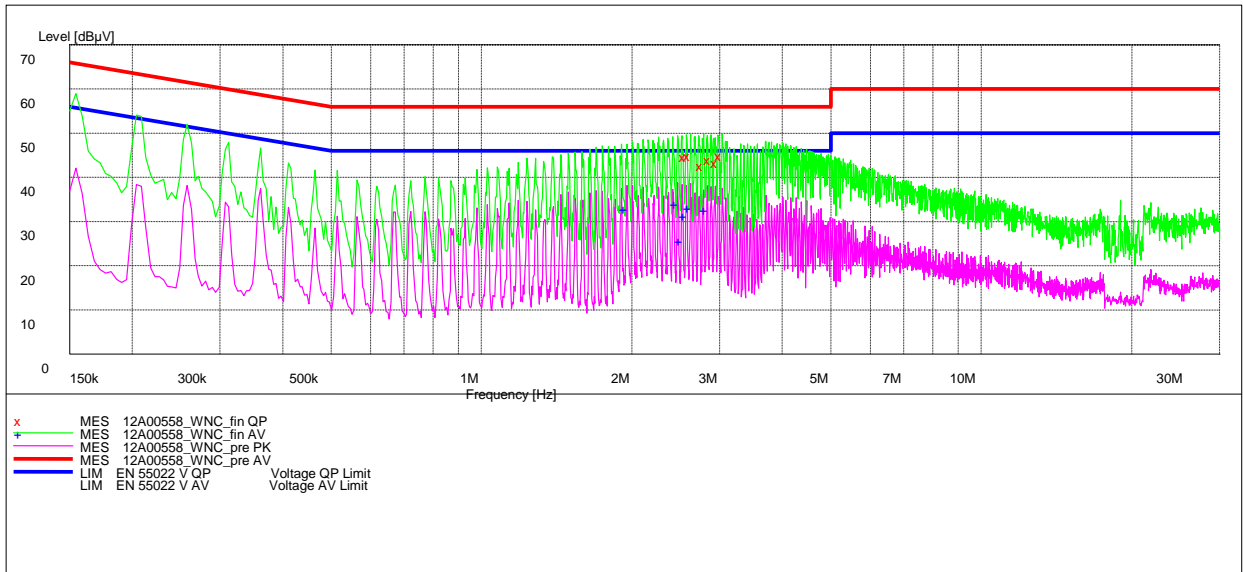
Fig. 77 AC Powerline Conducted Emission-802.11b
