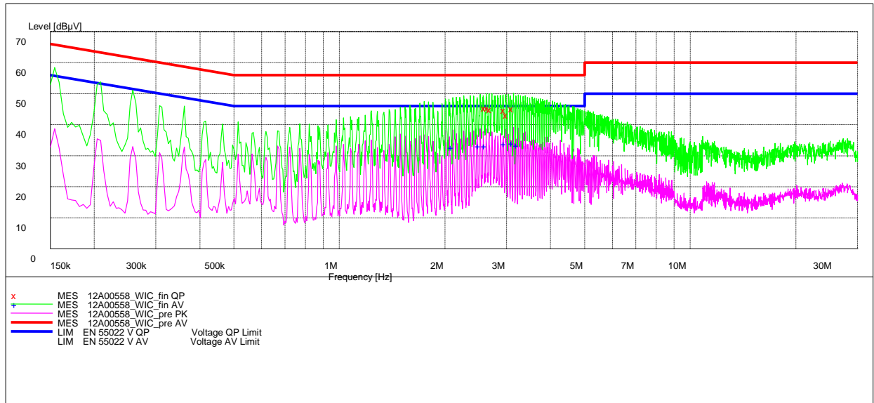
Fig. 78 AC Powerline Conducted Emission-802.11g
