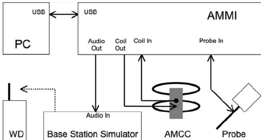
Figure 2 T-Coil Test Measurement Set-up
