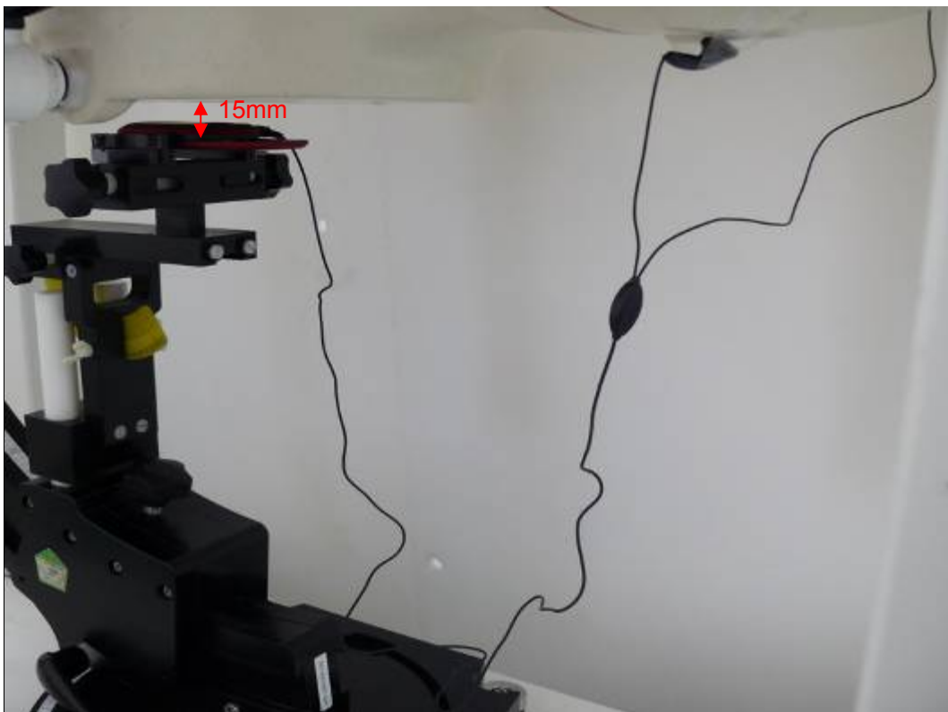
Picture 18: Body with Stereo Headset 1, The EUT display towards ground, the distance from EUT to the bottom of the Phantom is 15mm (Slide Open)
