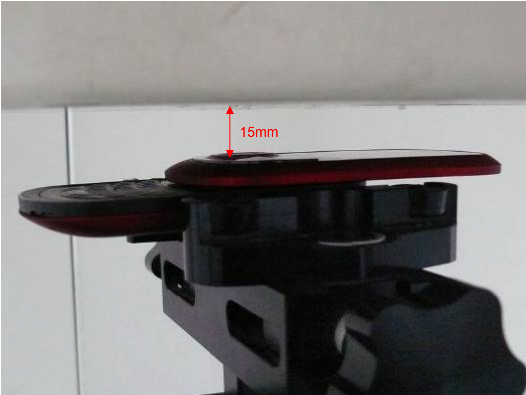
Picture 17: Body, The EUT display towards phantom, the distance from EUT to the bottom of the Phantom is 15mm (Slide Open)
