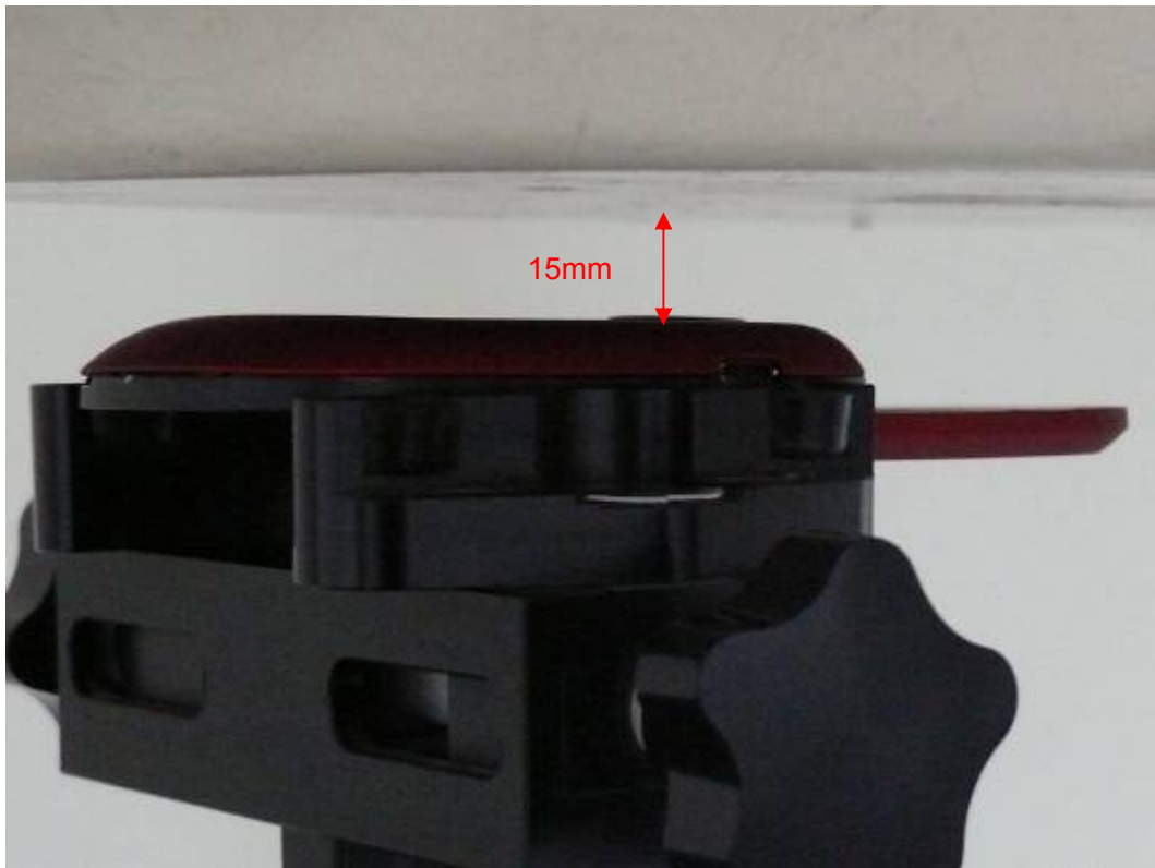
Picture 15: Body, The EUT display towards ground, the distance from EUT to the bottom of the Phantom is 15mm (Slide Open)
