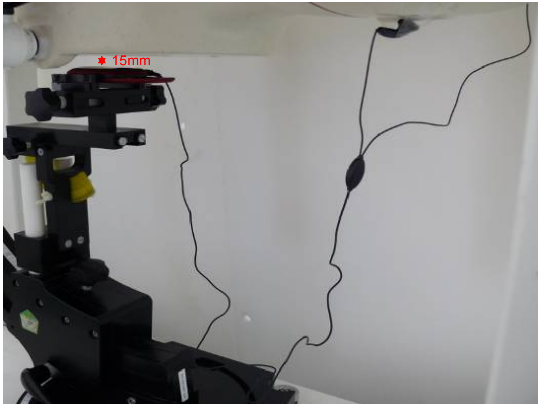
Picture 19: Body with Stereo Headset 2, The EUT display towards ground, the distance from EUT to the bottom of the Phantom is 15mm (Slide Open)
