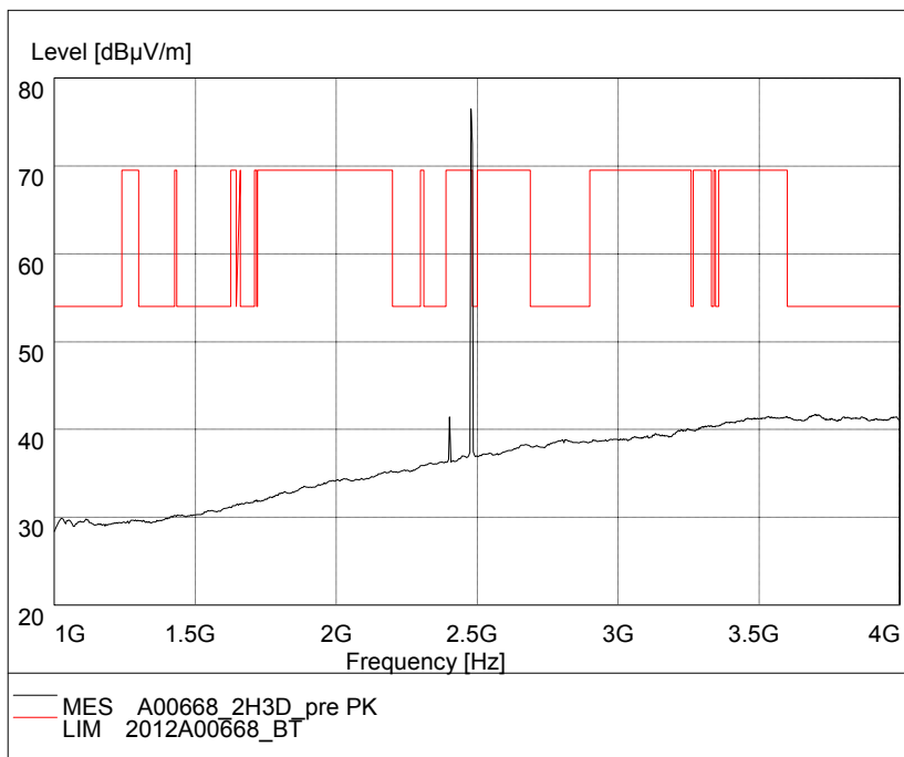
Fig.89. Radiated emission: 8DPSK, Channel 78, 1 GHz - 4 GHz
