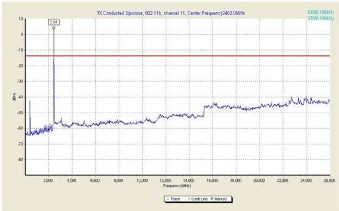
Fig. 22 Conducted Spurious Emission (802.11b, Ch11, 30 MHz-26 GHz)
