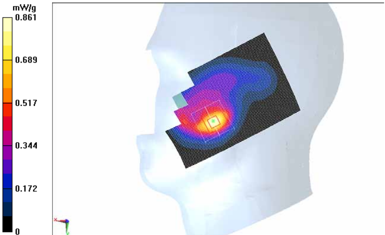
1900 MHz CH661
