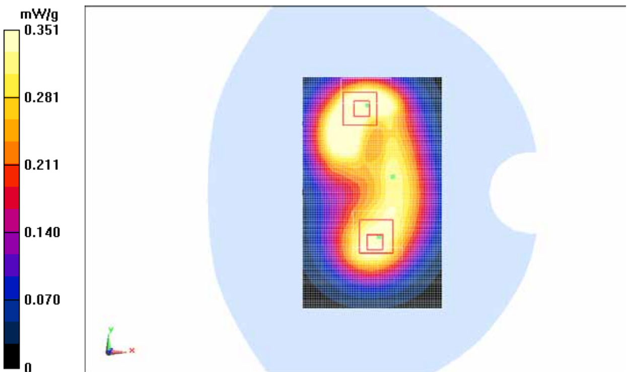
Fig. 35 1900 MHz CH512
