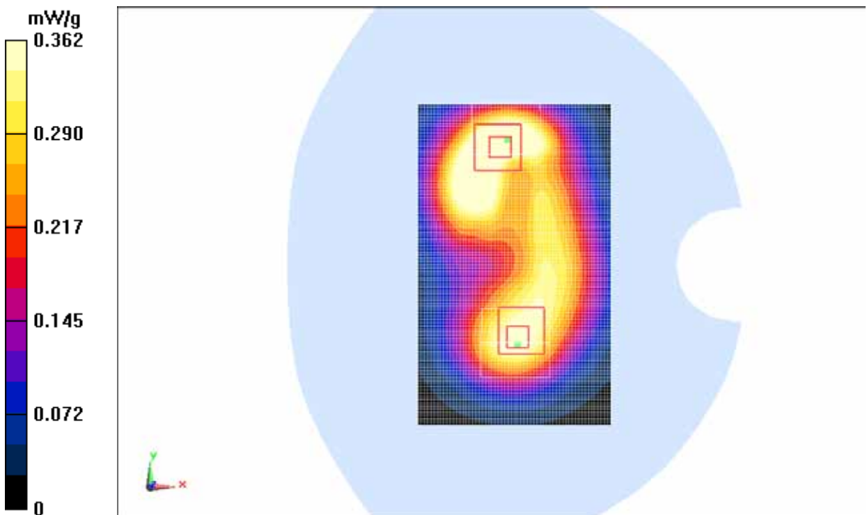
Fig. 34 1900 MHz CH661
