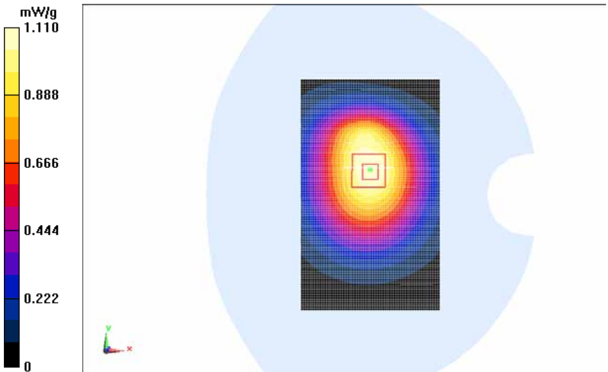
850 MHz CH251
