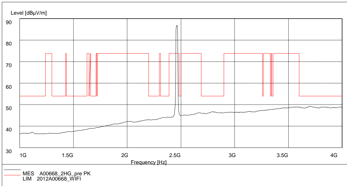
Fig. 49 Radiated Spurious Emission (802.11g, Ch11, 1 GHz-4 GHz)
