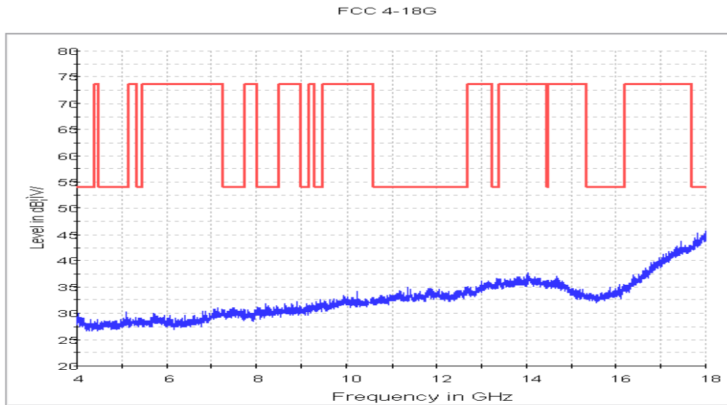
Fig. 32 Radiated Spurious Emission (802.11b, Ch1, 4 GHz-18 GHz)
