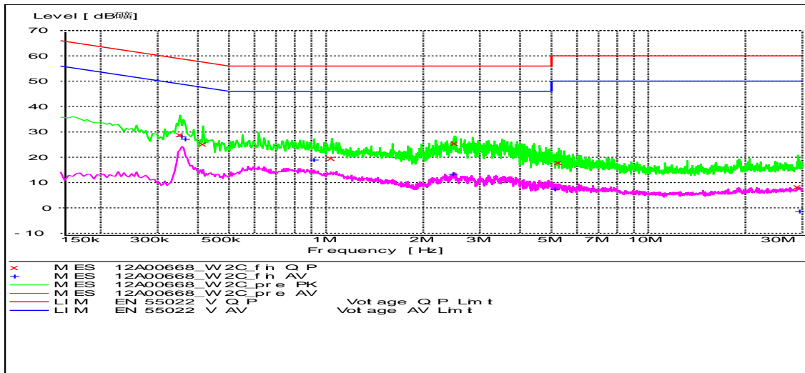
Fig. 53 AC Powerline Conducted Emission-802.11g with charger 2
