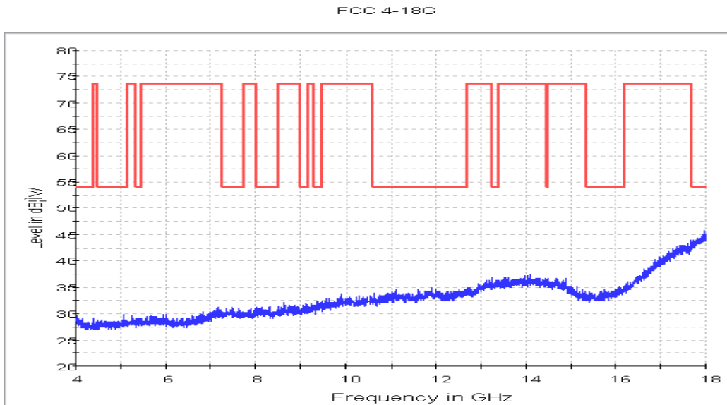
Fig. 43 Radiated Spurious Emission (802.11g, Ch1, 4 GHz-18 GHz)
