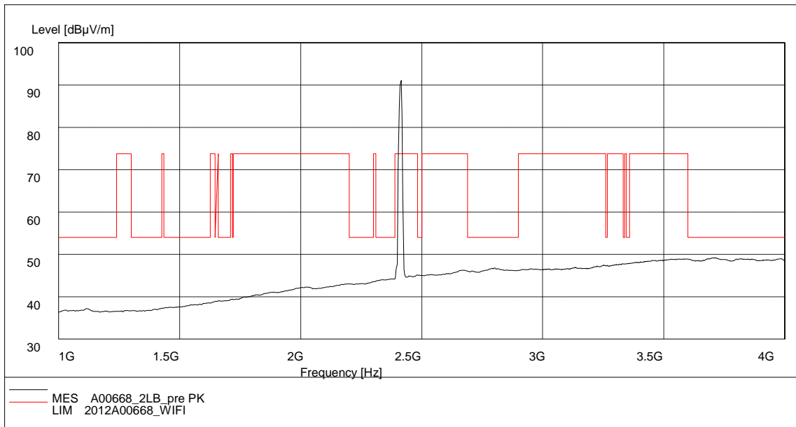
Fig. 31 Radiated Spurious Emission (802.11b, Ch1, 1 GHz-4 GHz)
