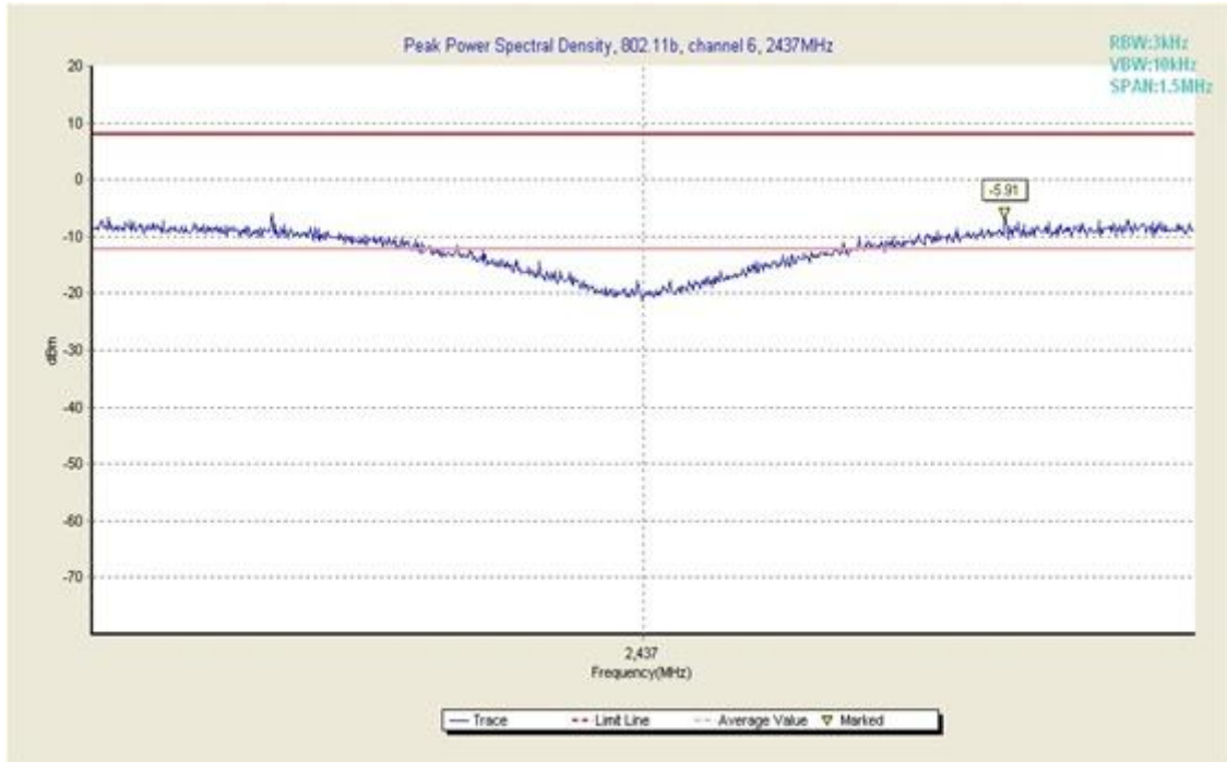
Fig. 2 Power Spectral Density (802.11b, Ch 6)
