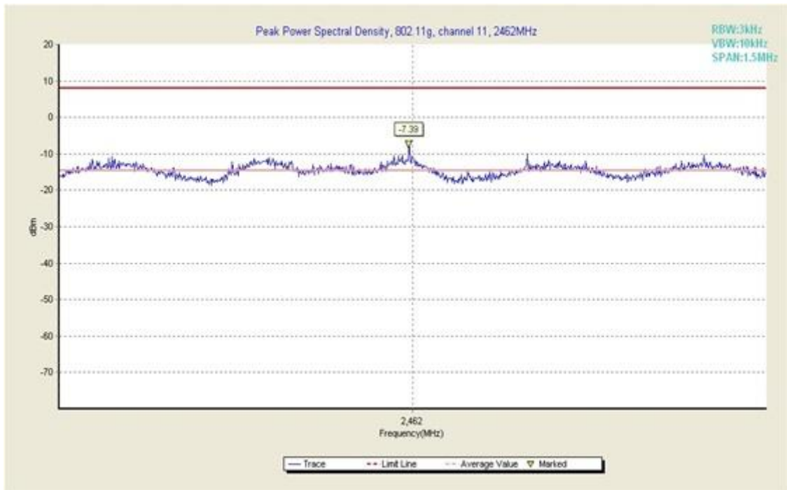
Fig. 6 Power Spectral Density (802.11g, Ch 11)
