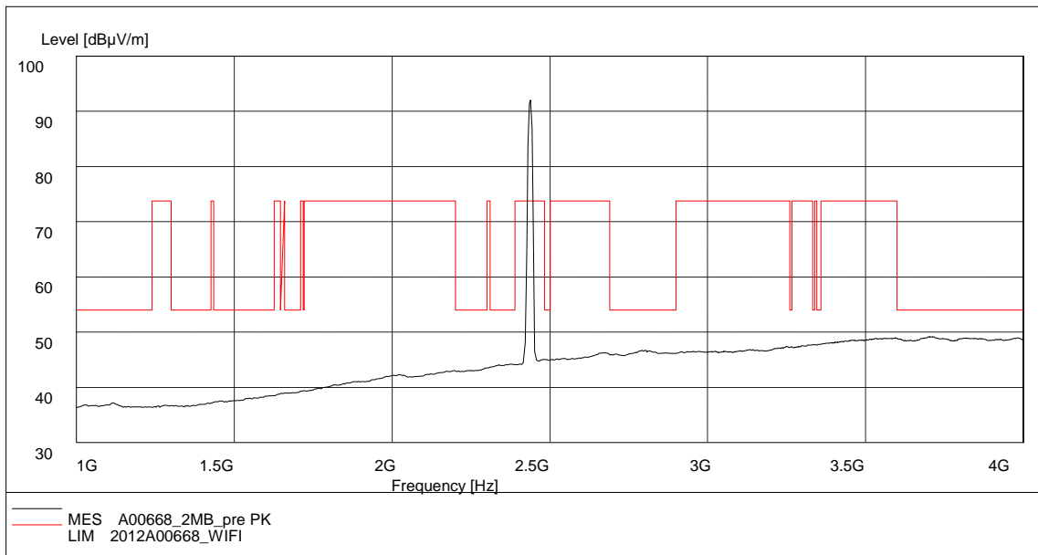
Fig. 34 Radiated Spurious Emission (802.11b, Ch6, 1 GHz-4 GHz)
