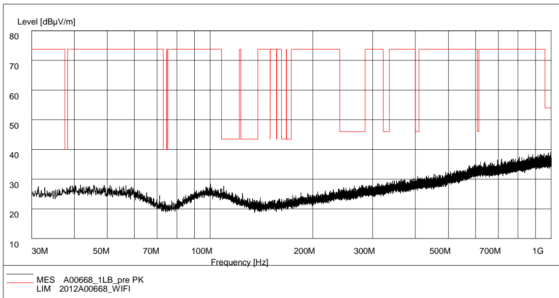
Fig. 30 Radiated Spurious Emission (802.11b, Ch1, 30 MHz-1 GHz)
