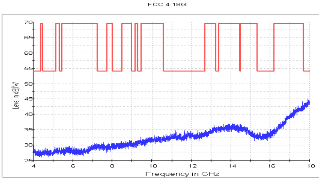
Fig. 39 Radiated Spurious Emission (802.11b, Ch11, 4 GHz-18 GHz)
