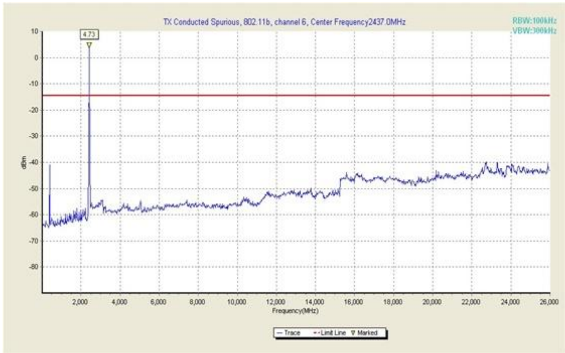
Fig. 20 Conducted Spurious Emission (802.11b, Ch6, 30 MHz-26 GHz)
