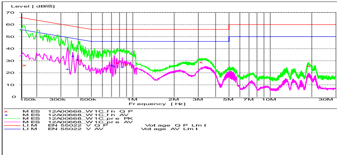
Fig. 52 AC Powerline Conducted Emission-802.11g with charger 1
