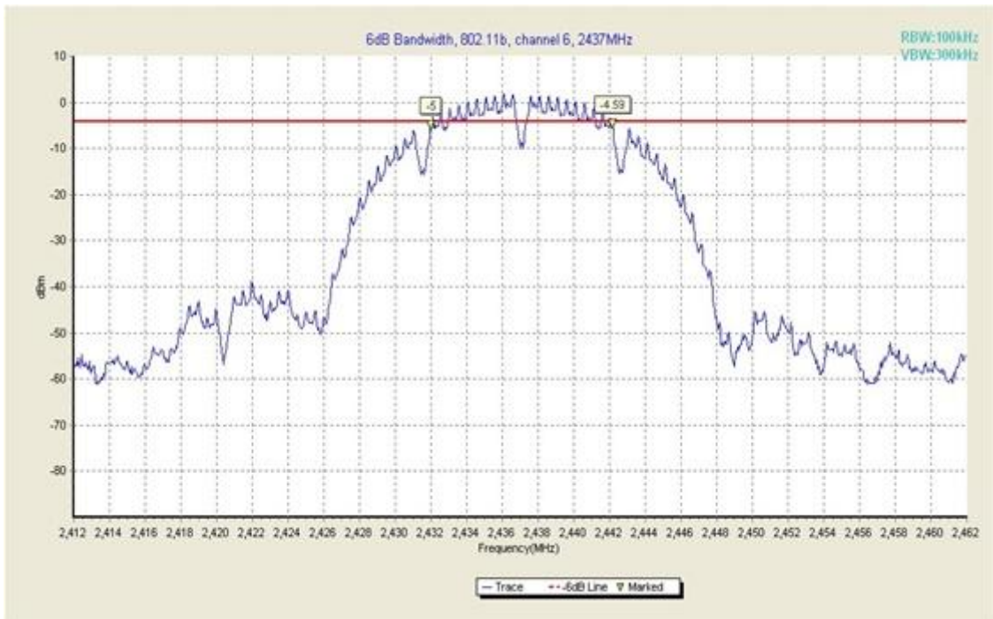
Fig. 8 Occupied 6dB Bandwidth (802.11b, Ch 6)
