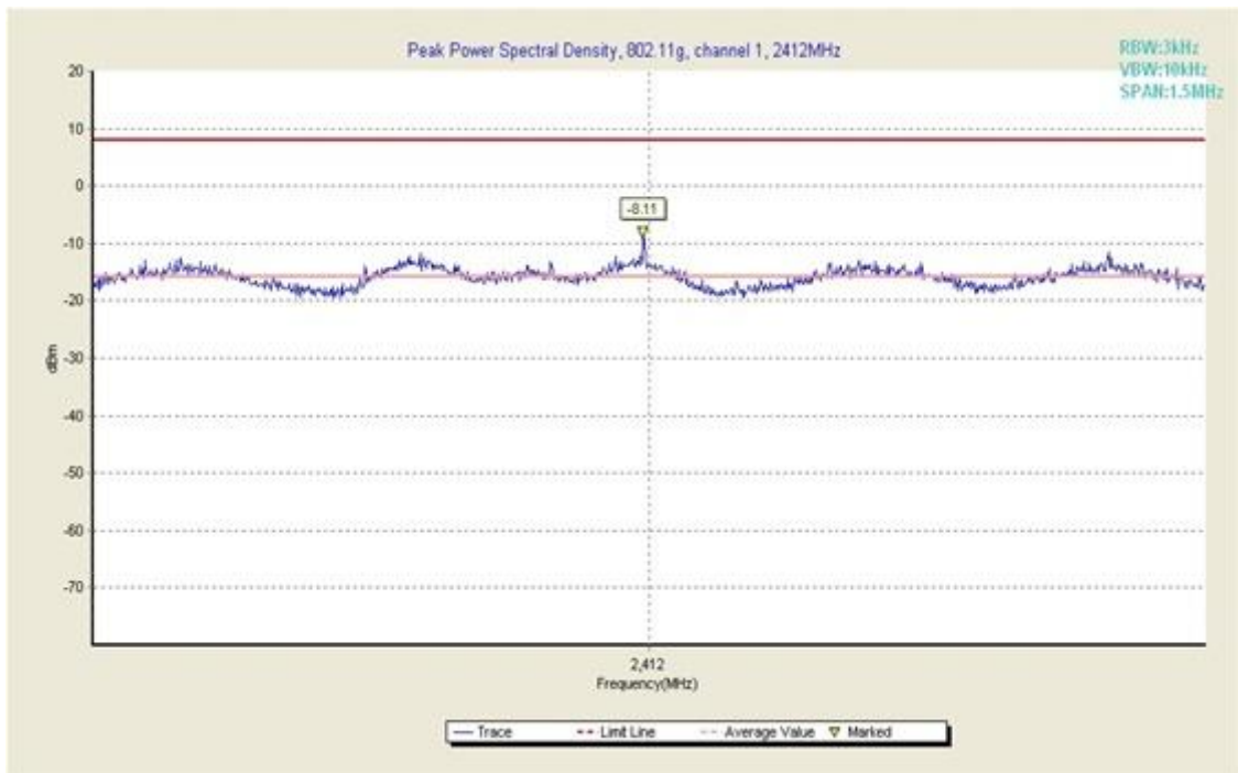
Fig. 4 Power Spectral Density (802.11g, Ch 1)
