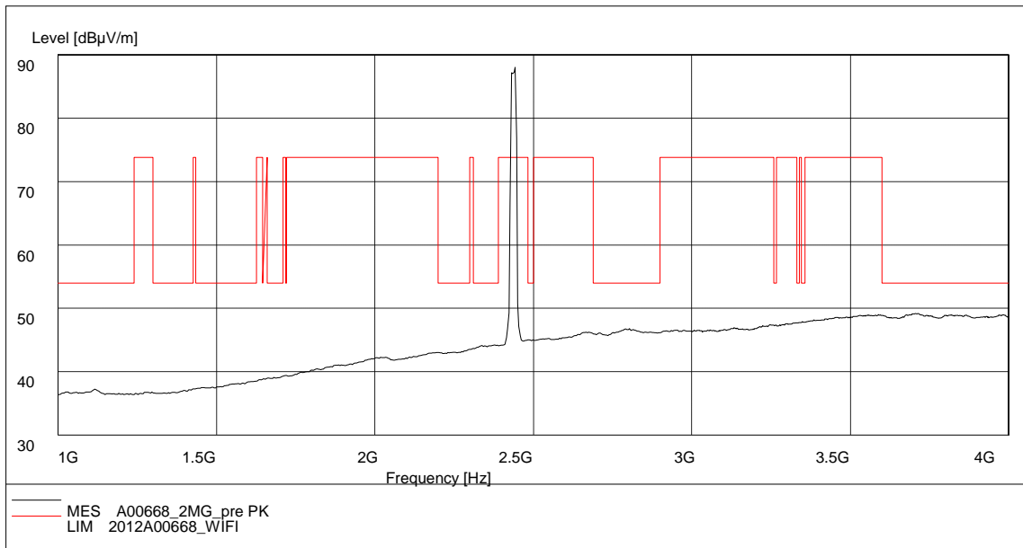
Fig. 45 Radiated Spurious Emission (802.11g, Ch6, 1 GHz-4 GHz)
