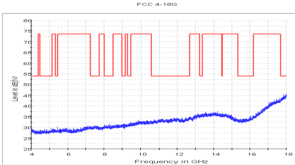
Fig. 46 Radiated Spurious Emission (802.11g, Ch6, 4 GHz-18 GHz)
