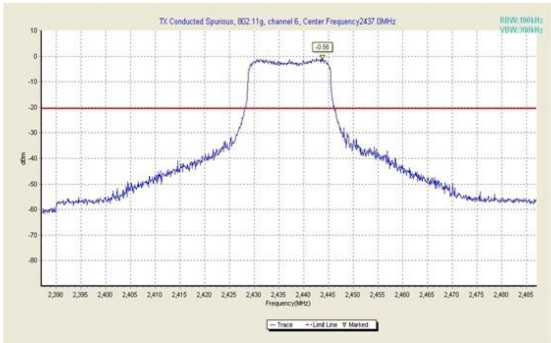
Fig. 25 Conducted Spurious Emission (802.11g, Ch6, Center Frequency)
