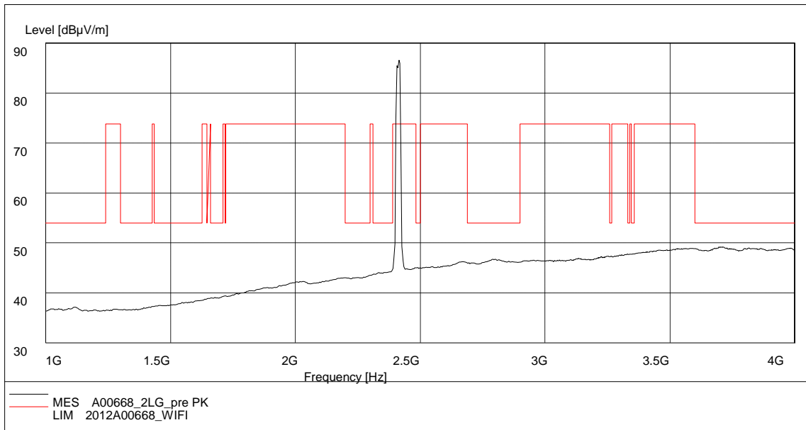
Fig. 42 Radiated Spurious Emission (802.11g, Ch1, 1 GHz-4 GHz)
