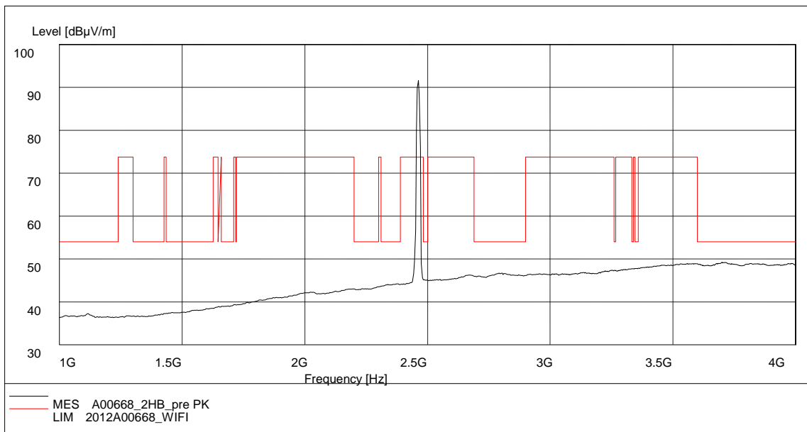
Fig. 38 Radiated Spurious Emission (802.11b, Ch11, 1 GHz-4 GHz)
