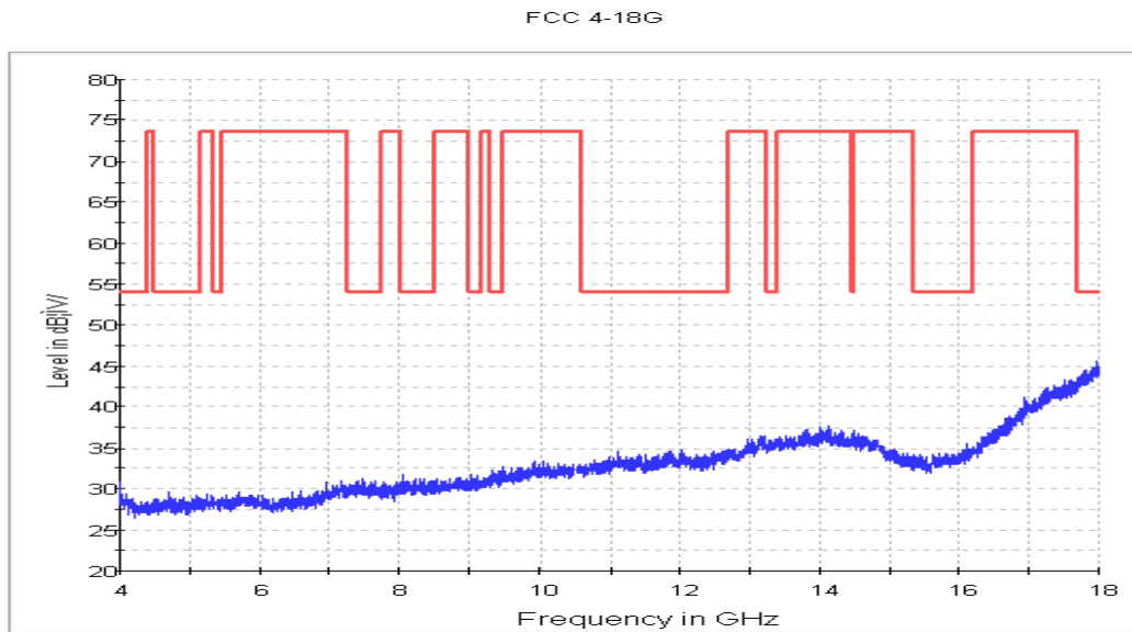
Fig. 50 Radiated Spurious Emission (802.11g, Ch11, 4 GHz-18 GHz)
