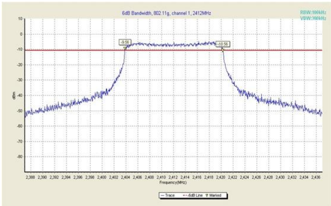
Fig. 10 Occupied 6dB Bandwidth (802.11g, Ch 1)
