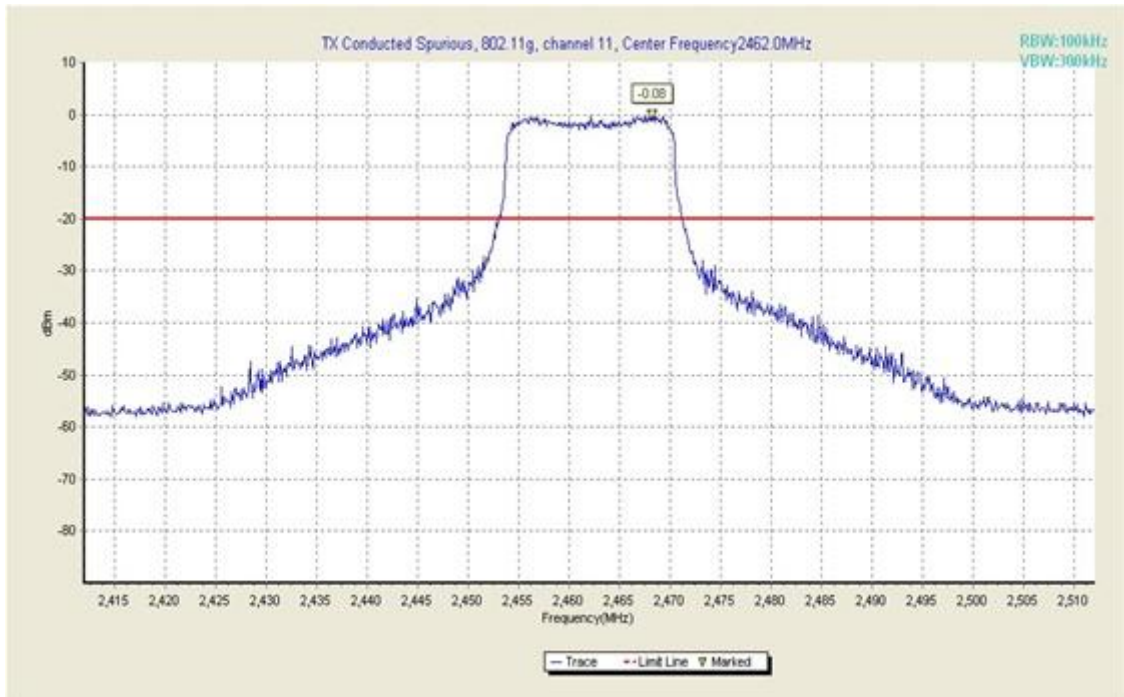
Fig. 27 Conducted Spurious Emission (802.11g, Ch11, Center Frequency)
