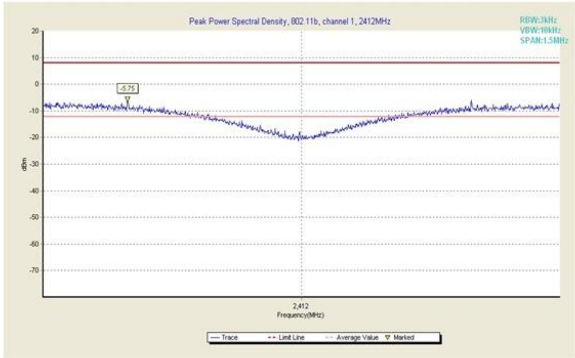
Fig. 1 Power Spectral Density (802.11b, Ch 1)
