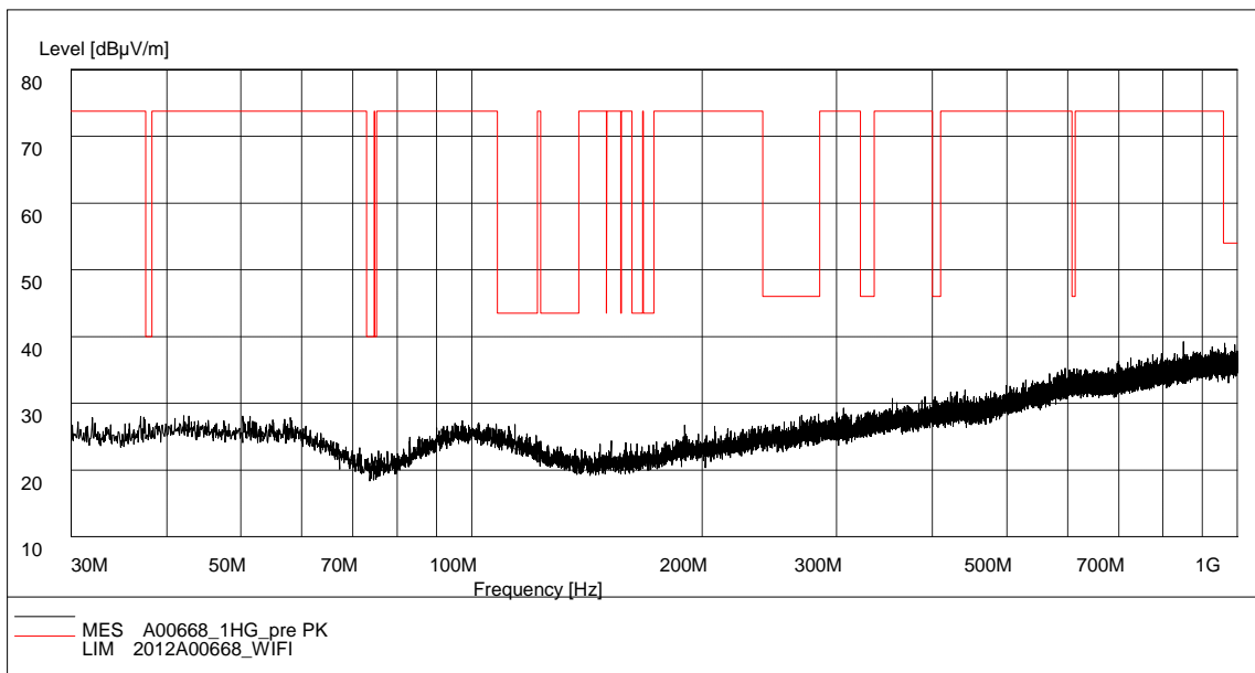
Fig. 48 Radiated Spurious Emission (802.11g, Ch11, 30 MHz-1 GHz)
