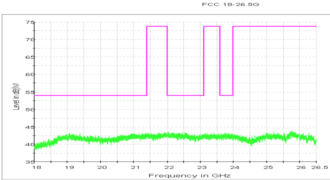
Fig. 51 Radiated emission: 18 GHz - 26.5 GHz
