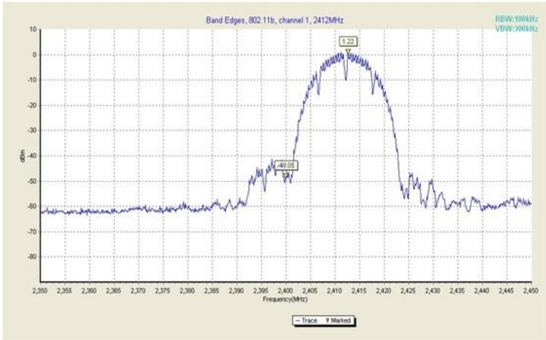
Fig. 13 Band Edges (802.11b, Ch 1)
