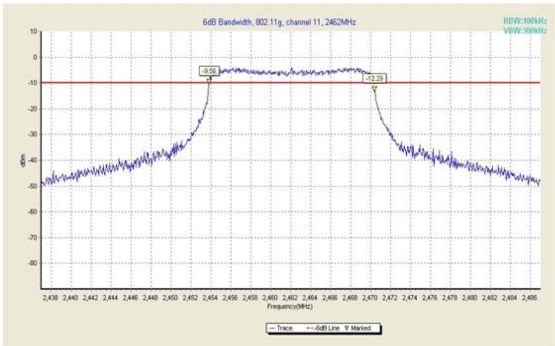
Fig. 12 Occupied 6dB Bandwidth (802.11g, Ch 11)
