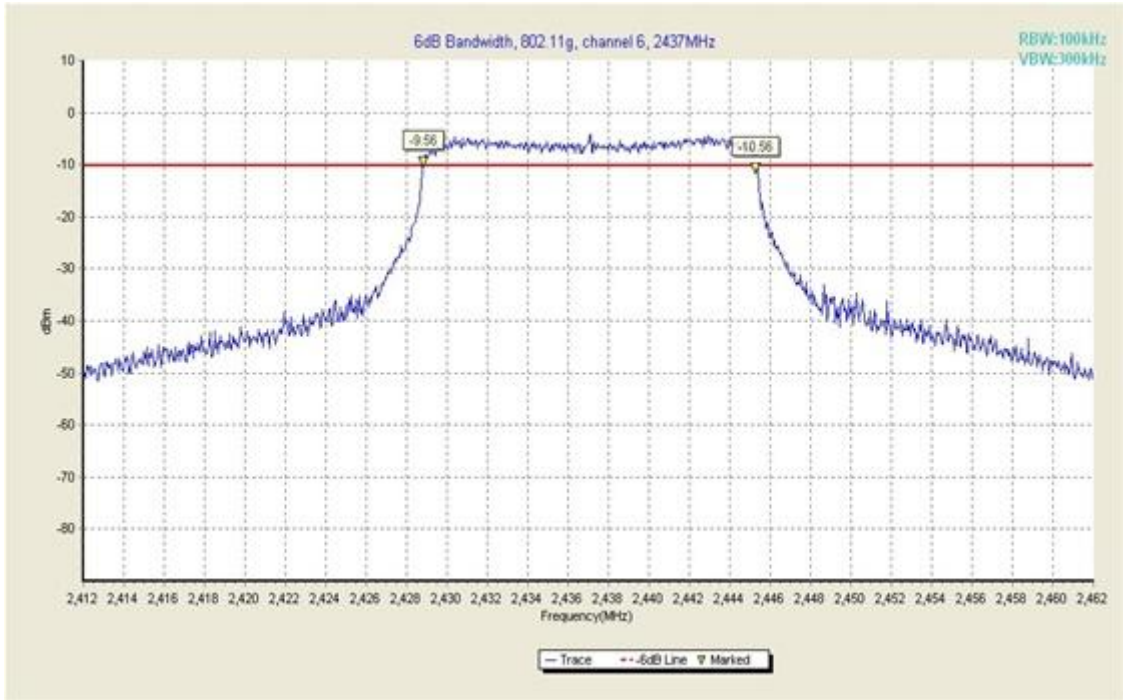
Fig. 11 Occupied 6dB Bandwidth (802.11g, Ch 6)
