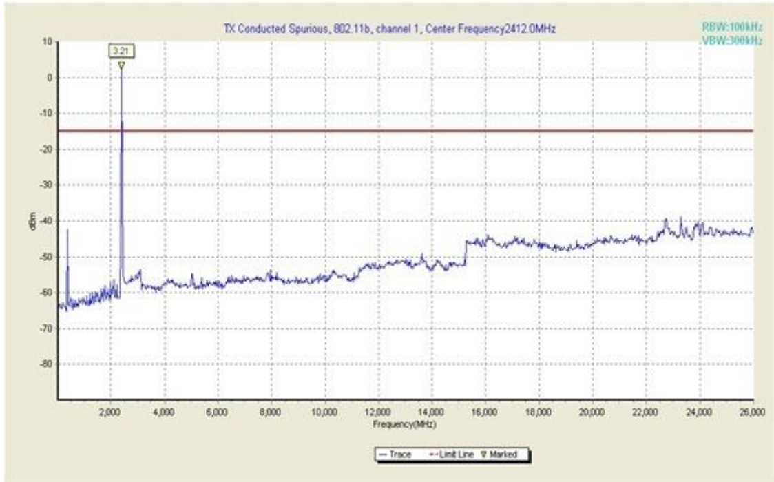
Fig. 18 Conducted Spurious Emission (802.11b, Ch1, 30 MHz-26 GHz)
