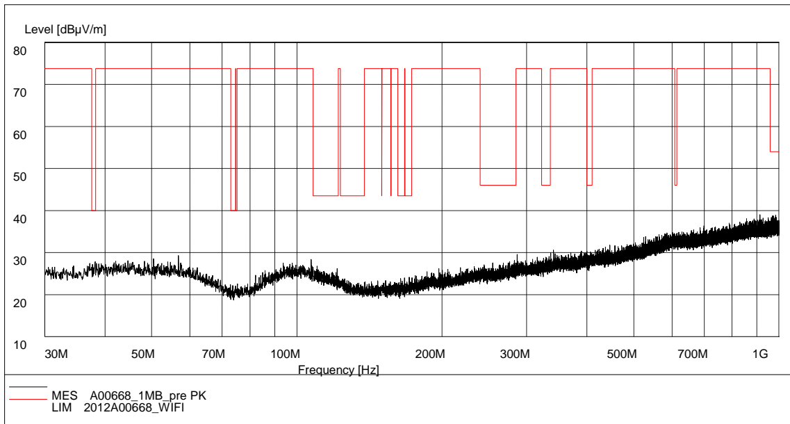
Fig. 33 Radiated Spurious Emission (802.11b, Ch6, 30 MHz-1 GHz)
