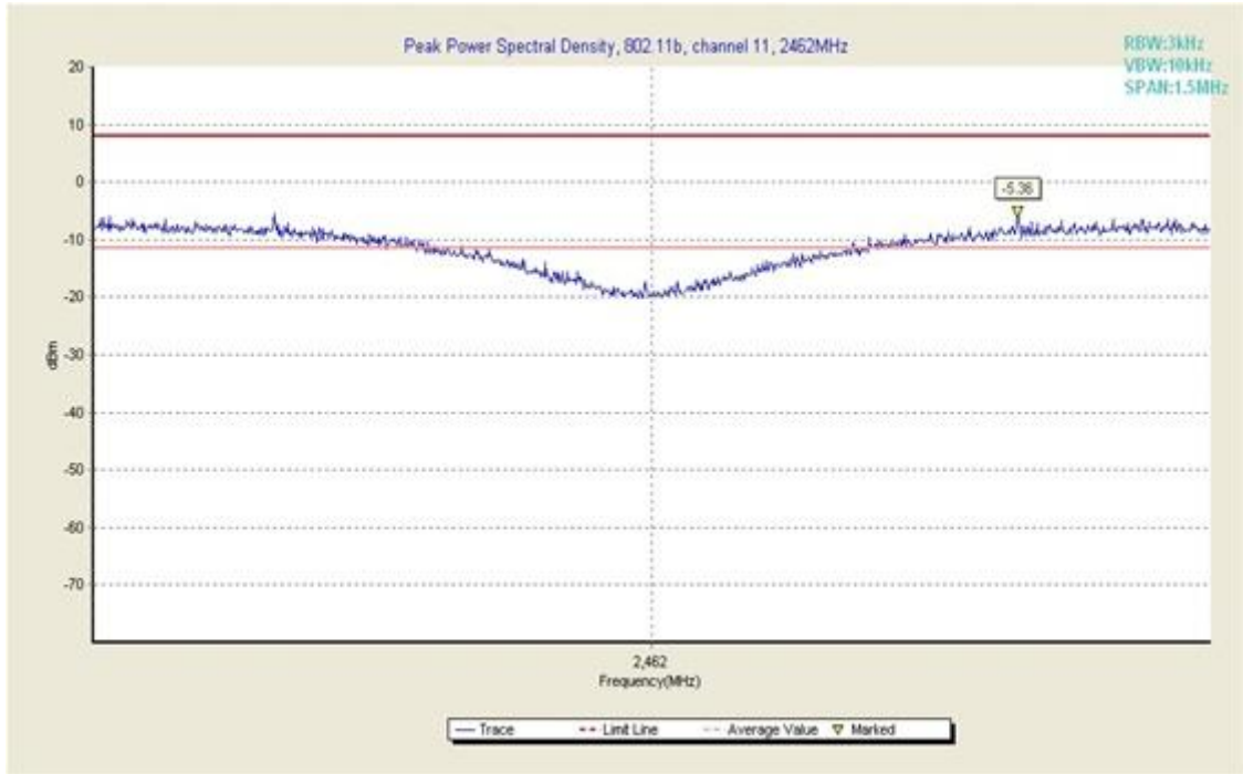
Fig. 3 Power Spectral Density (802.11b, Ch 11)
