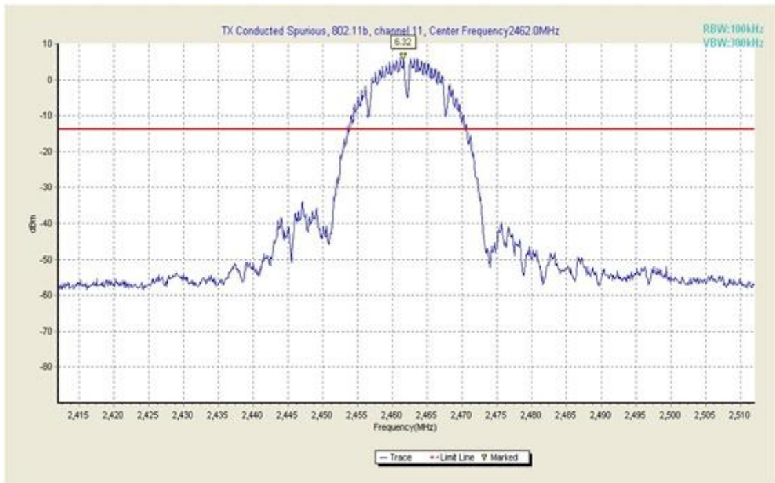
Fig. 21 Conducted Spurious Emission (802.11b, Ch11, Center Frequency)
