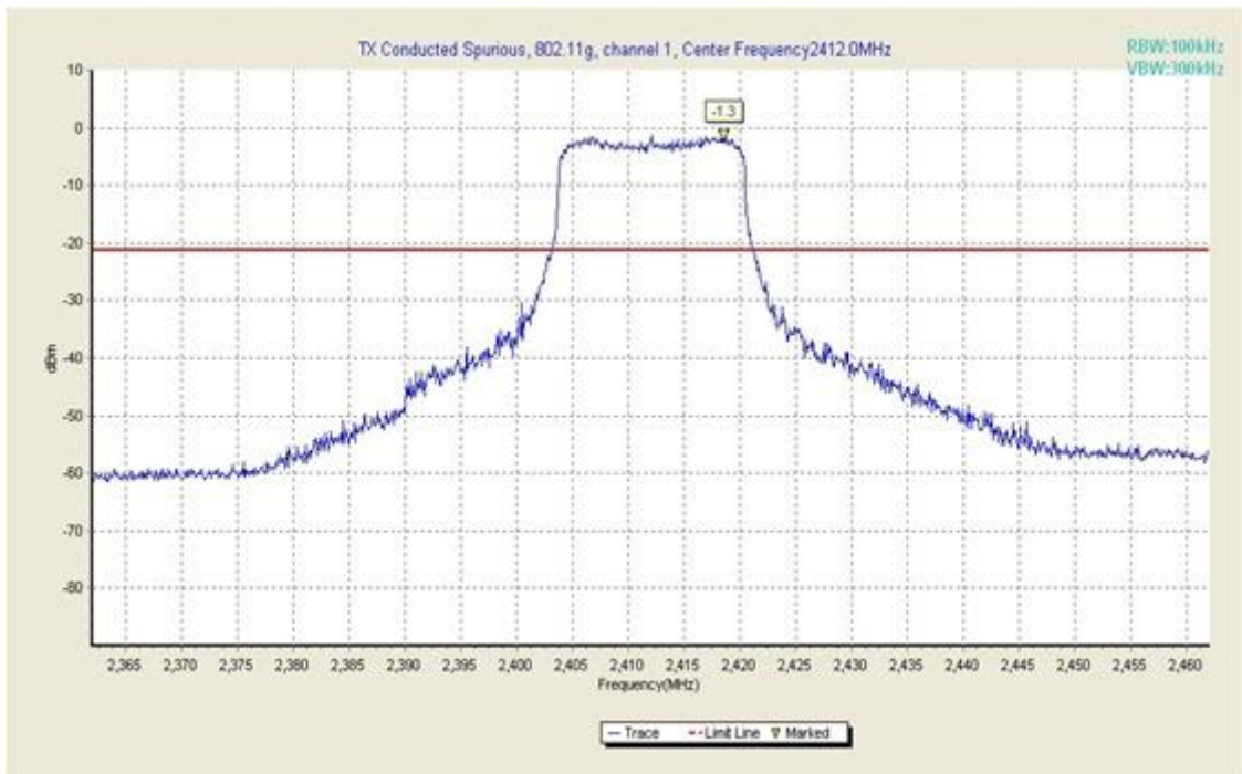
Fig. 23 Conducted Spurious Emission (802.11g, Ch1, Center Frequency)
