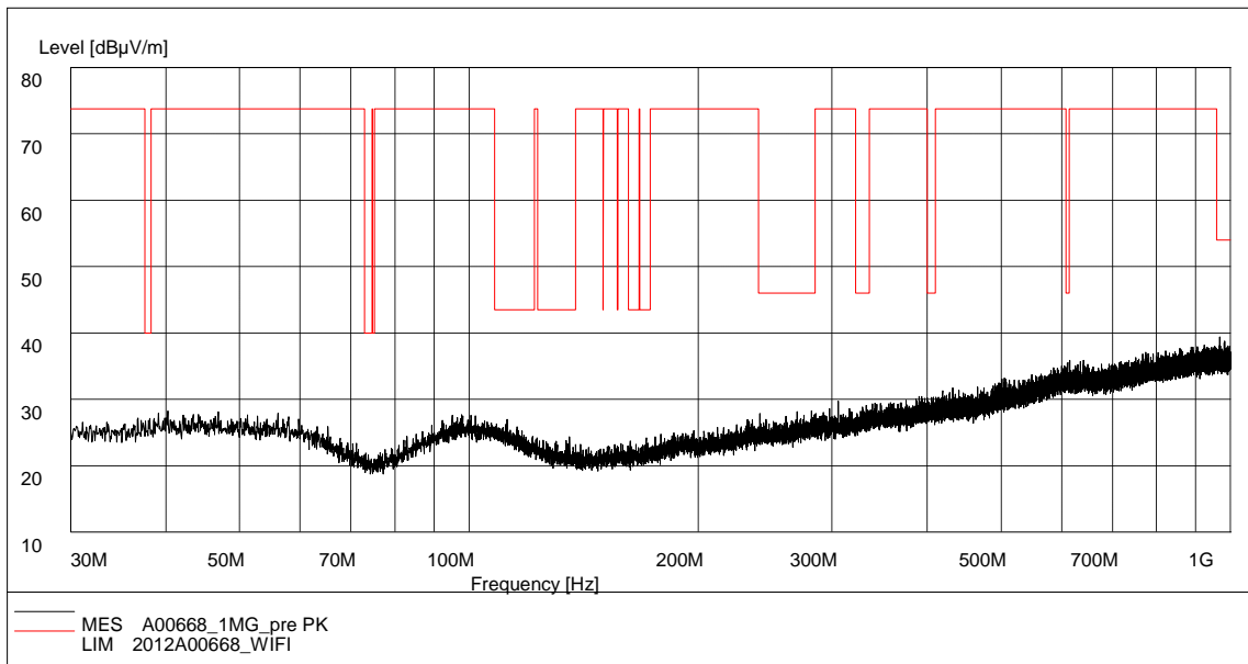
Fig. 44 Radiated Spurious Emission (802.11g, Ch6, 30 MHz-1 GHz)
