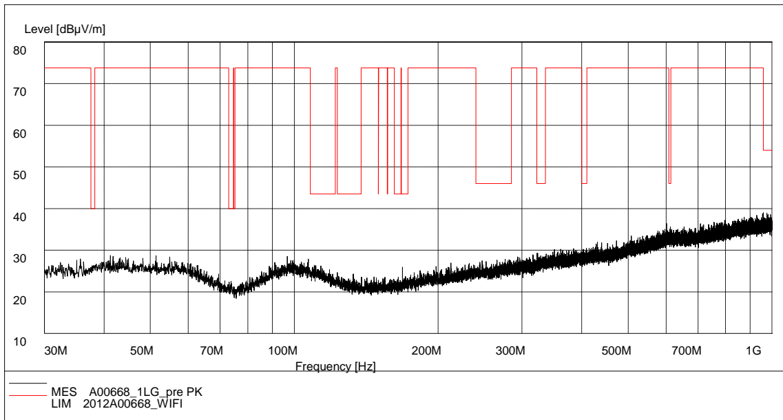
Fig. 41 Radiated Spurious Emission (802.11g, Ch1, 30 MHz-1 GHz)
