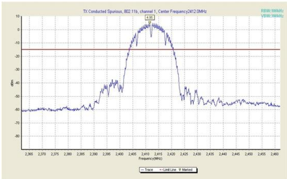
Fig. 17 Conducted Spurious Emission (802.11b, Ch1, Center Frequency)
