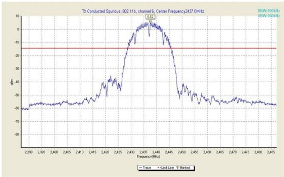
Fig. 19 Conducted Spurious Emission (802.11b, Ch6, Center Frequency)
