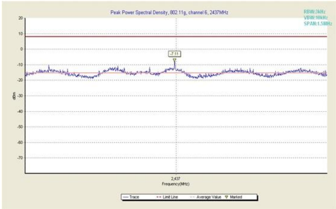
Fig. 5 Power Spectral Density (802.11g, Ch 6)
