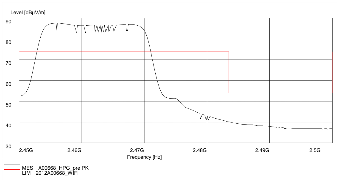
Fig. 47 Radiated Spurious Emission (Power): 802.11g, ch11, 2.45 GHz - 2.50GHz
