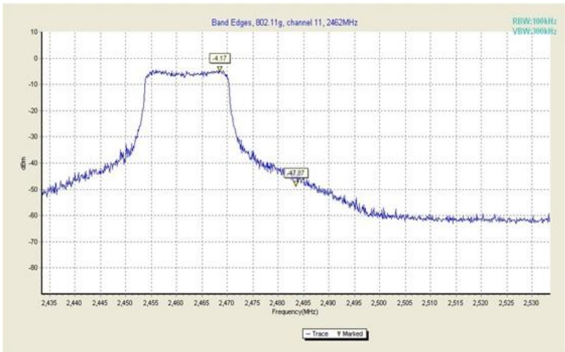
Fig. 16 Band Edges (802.11g, Ch 11)
