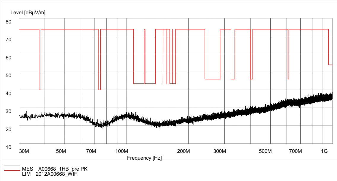
Fig. 37 Radiated Spurious Emission (802.11b, Ch11, 30 MHz-1 GHz)
