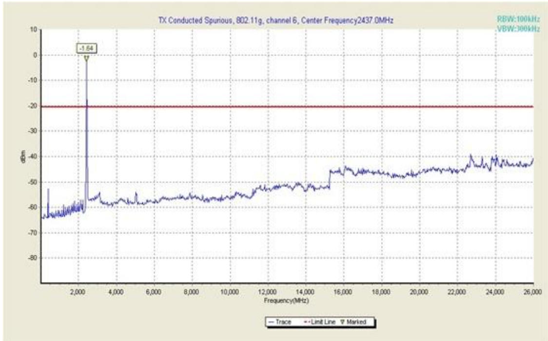
Fig. 26 Conducted Spurious Emission (802.11g, Ch6, 30 MHz-26 GHz)
