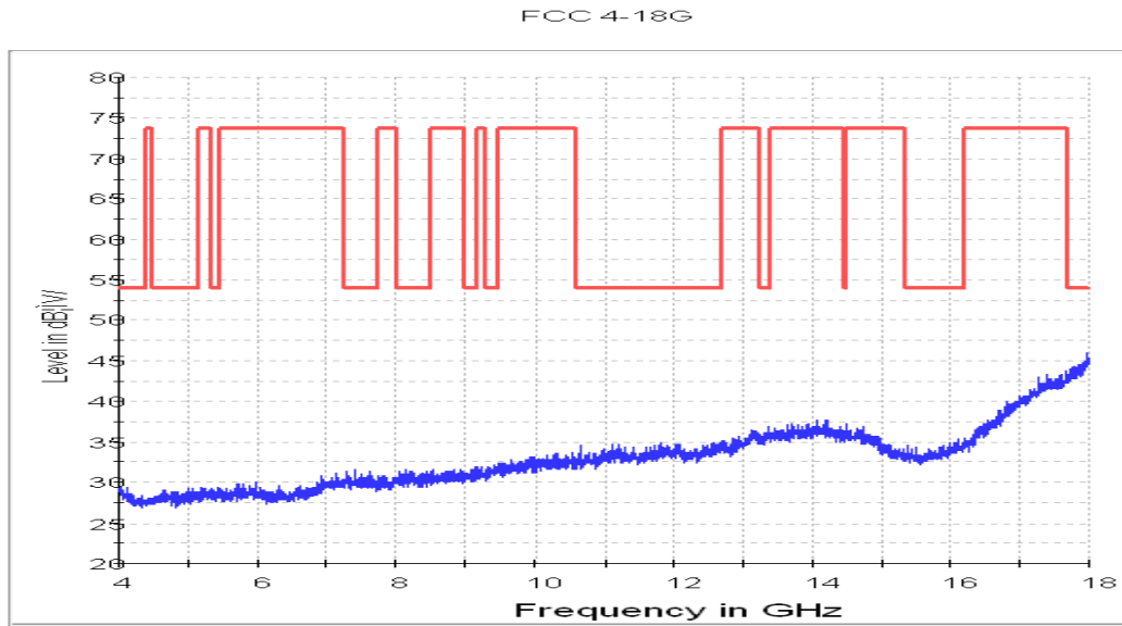
Fig. 35 Radiated Spurious Emission (802.11b, Ch6, 4 GHz-18 GHz)
