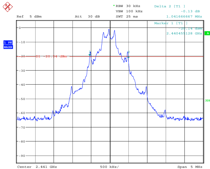
Fig.132. Occupied Bandwidth 20dB IC Ref: GFSK, Channel 39
