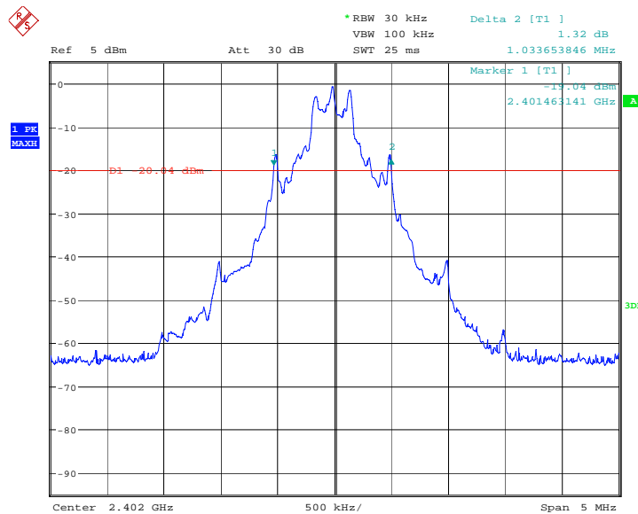
Fig.130. Occupied Bandwidth 20dB IC Ref: GFSK, Channel 0
