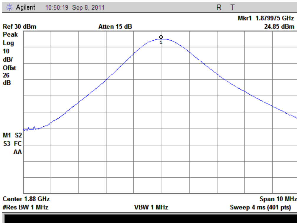
(Plot N 2: EGPRS 1900MHz Channel = 661)
