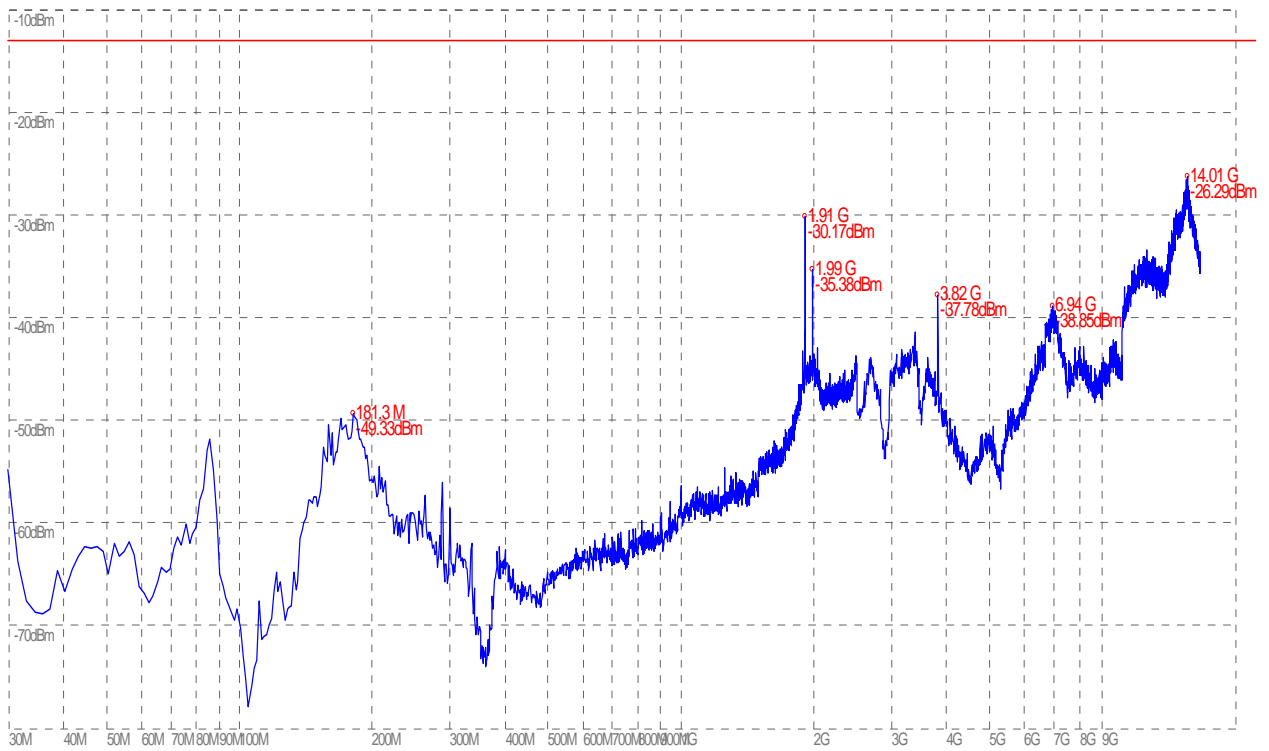
(Plot F.6: WCDMA 1900MHz Channel = 9938, Test Antenna Vertical)
