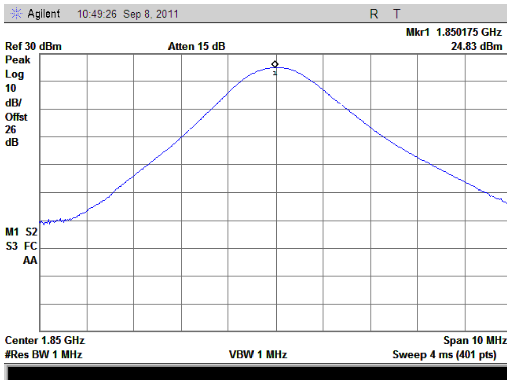
(Plot N 1: EGPRS 1900MHz Channel = 512)
