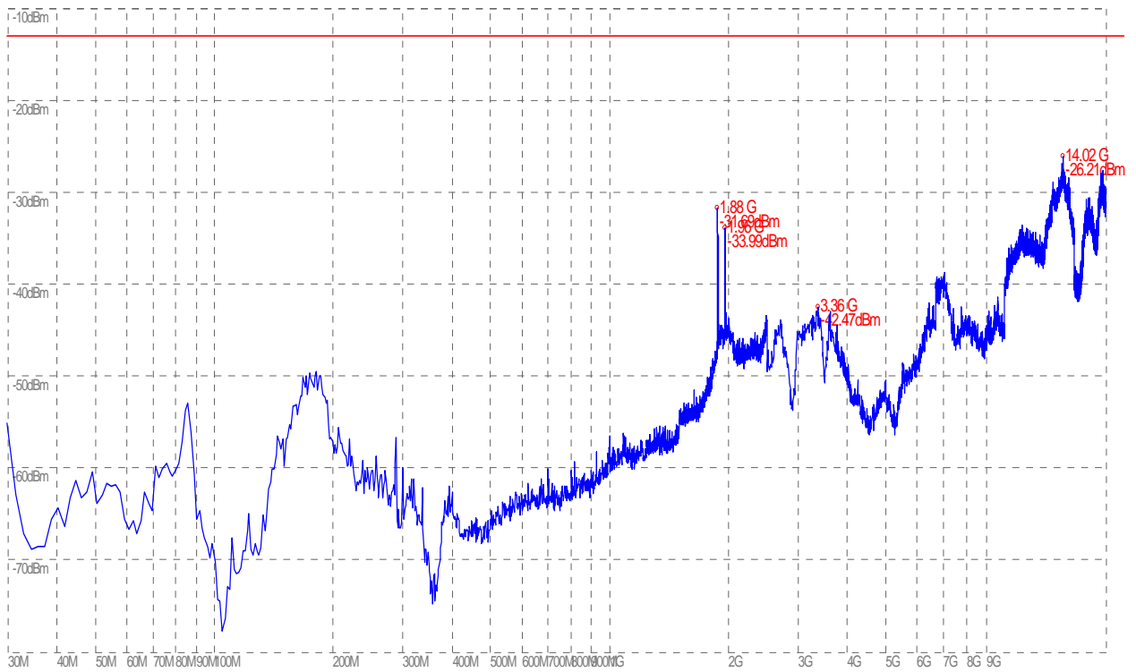
(Plot L.4: HSPA+ 1900 MHz Channel = 9800, Test Antenna V ertical)
