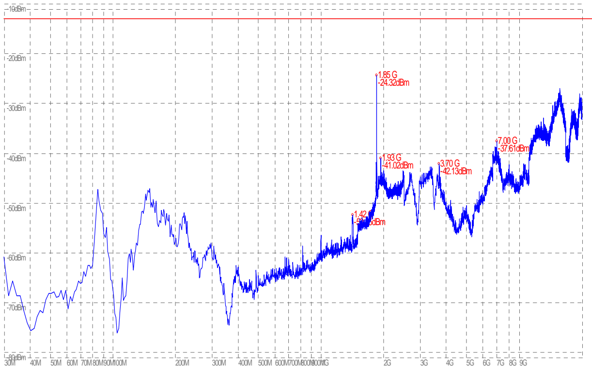
(Plot F.1: WCDMA 1900MHz Channel = 9662, Test Antenna Horizontal)
