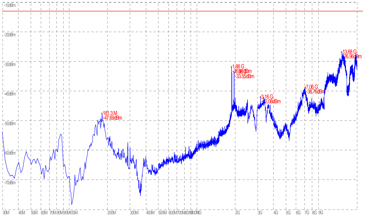
(Plot F.4: WCDMA 1900MHz Channel = 9800, Test Antenna Vertical)
