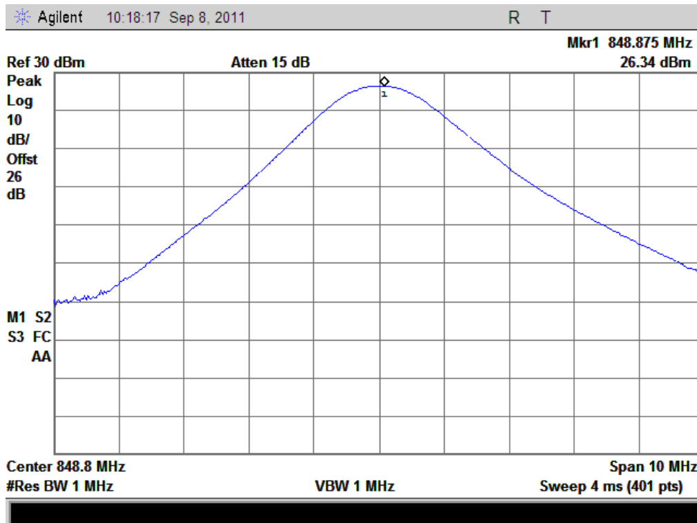
(Plot M 3: EGPRS 850MHz Channel = 251)
