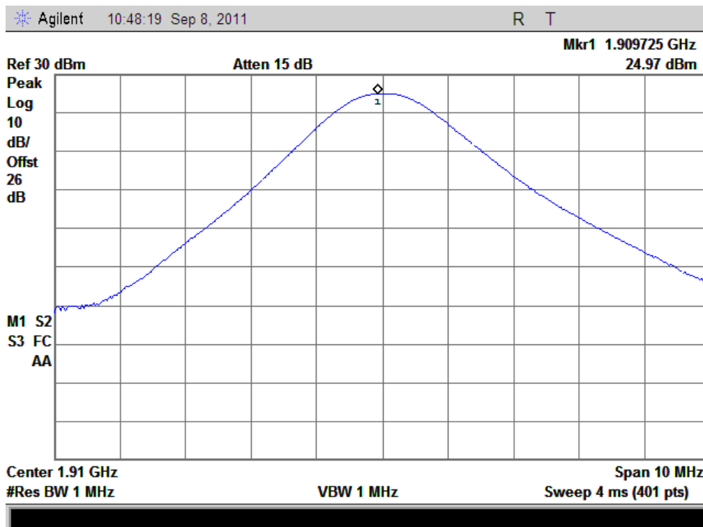
(Plot N 3: EGPRS 1900MHz Channel = 810)
