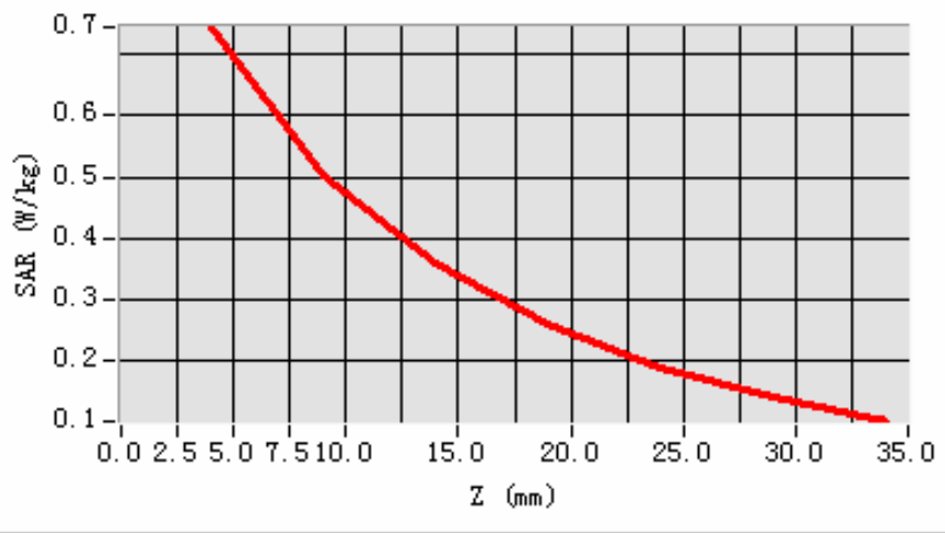
SAR, Z Axis Scan (X = 3, Y = -11)
