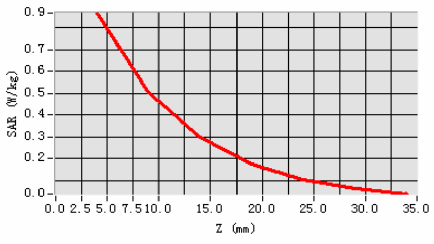
SAR, Z Axis Scan (X = -2, Y = -36)
