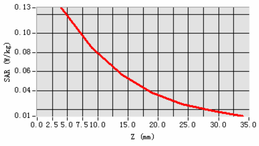
SAR, Z Axis Scan (X = 7, Y = 23)
