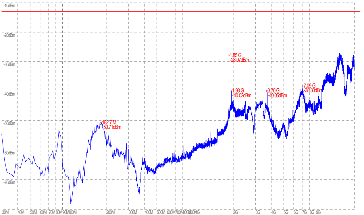
(Plot J.2: HSUPA 1900 MHz Channel = 9662, Test Antenna Vertical)
