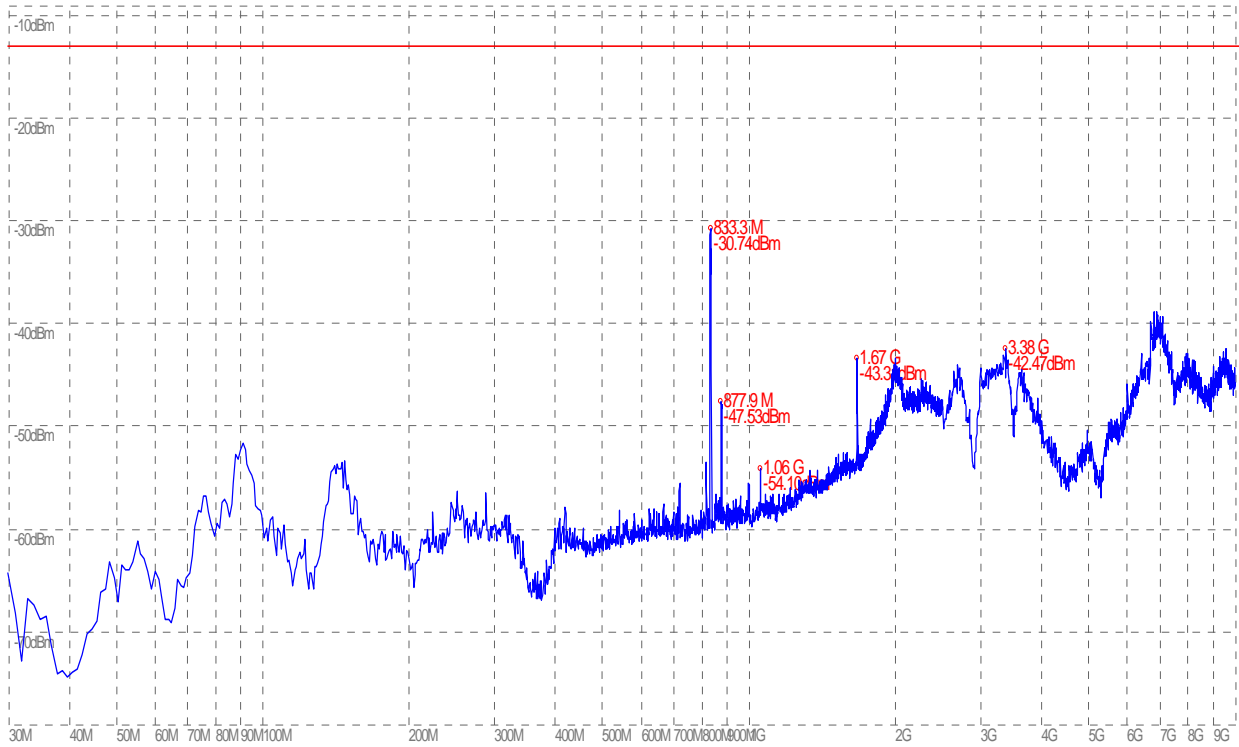
(Plot K.3: HSPA+ 850 MHz Channel = 4400, Test Antenna Horizontal)
