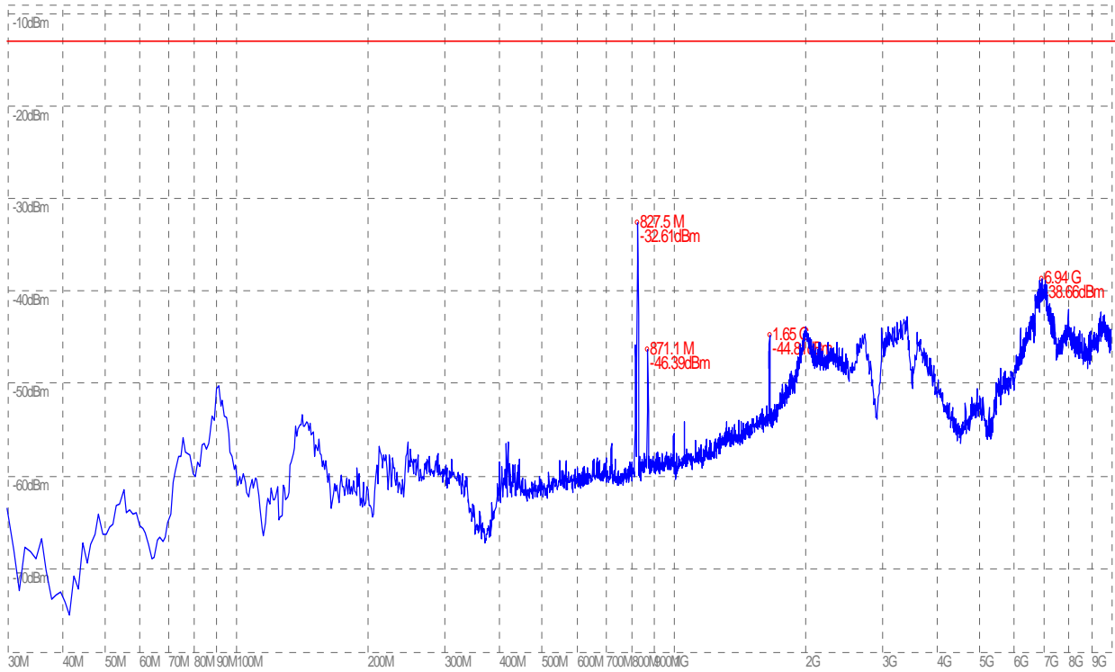
(Plot K.1: HSPA+ 850 MHz Channel = 4357, Test Antenna Horizontal)
