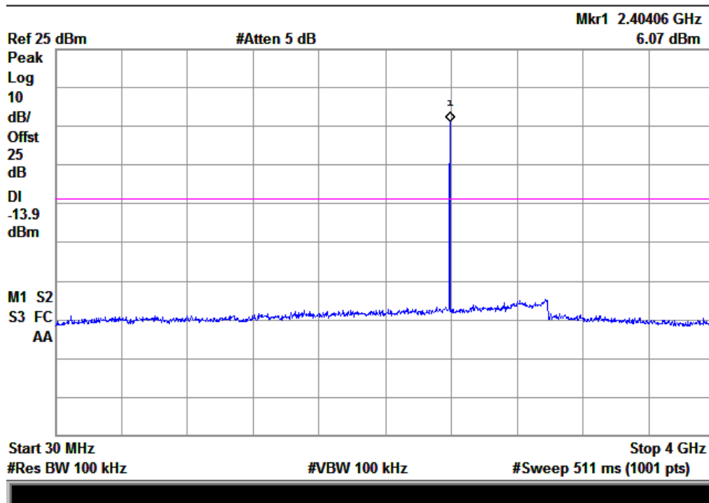
(Plot D.1: Channel = 0, 30MHz to 4GHz)
