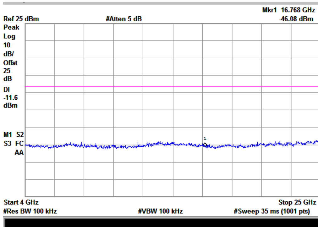
(Plot H.2: Channel = 39, 4GHz to 25GHz)
