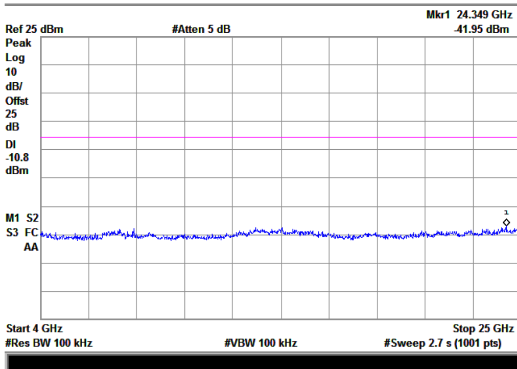
(Plot B.2: Channel = 39, 4GHz to 25GHz)
