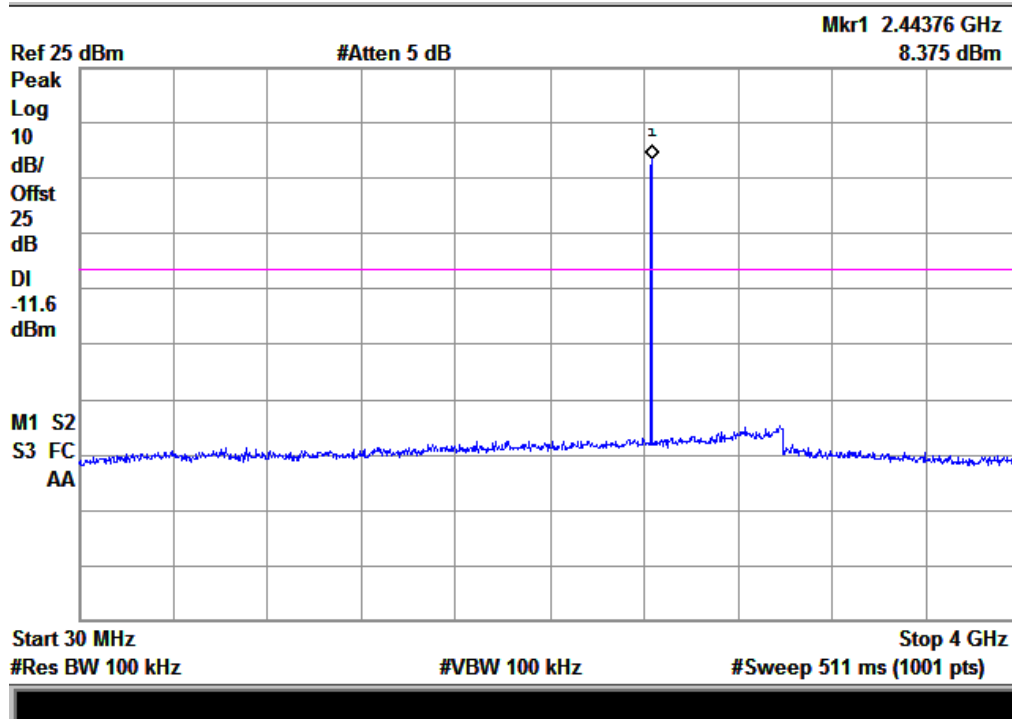
(Plot H.1: Channel = 39, 30MHz to 4GHz)
