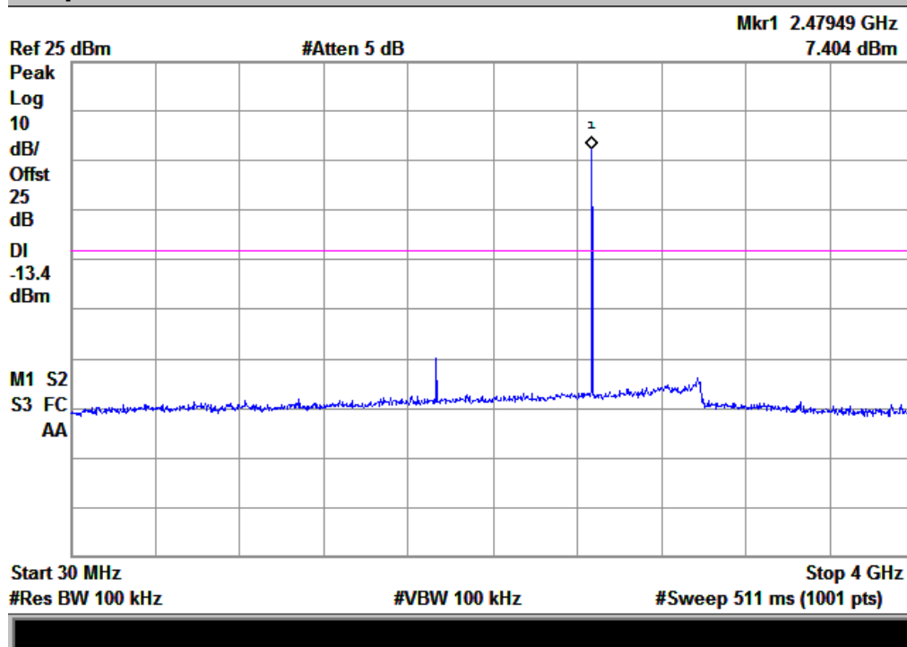
(Plot I.1: Channel = 78, 30MHz to 4GHz)
