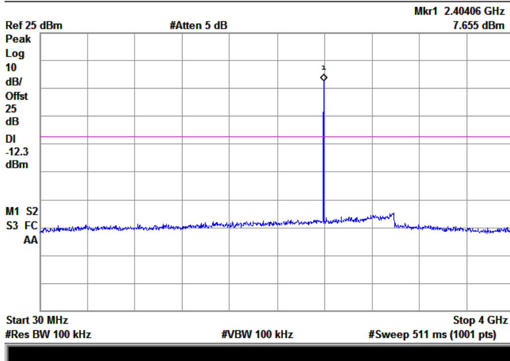
(Plot G.1: Channel = 0, 30MHz to 4GHz)
