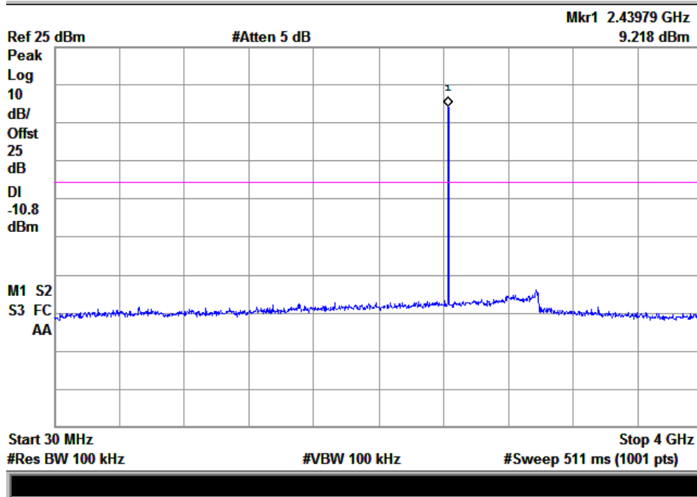
(Plot B.1: Channel = 39, 30MHz to 4GHz)
