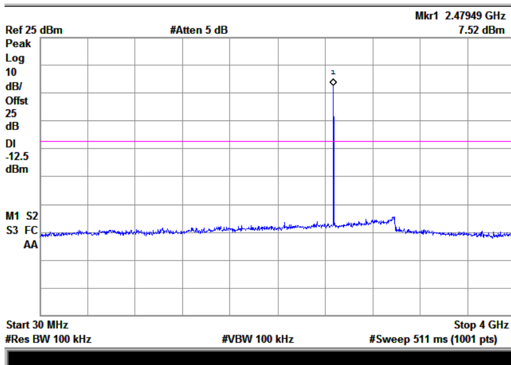
(Plot F.1: Channel = 78, 30MHz to 4GHz)
