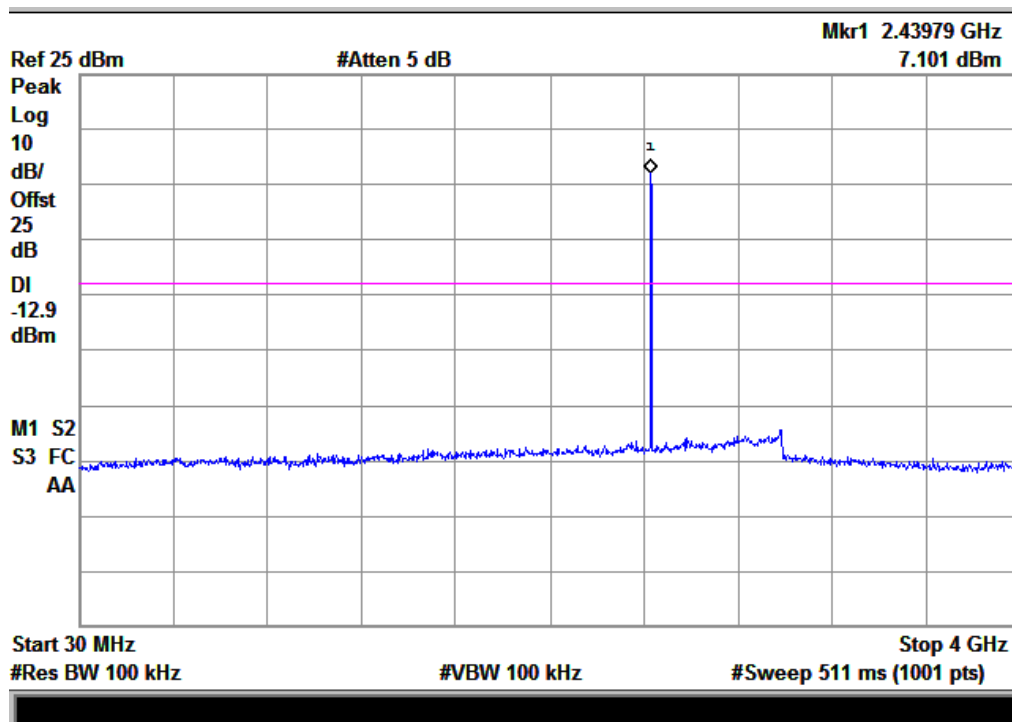
(Plot E.1: Channel = 39, 30MHz to 4GHz)
