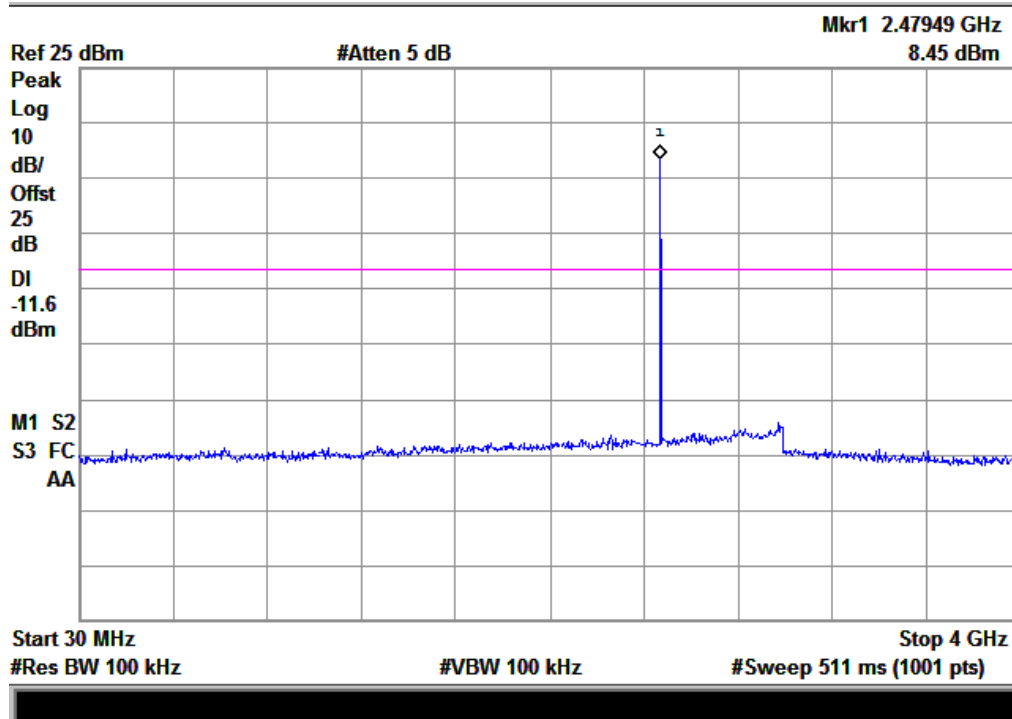
(Plot C.1: Channel = 78, 30MHz to 4GHz)
