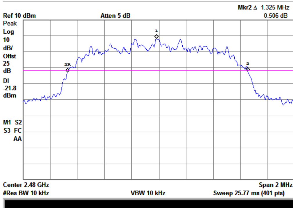
(Plot F: Channel = 2480)
