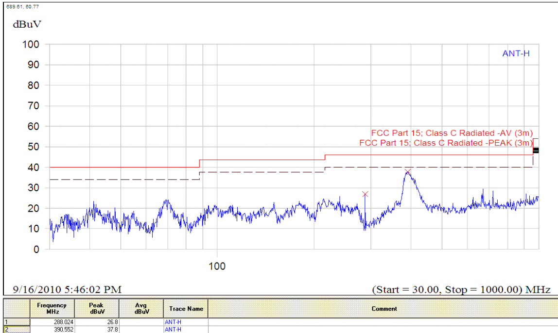
(Plot A.2: Antenna Horizontal, 30MHz to 1GHz)
