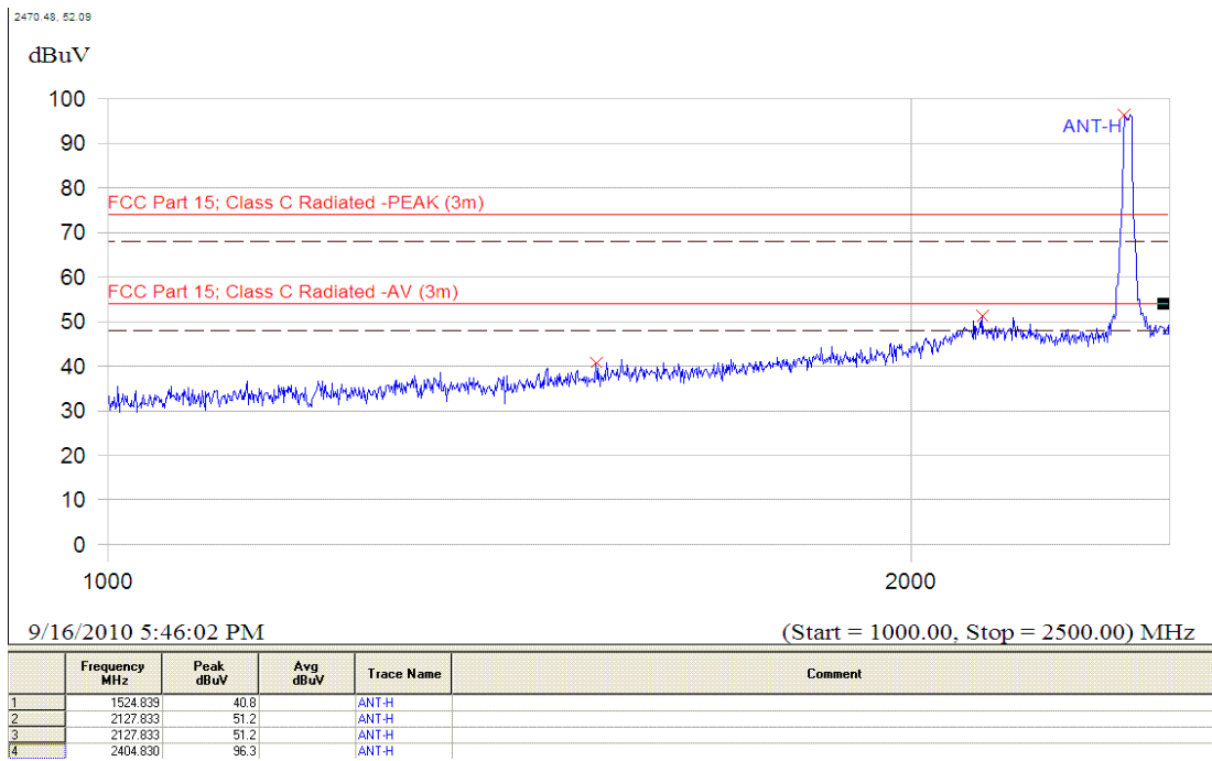
(Plot A.3: Antenna Horizontal, 1GHz to 2.5GHz)
