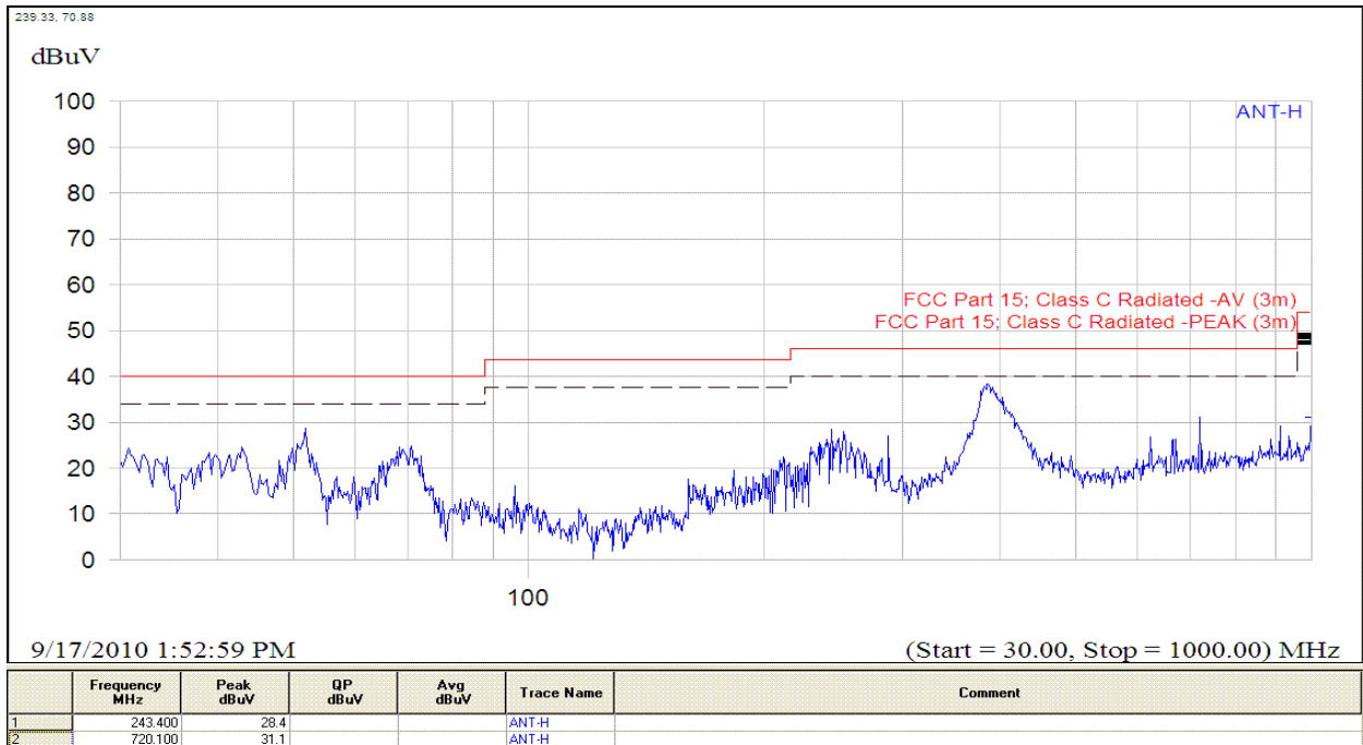
(Plot A.2: Antenna Horizontal, 30MHz to 1GHz)
