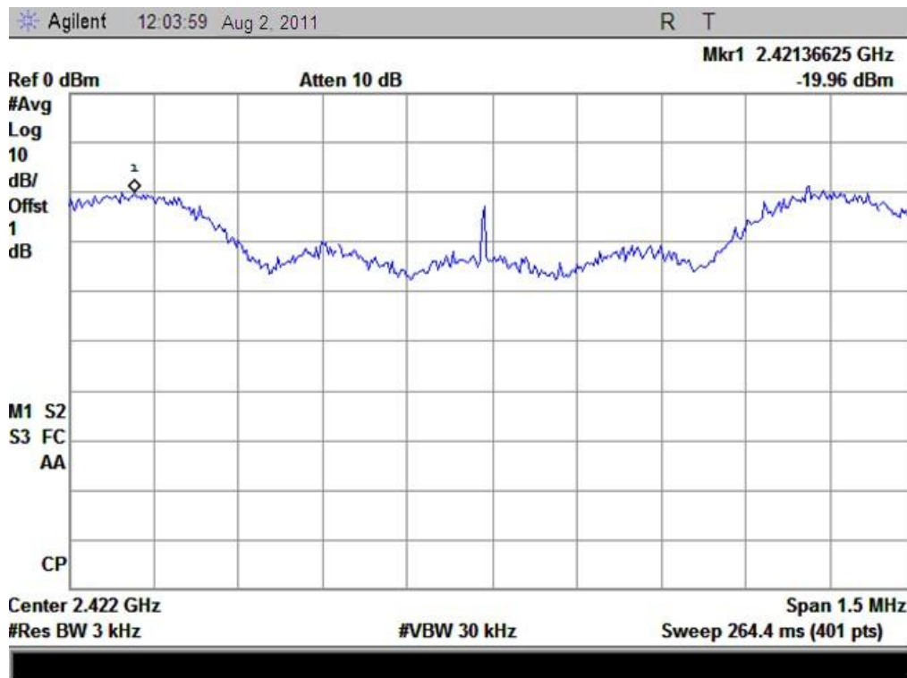
(Plot J: Channel = 3)
