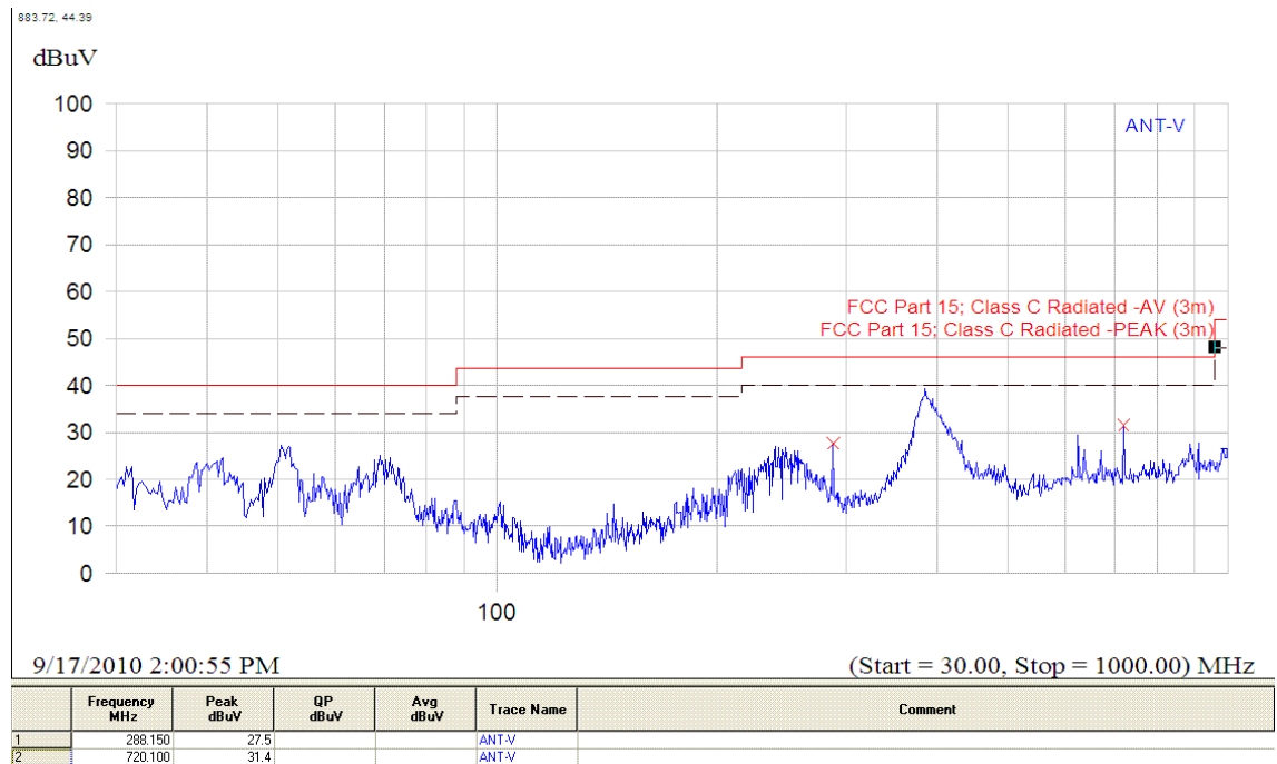
(Plot A.5: Antenna Vertical, 30MHz to 1GHz)
