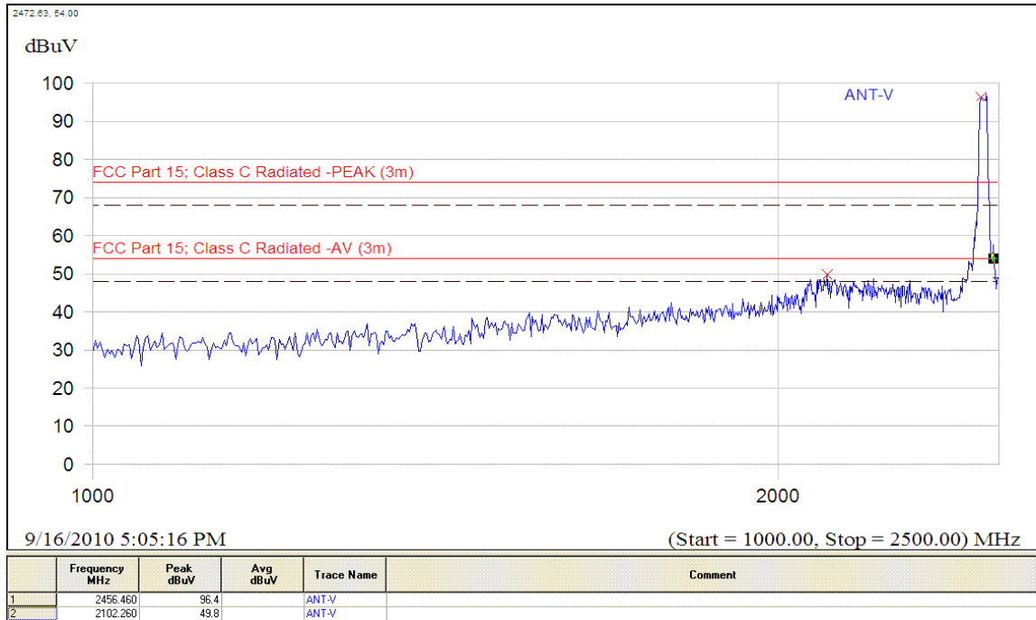
(Plot C.6: Antenna Vertical, 1GHz to 2.5GHz)
