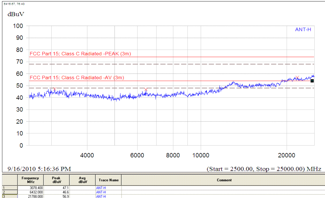
(Plot C.4: Antenna Horizontal, 2.5GHz to 25GHz)
