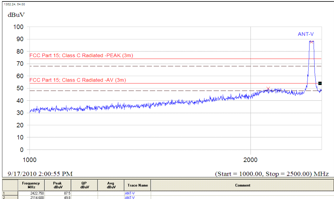
(Plot A.6: Antenna Vertical, 1GHz to 2.5GHz)
