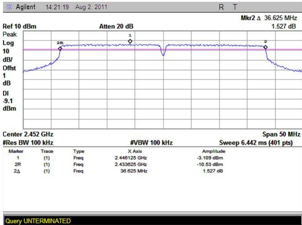
(Plot C: Channel 9: 2452MHz)
