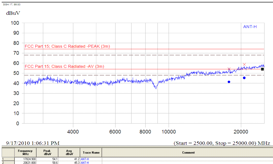
(Plot B.4: Antenna Horizontal, 2.5GHz to 25GHz)
