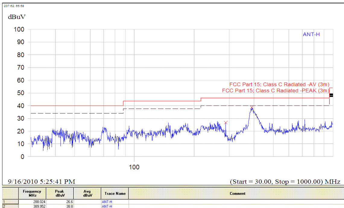
(Plot B.2: Antenna Horizontal, 30MHz to 1GHz)
