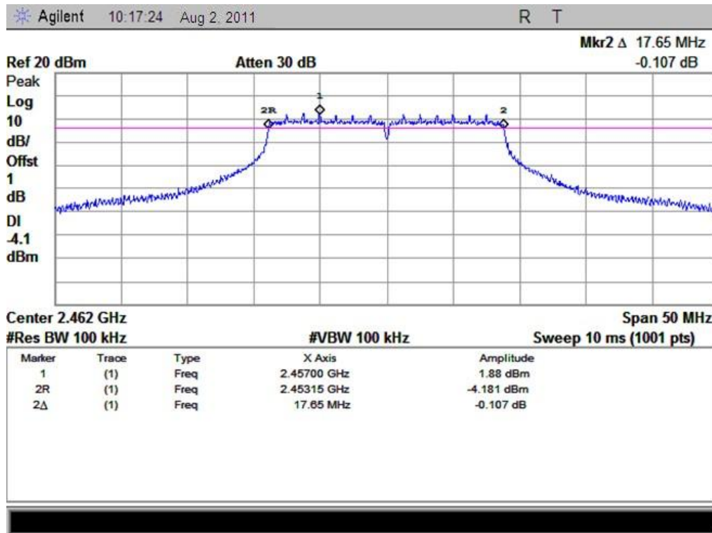
(Plot C: Channel 11: 2462MHz)
