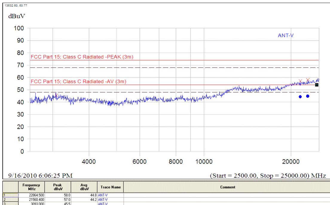
(Plot A.7: Antenna Vertical, 2.5GHz to 25GHz)
