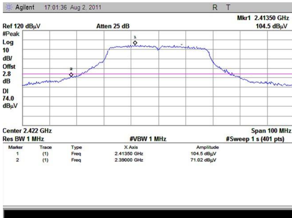
(Plot A1: Channel = 3 PEAK)
