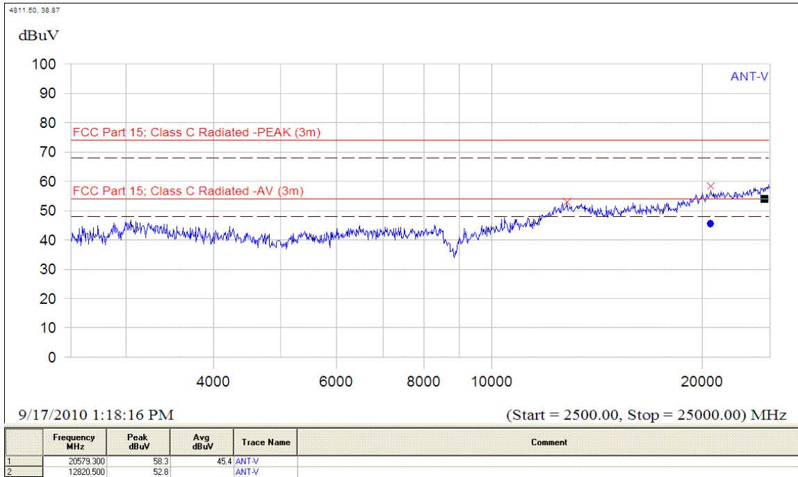
(Plot B.7: Antenna Vertical, 2.5GHz to 25GHz)
