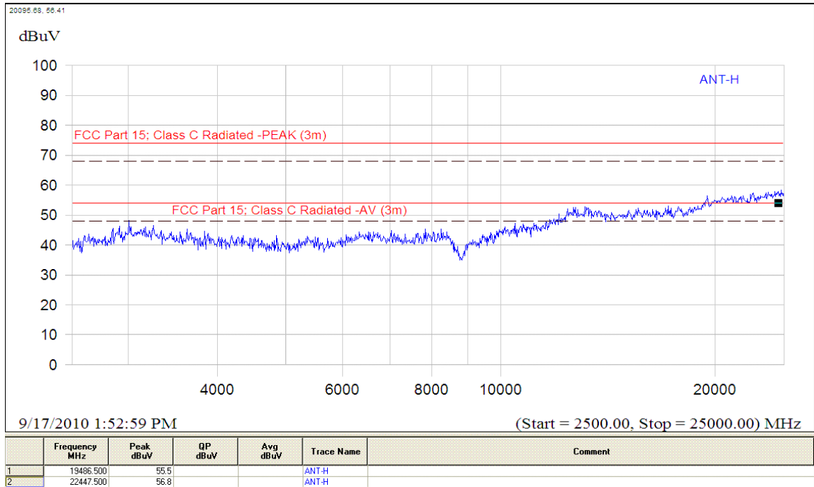
(Plot A.4: Antenna Horizontal, 2.5GHz to 25GHz)
