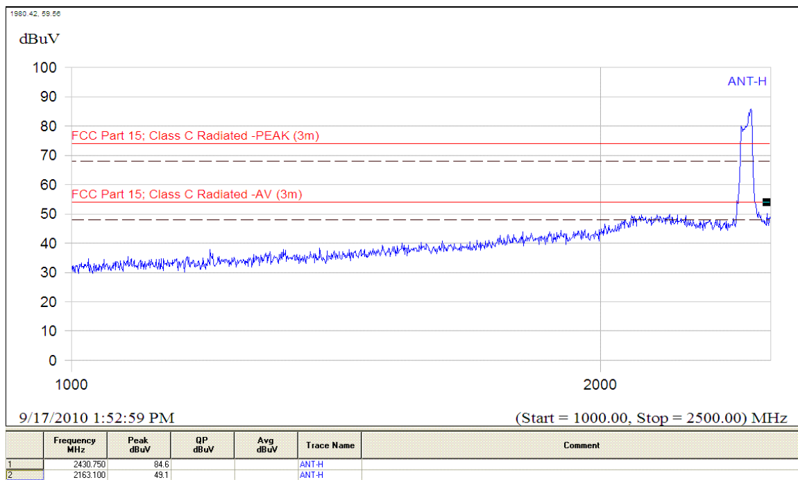
(Plot A.3: Antenna Horizontal, 1GHz to 2.5GHz)
