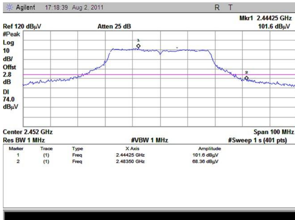
(Plot B1: Channel = 9 PEAK)
