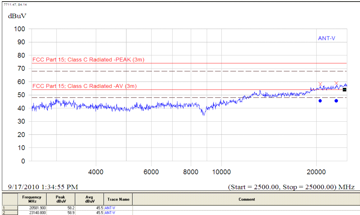
(Plot C.7: Antenna Vertical, 2.5GHz to 25GHz)
