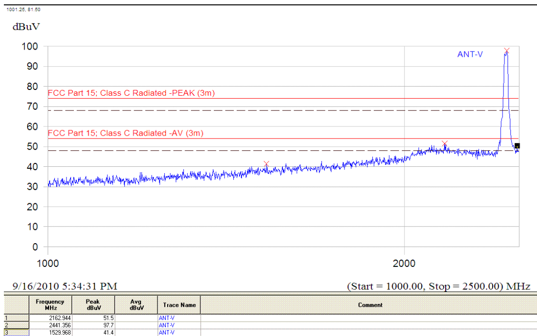
(Plot B.6: Antenna Vertical, 1GHz to 2.5GHz)
