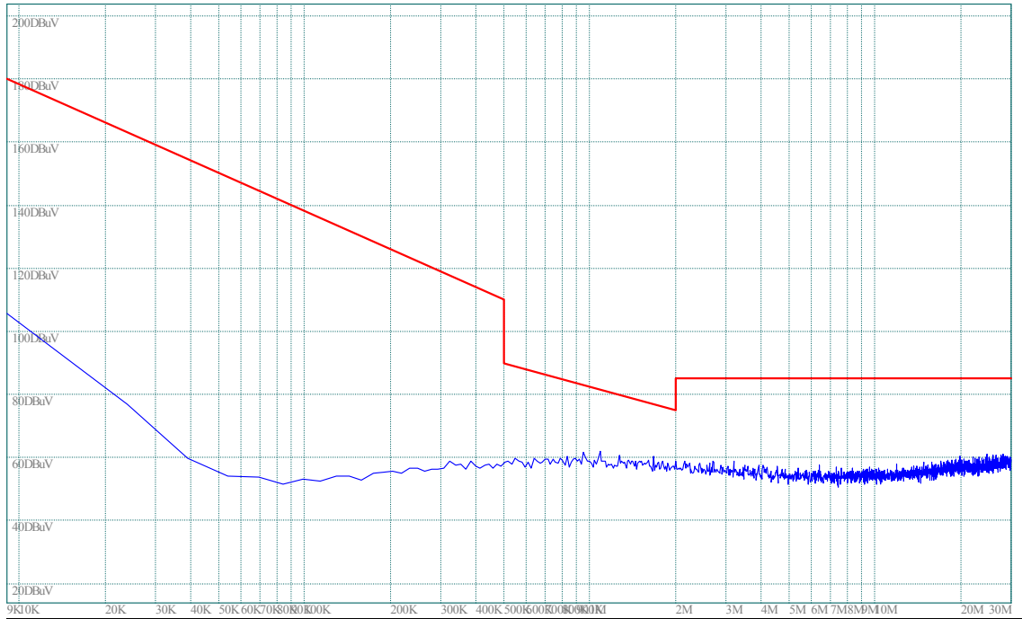
(Plot B.1: 9kHz to 30MHz)
