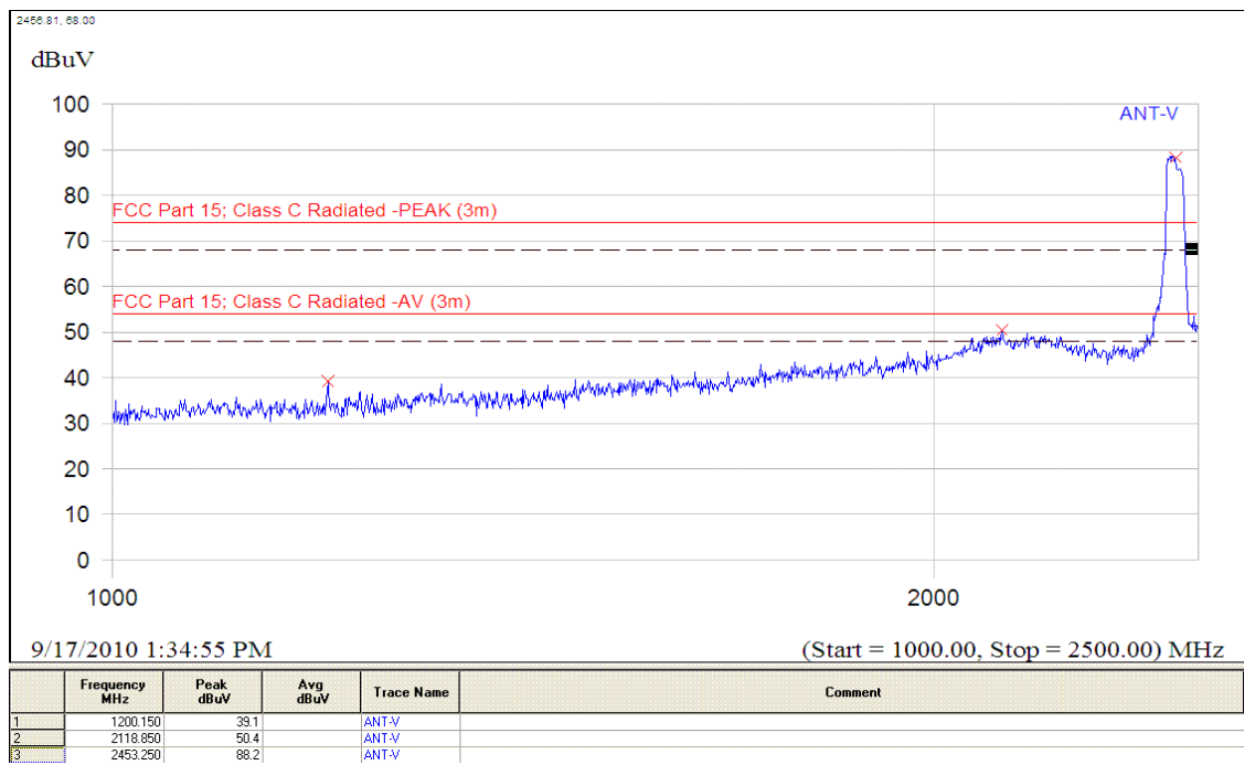
(Plot C.6: Antenna Vertical, 1GHz to 2.5GHz)
