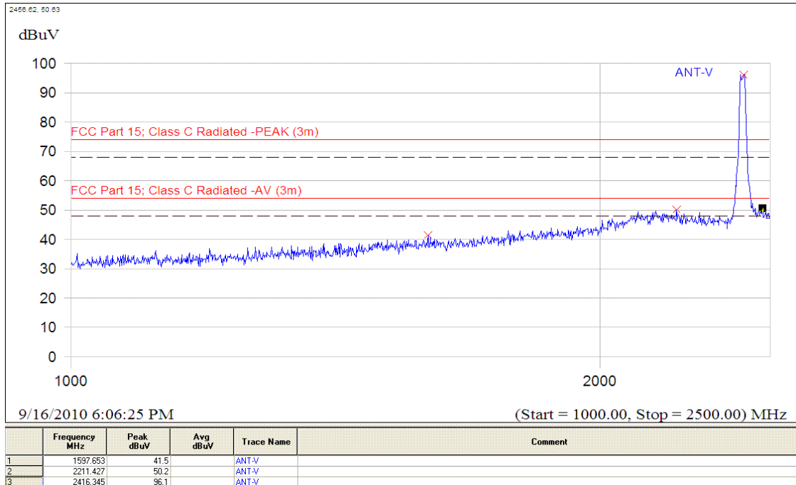
(Plot A.6: Antenna Vertical, 1GHz to 2.5GHz)
