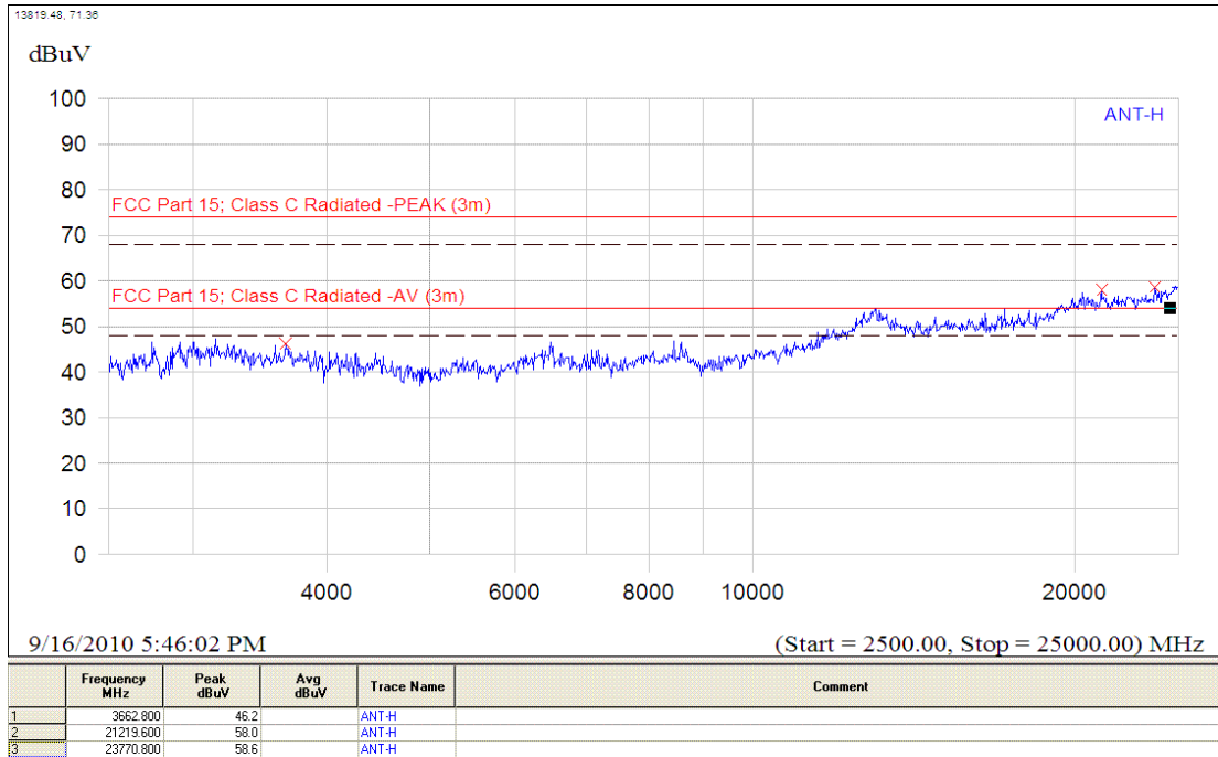
(Plot A.4: Antenna Horizontal, 2.5GHz to 25GHz)
