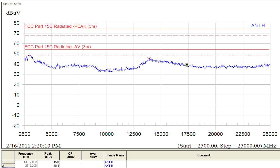
(Plot C.4: Antenna Horizontal, 2.5GHz to 25GHz)
