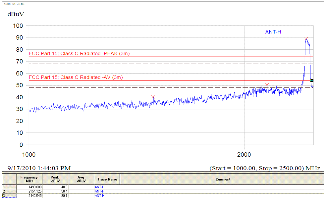
(Plot C.3: Antenna Horizontal, 1GHz to 2.5GHz)
