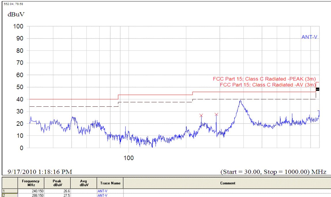
(Plot B.5: Antenna Vertical, 30MHz to 1GHz)
