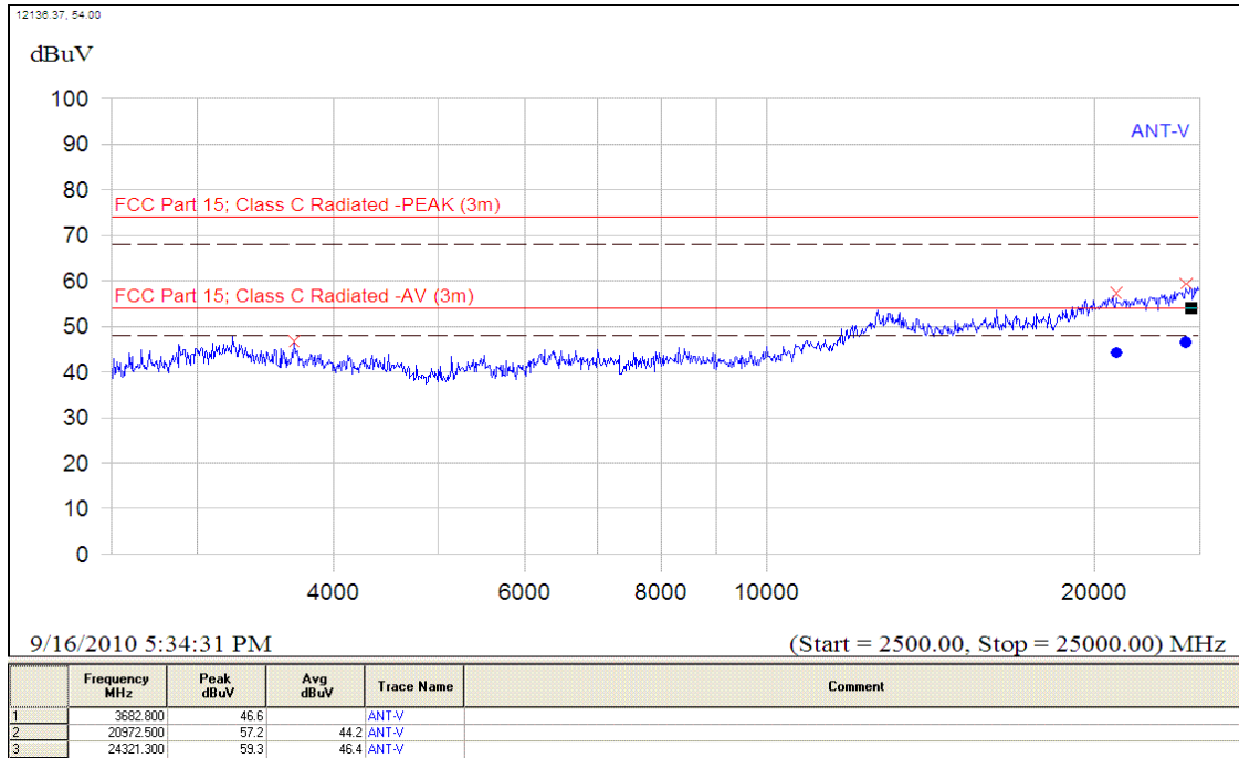
(Plot B.7: Antenna Vertical, 2.5GHz to 25GHz)
