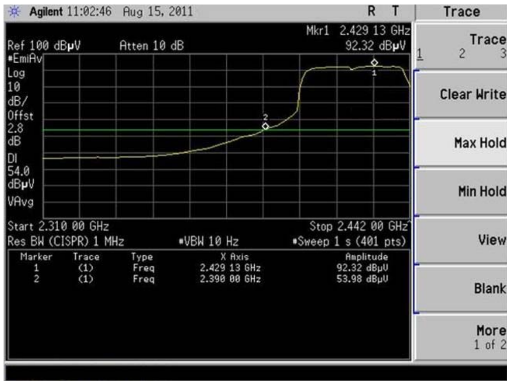
(Plot A2: Channel = 3 AVG)
