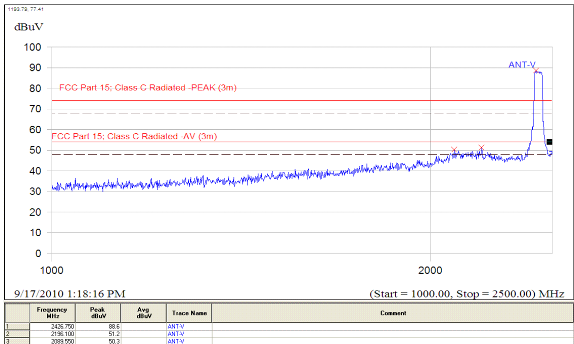
(Plot B.6: Antenna Vertical, 1GHz to 2.5GHz)
