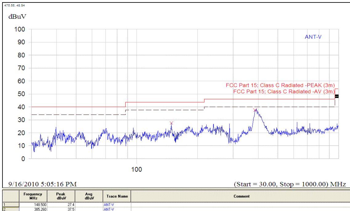
(Plot C.5: Antenna Vertical, 30MHz to 1GHz)
