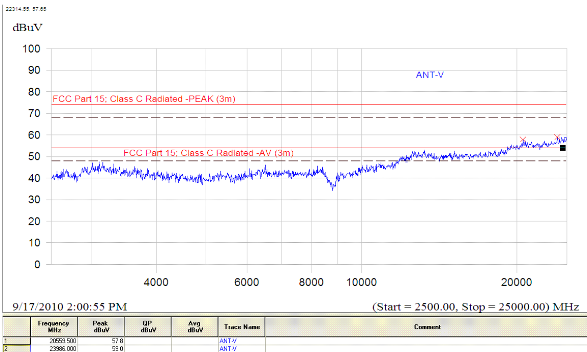
(Plot A.7: Antenna Vertical, 2.5GHz to 25GHz)
