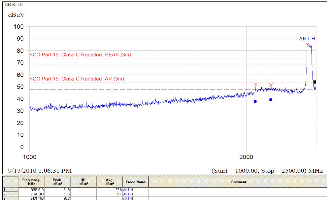
(Plot B.3: Antenna Horizontal, 1GHz to 2.5GHz)
