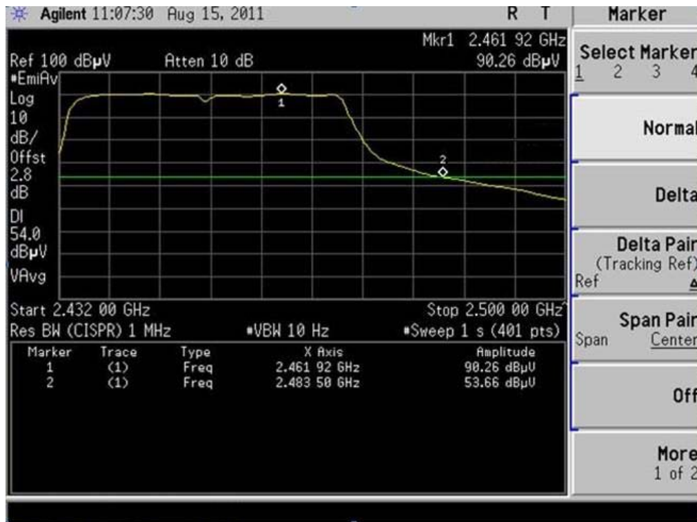
(Plot B2: Channel = 9 AVG)
