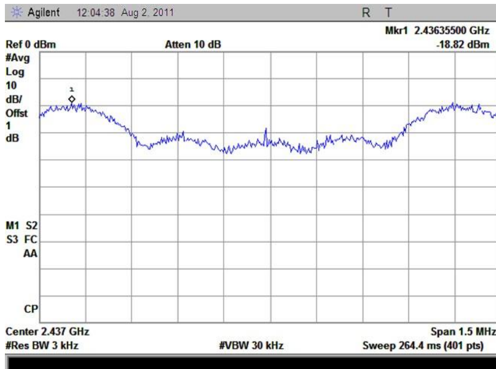
(Plot K: Channel = 6)
