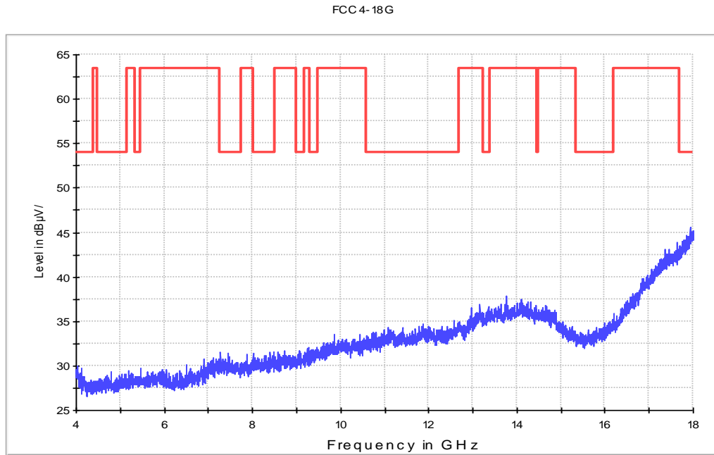
Fig.72. Radiated emission: \pi/4 DQPSK, Channel 0, 4 GHz - 18 GHz
