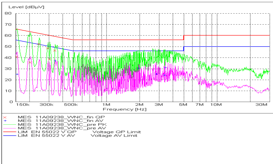
Fig. 77 AC Powerline Conducted Emission-802.11n
