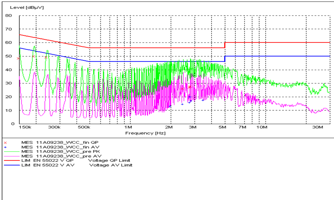
Fig. 78 AC Powerline Conducted Emission-IDLE
