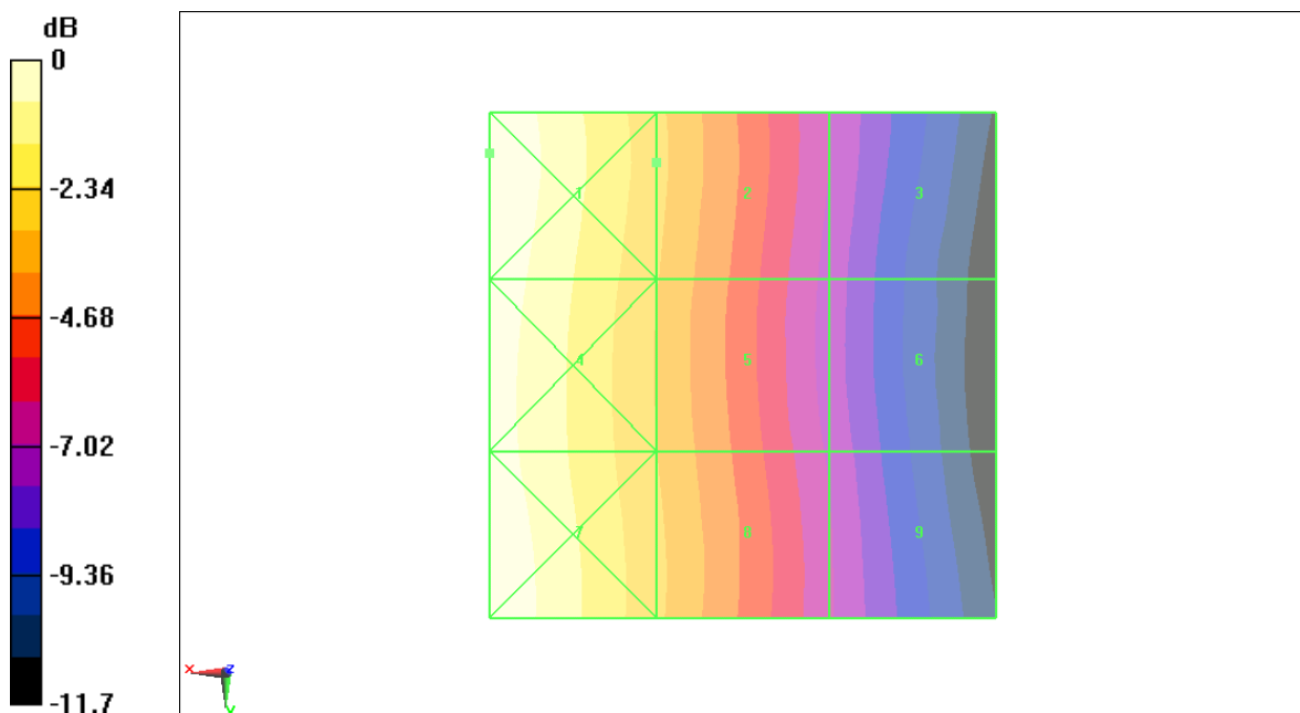
Fig B.20 HAC RF H-Field WCDMA 850 Middle
