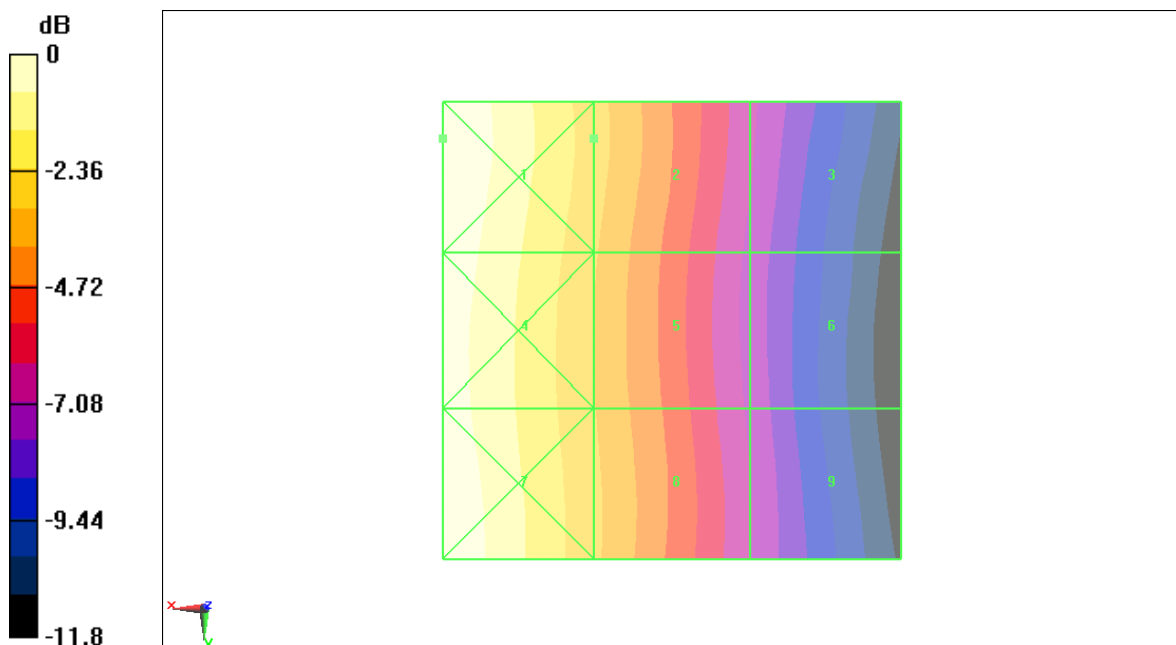
Fig B.19 HAC RF H-Field WCDMA 850 High
