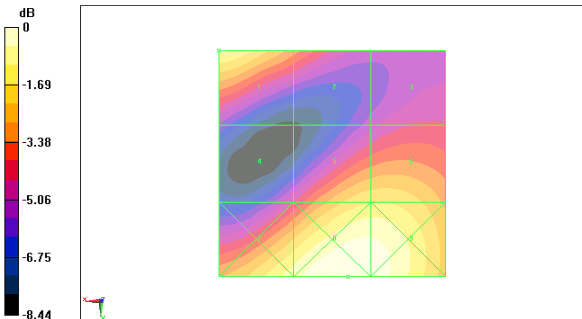
Fig B.12 HAC RF E-Field WCDMA 1900 Low
