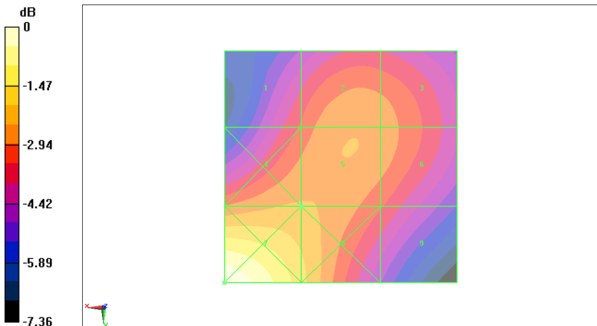
Fig B.22 HAC RF H-Field WCDMA 1900 High
