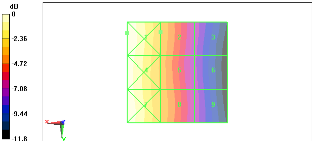
Fig B.15 HAC RF H-Field GSM 850 Low
