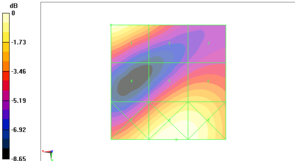
Fig B.11 HAC RF E-Field WCDMA 1900 Middle
