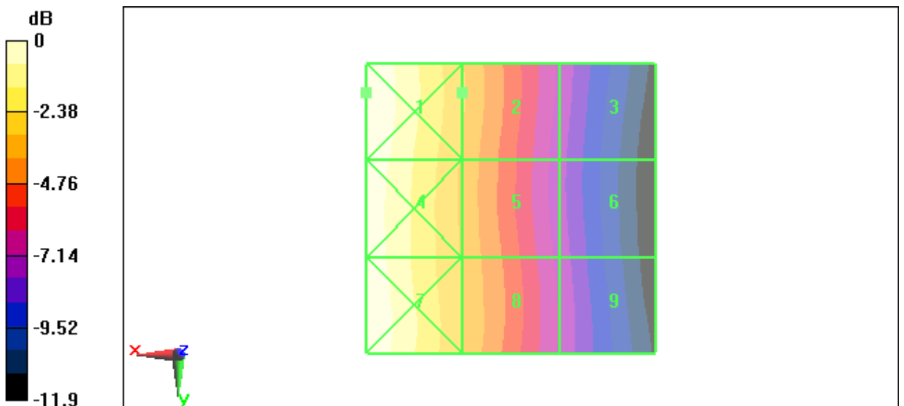
Fig B.14 HAC RF H-Field GSM 850 Middle
