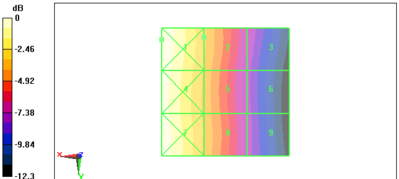
Fig B.13 HAC RF H-Field GSM 850 High
