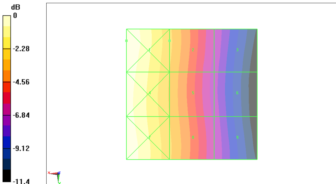
Fig B.21 HAC RF H-Field WCDMA 850 Low
