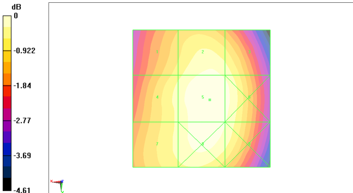
Fig B.8 HAC RF E-Field WCDMA 850 Middle
