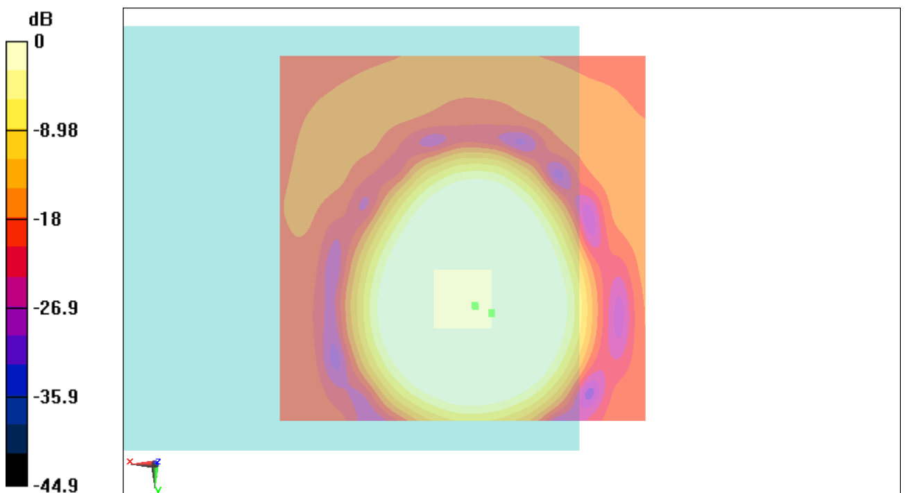
Fig B.6 T-Coil GSM 1900
