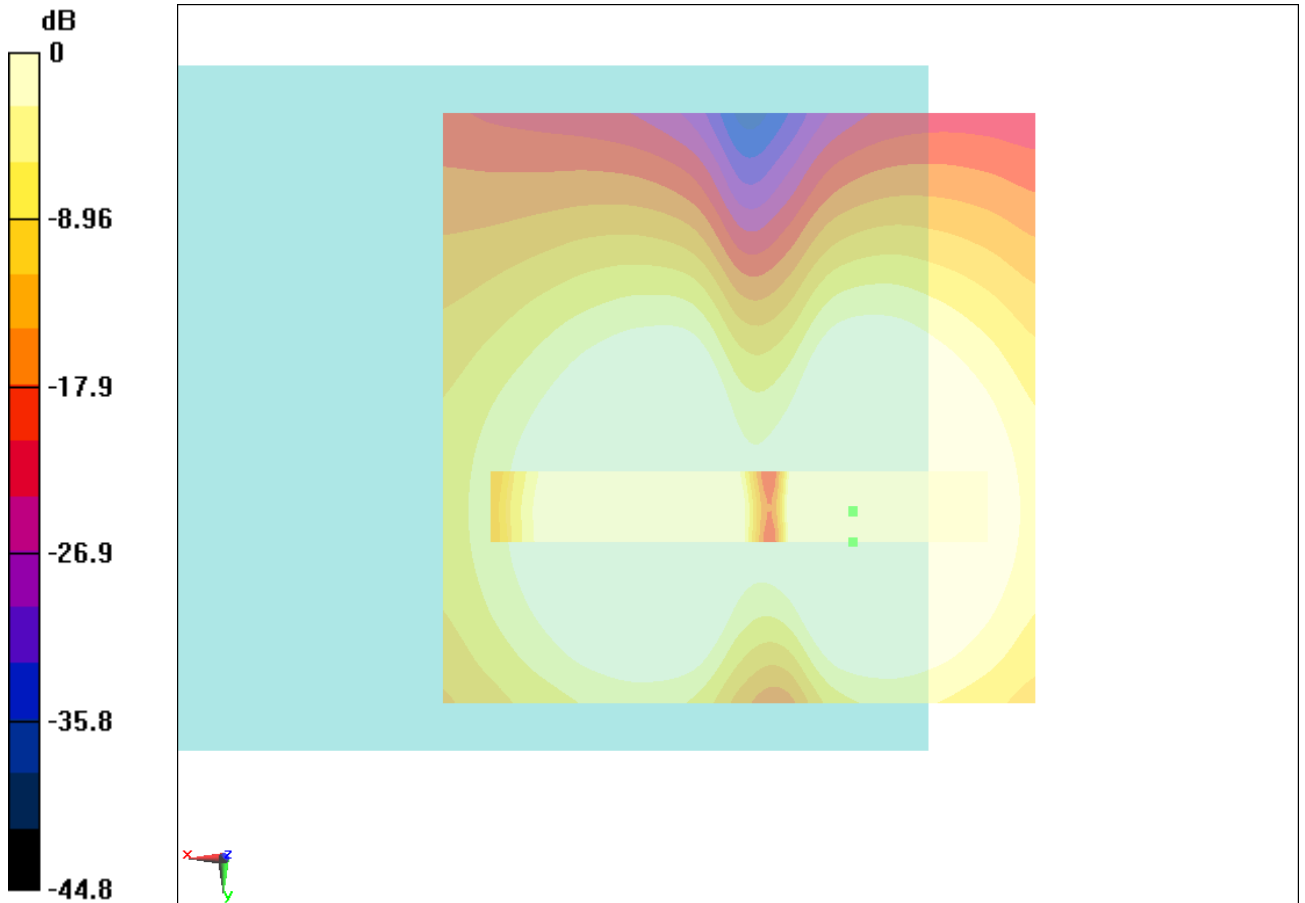
Fig B.1 T-Coil GSM 850
