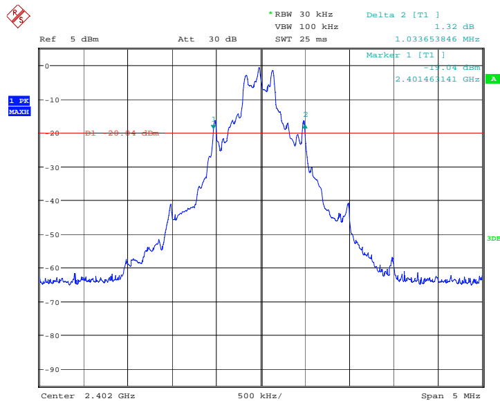
Fig.130. Occupied Bandwidth 20dB IC Ref: GFSK, Channel 0
