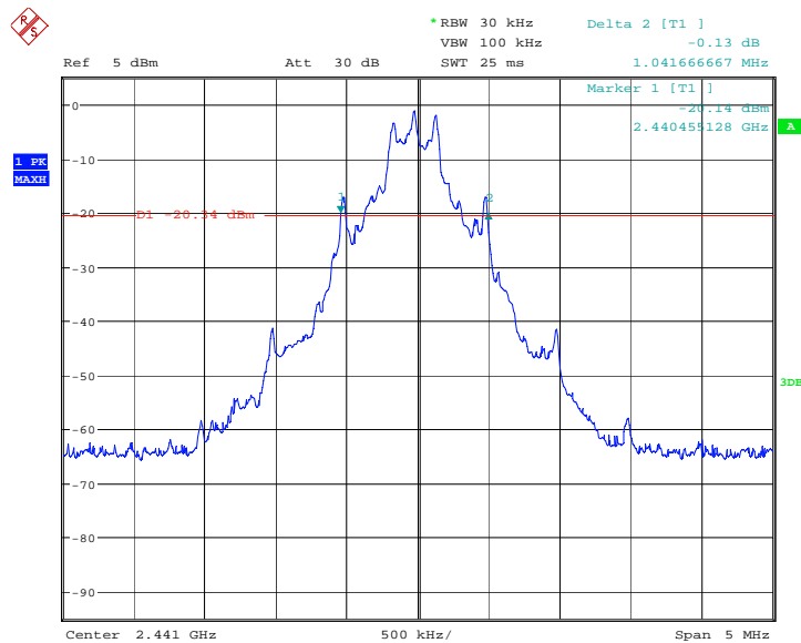
Fig.132. Occupied Bandwidth 20dB IC Ref: GFSK, Channel 39
