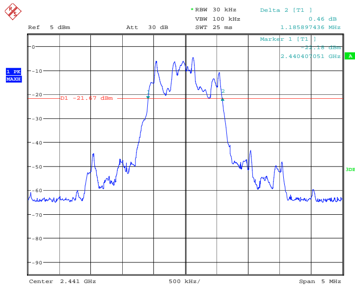
Fig.144. Occupied Bandwidth 20dB IC Ref: 8DDPSK , Channel 39
