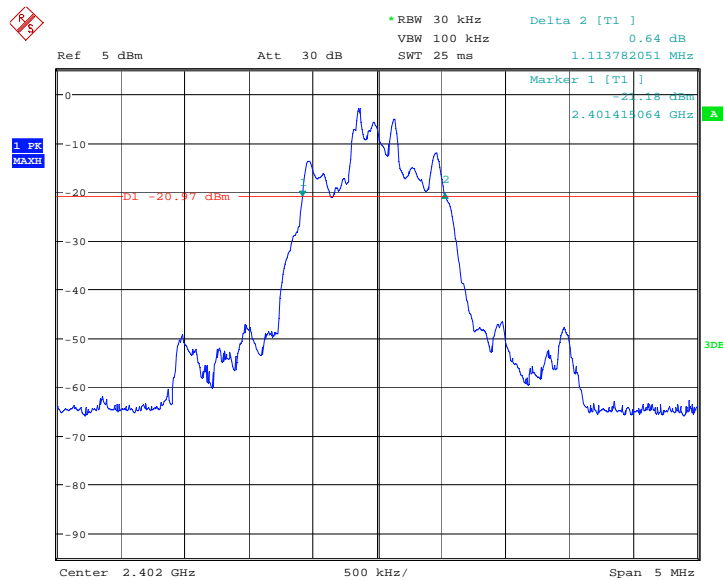
Fig.136. Occupied Bandwidth 20dB IC Ref: \pi/4 DQPSK , Channel 0
