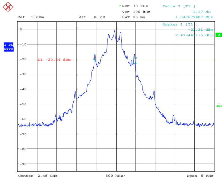
Fig.134. Occupied Bandwidth 20dB IC Ref: GFSK, Channel 78
