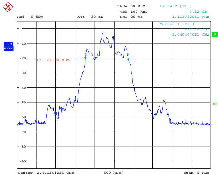
Fig.138. Occupied Bandwidth 20dB IC Ref: \pi/4 DQPSK , Channel 39
