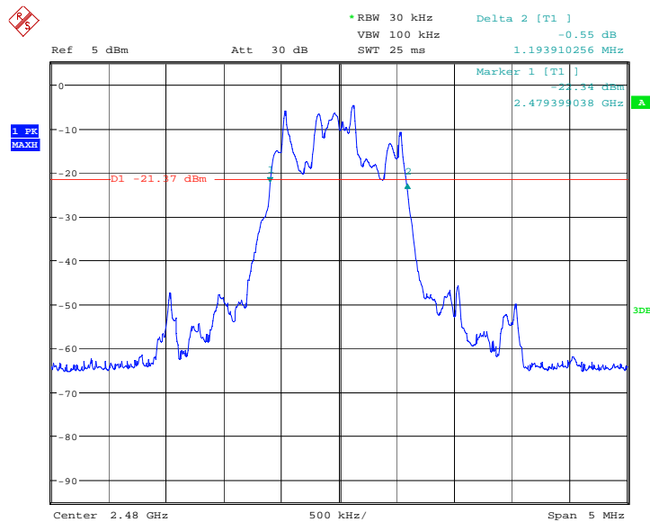
Fig.146. Occupied Bandwidth 20dB IC Ref: 8DDPSK , Channel 78
