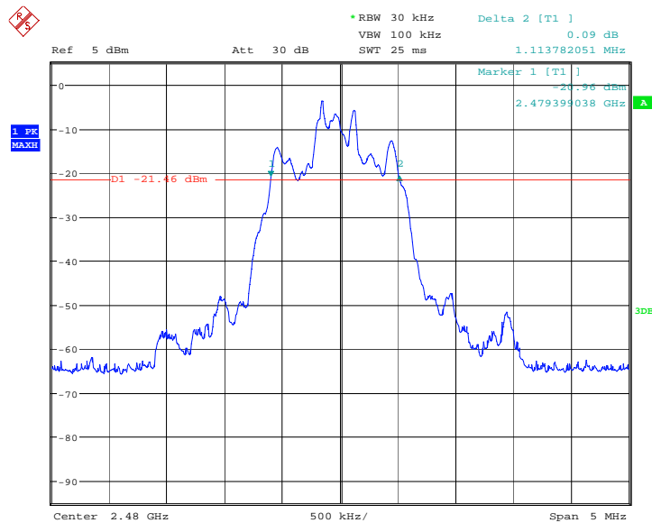
Fig.140. Occupied Bandwidth 20dB IC Ref: \pi/4 DQPSK , Channel 78
