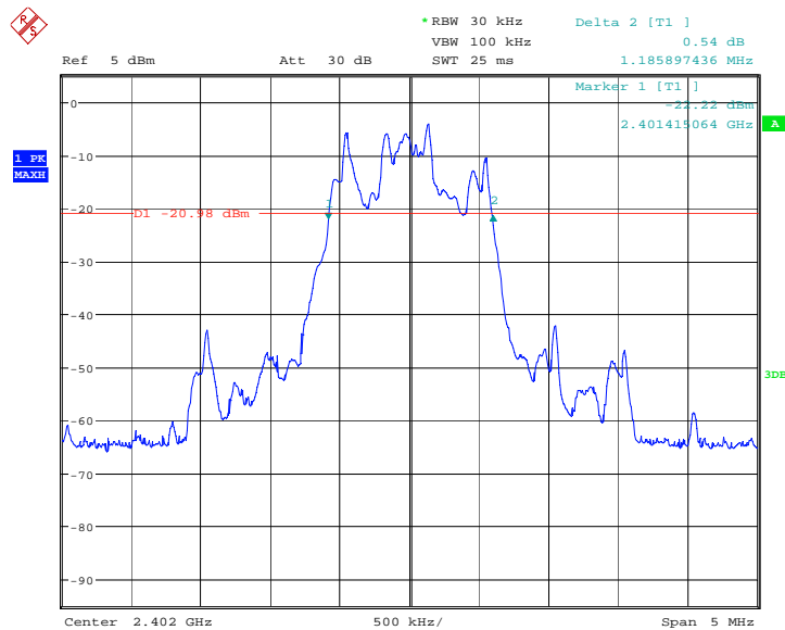
Fig.142. Occupied Bandwidth 20dB IC Ref: 8DDPSK , Channel 0
