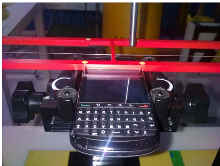
Picture 3: EUT Positioning for T-Coil
