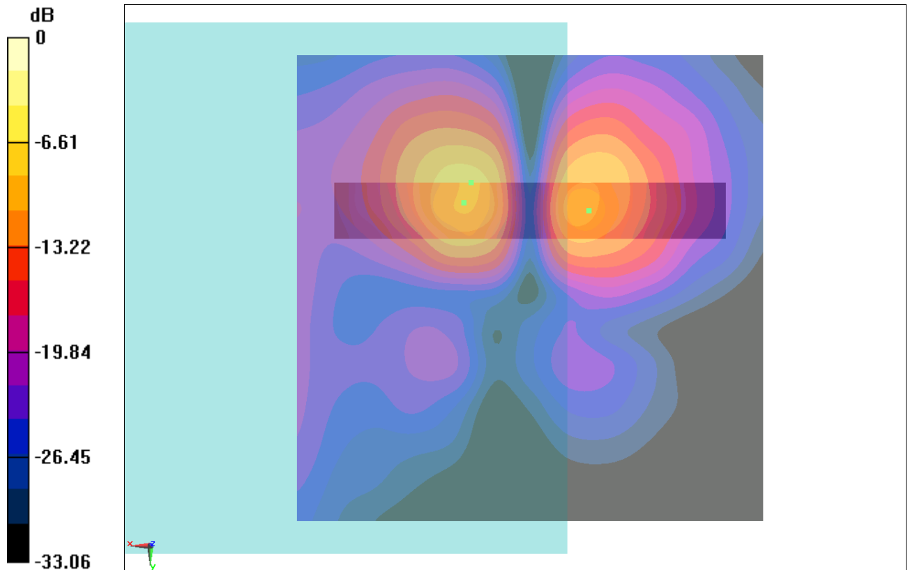
Fig B.13 T-Coil CDMA 1880_Channel 600
