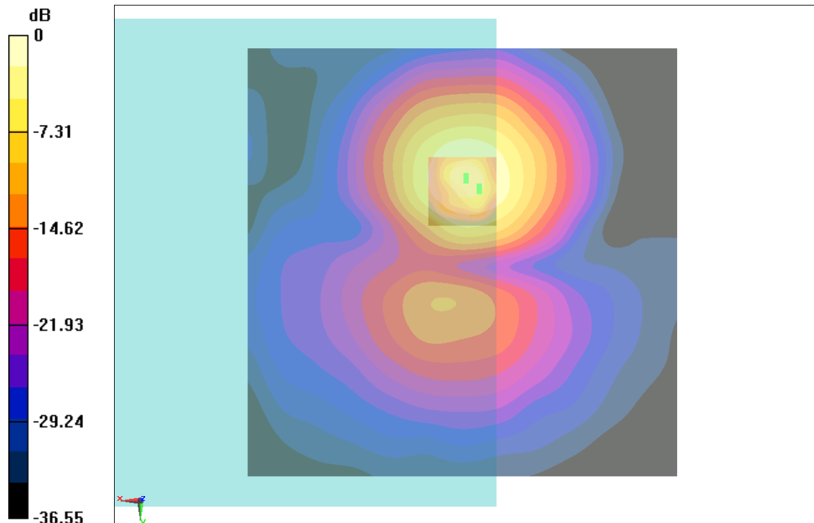
Fig B.9 T-Coil CDMA 835_Channel 1013
