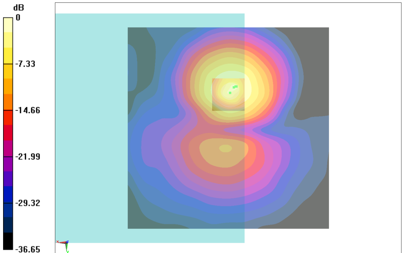
Fig B.3 T-Coil CDMA 835_Channel 777
