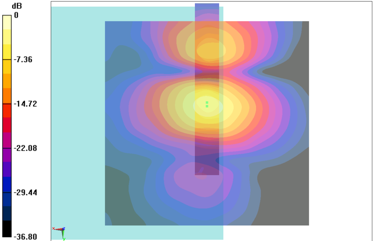
Fig B.8 T-Coil CDMA 835_Channel 1013
