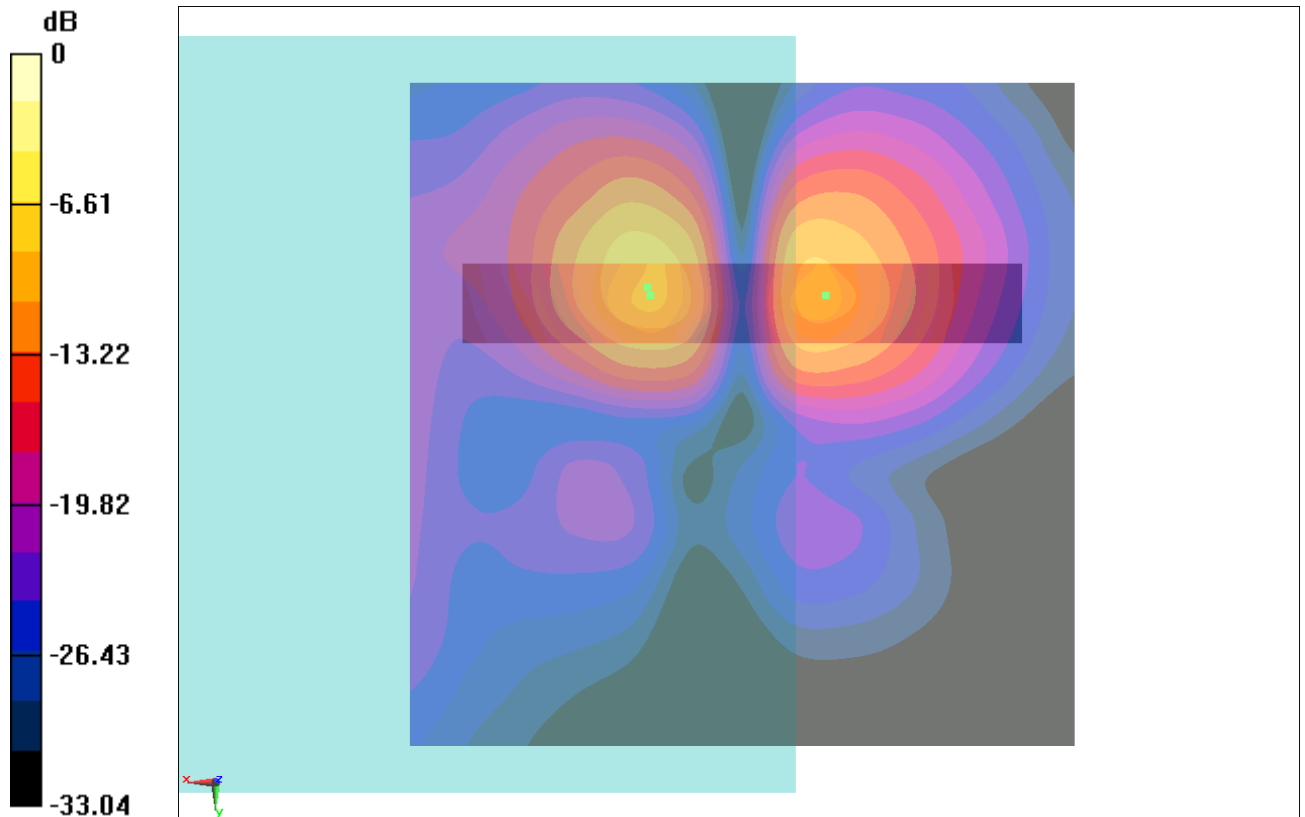
Fig B.16 T-Coil CDMA 1880_Channel 25
