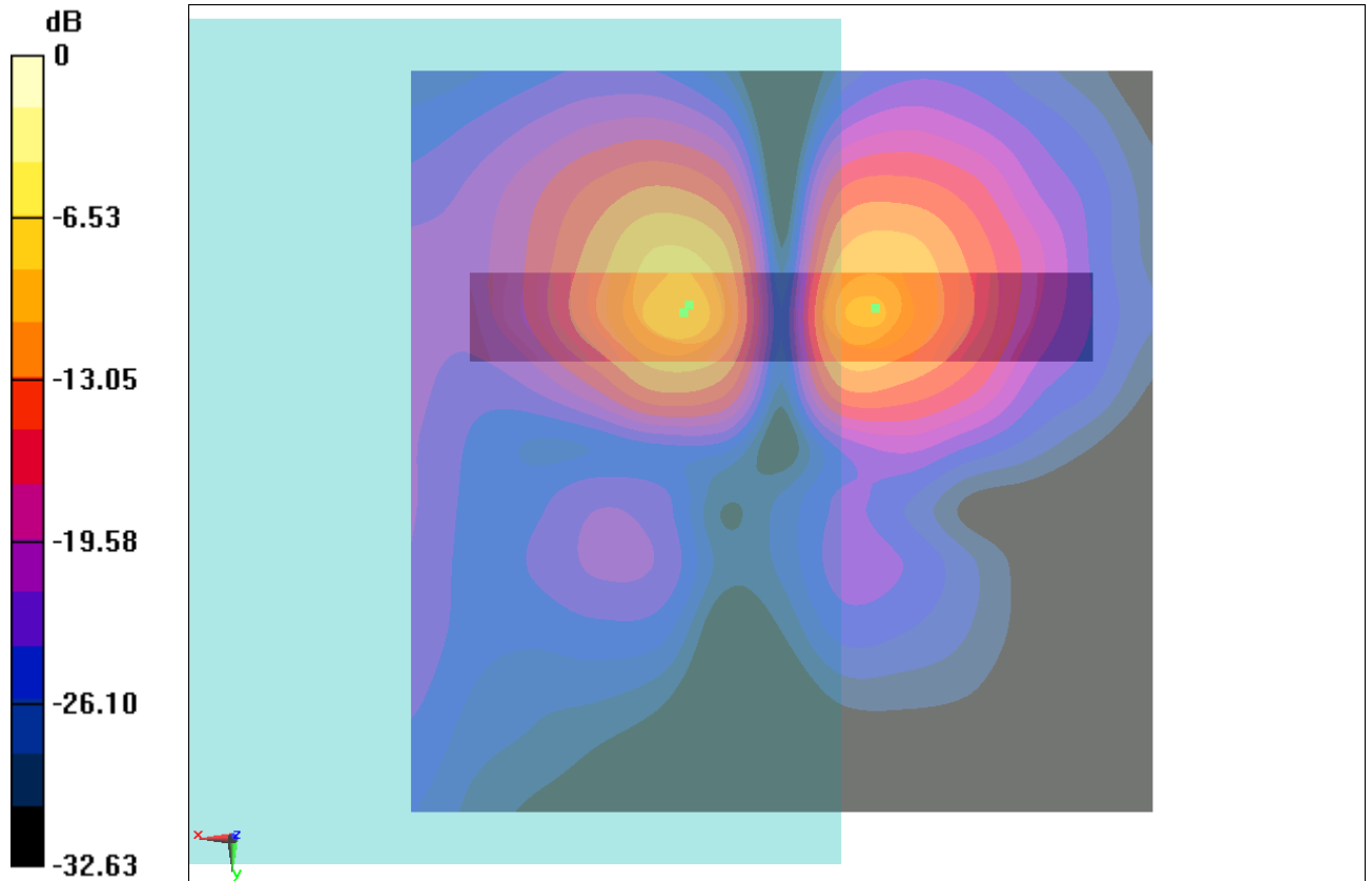
Fig B.7 T-Coil CDMA 835_Channel 1013
