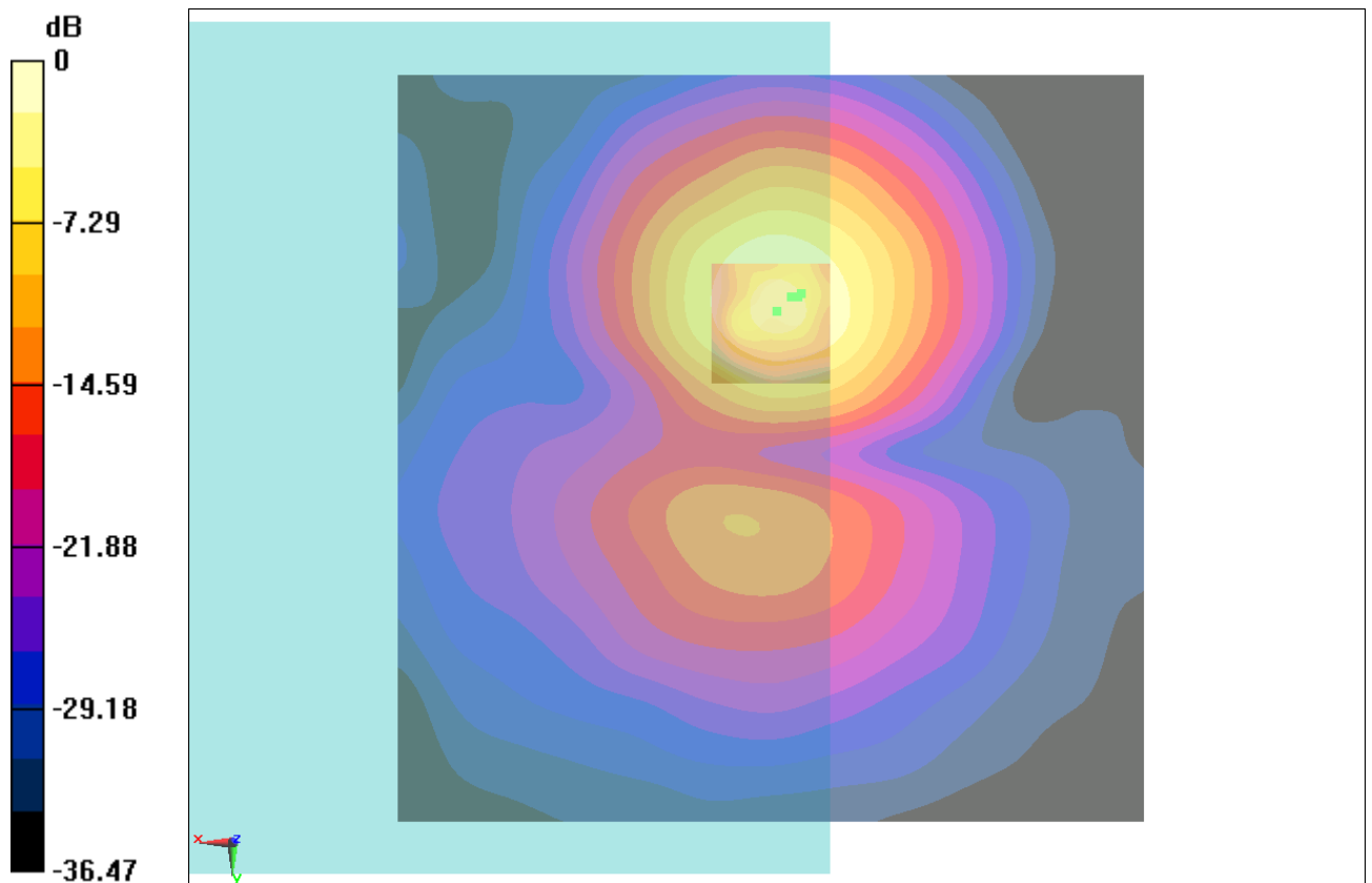
Fig B.12 T-Coil CDMA 1880_Channel 1175
