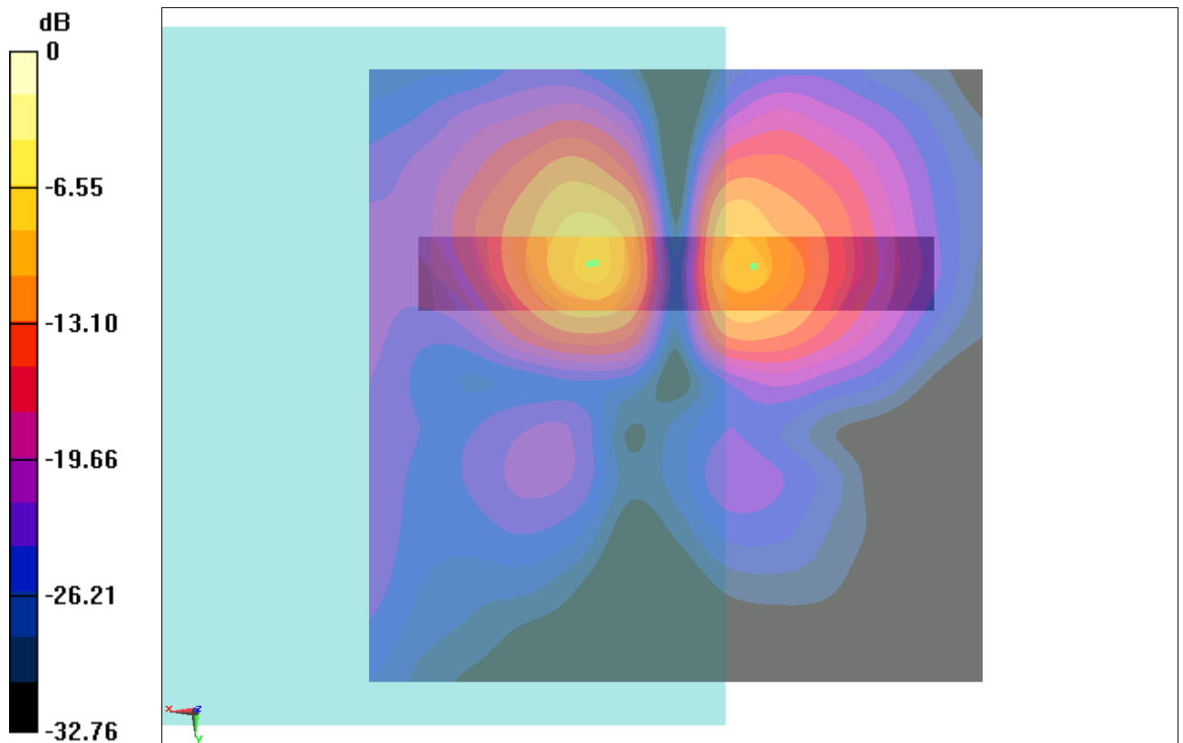
Fig B.1 T-Coil CDMA 835_Channel 777
