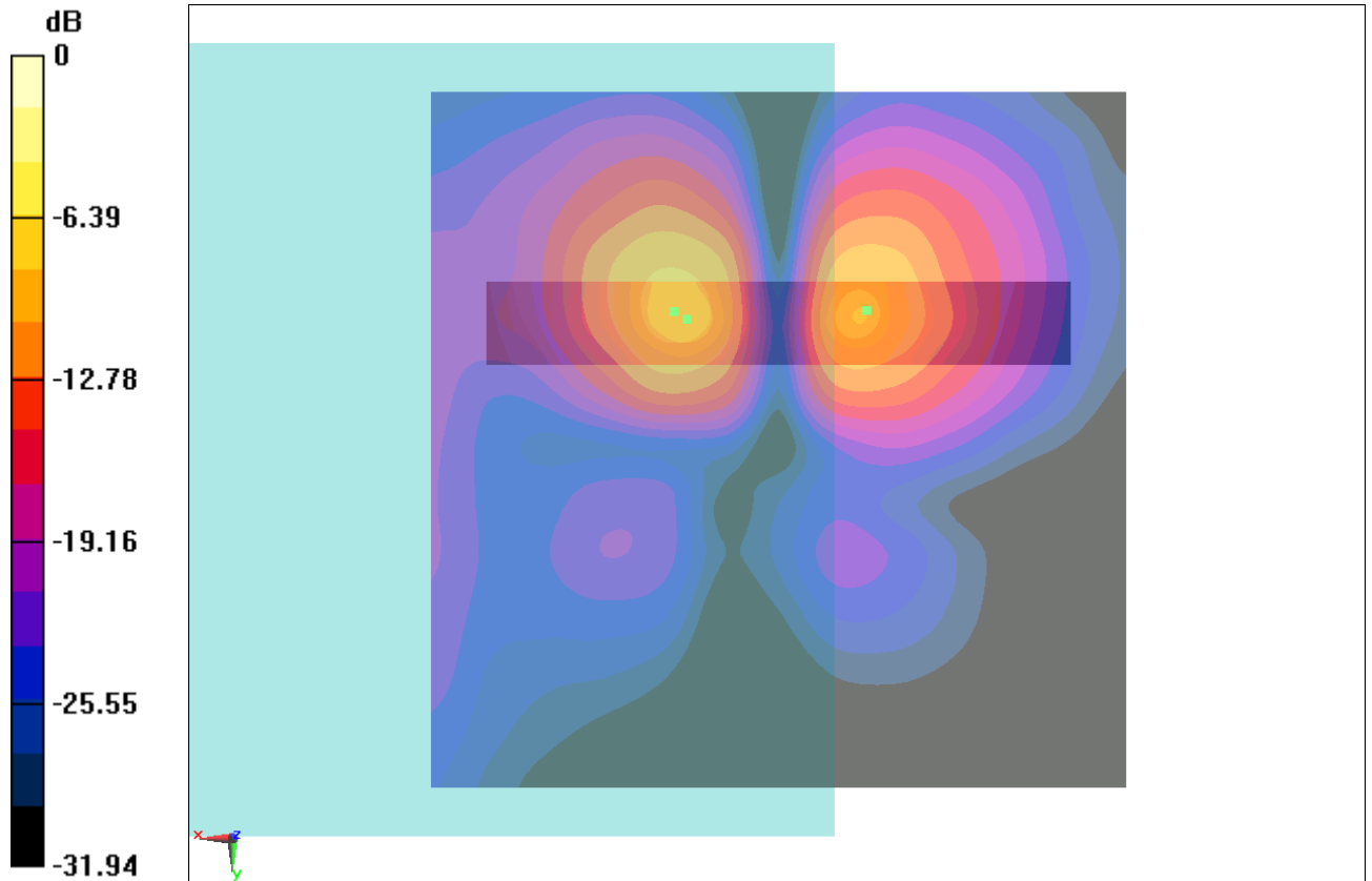
Fig B.10 T-Coil CDMA 1880_Channel 1175
