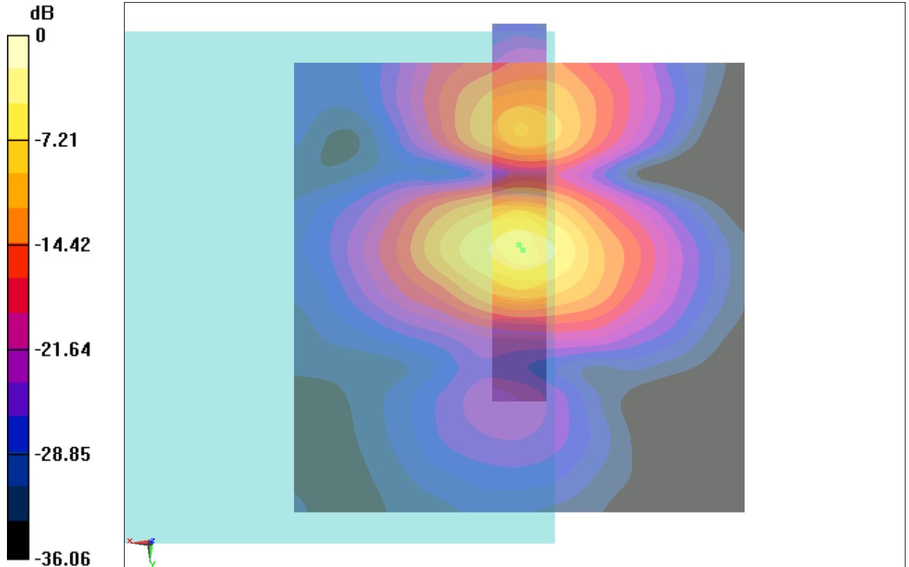
Fig B.14 T-Coil CDMA 1880_Channel 600
