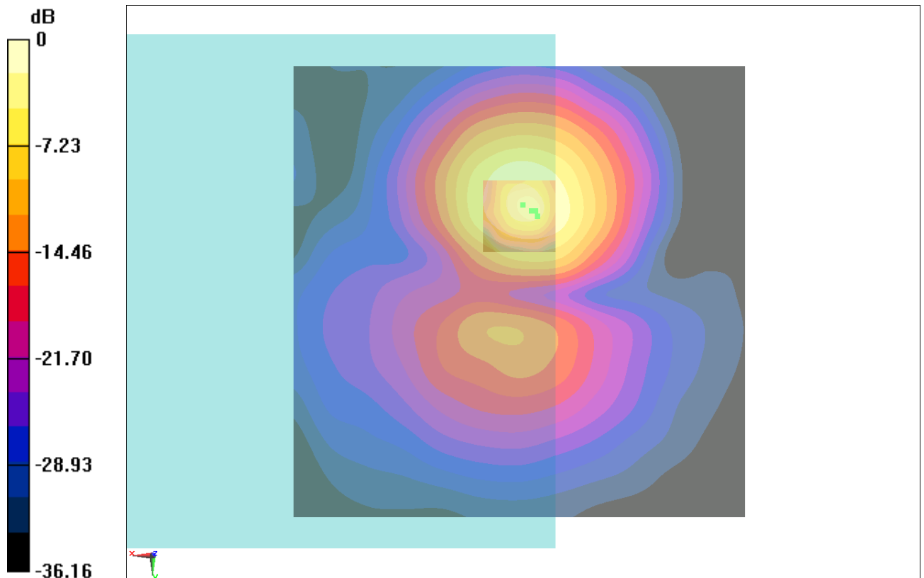
Fig B.15 T-Coil CDMA 1880_Channel 600
