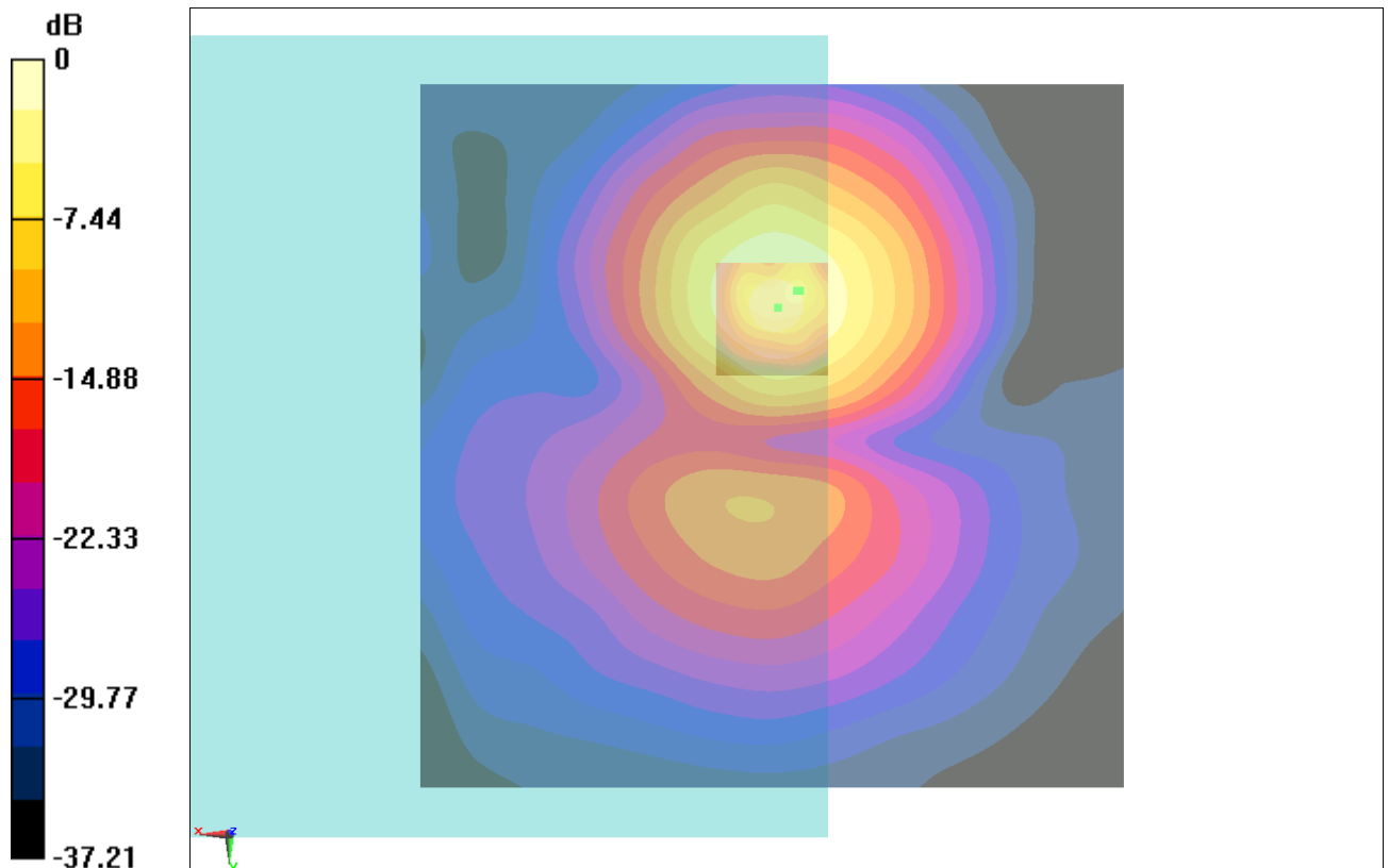
Fig B.18 T-Coil CDMA 1880_Channel 25
