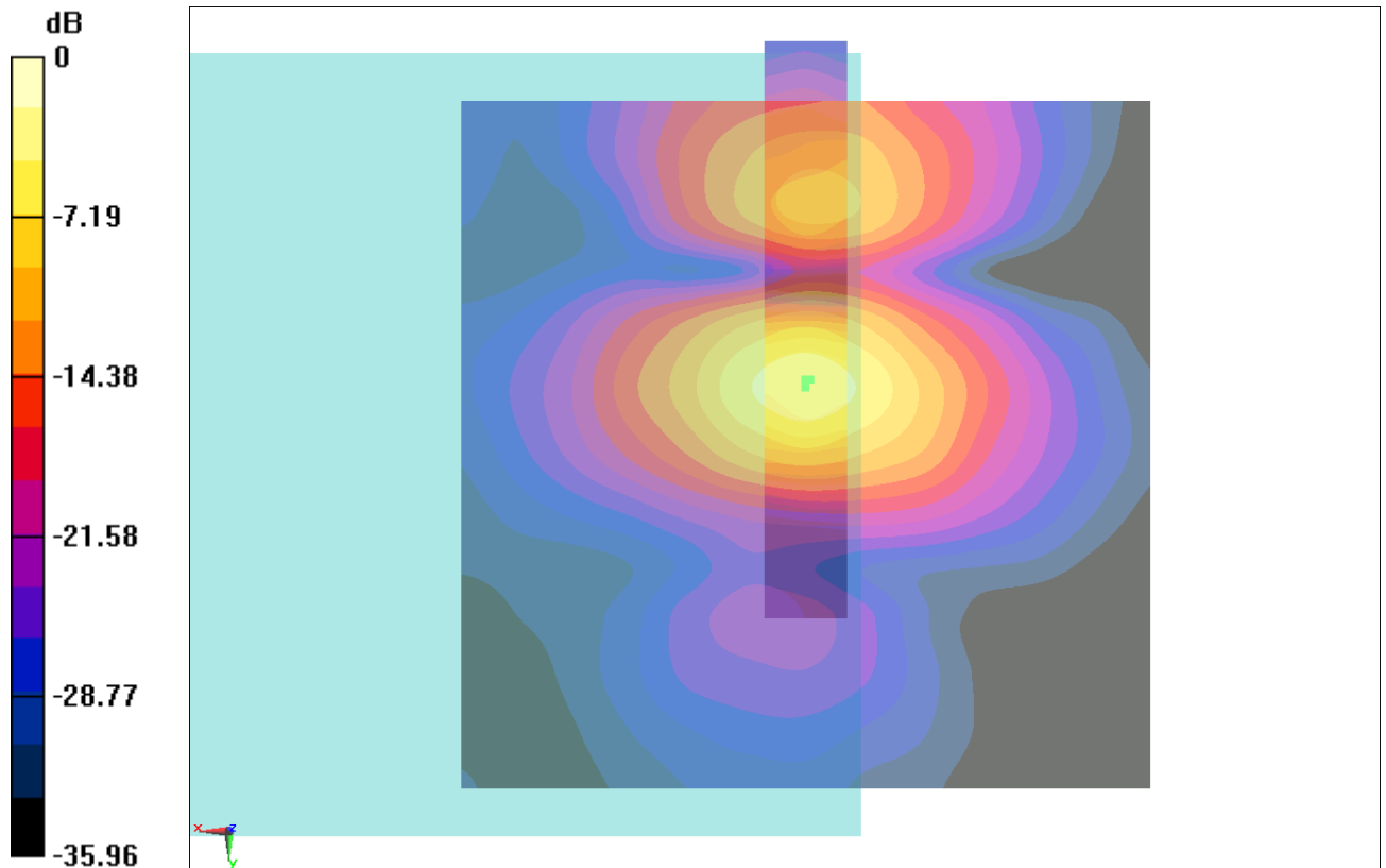
Fig B.17 T-Coil CDMA 1880_Channel 25
