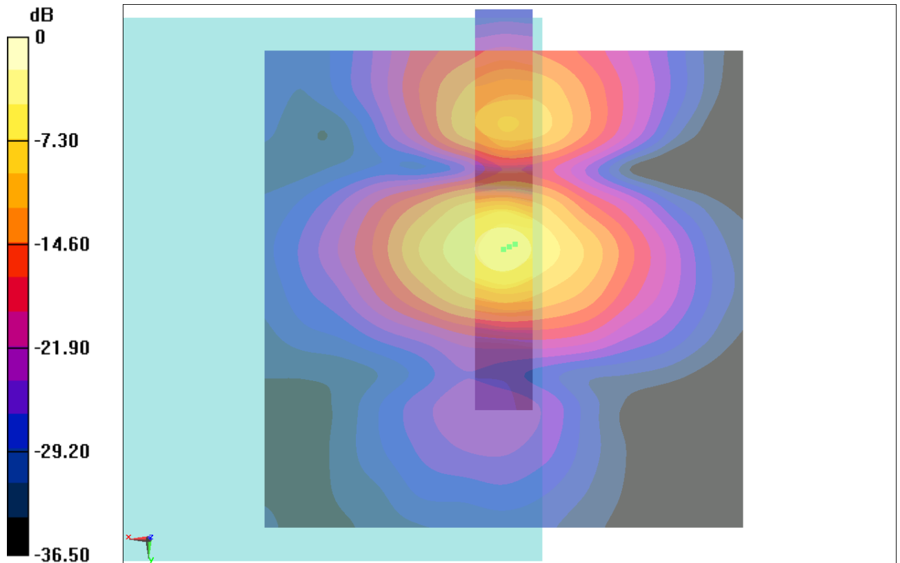
Fig B.2 T-Coil CDMA 835_Channel 777
