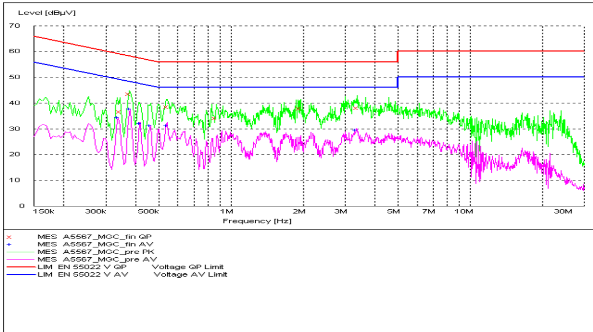
Fig. 78 AC Powerline Conducted Emission-802.11g
