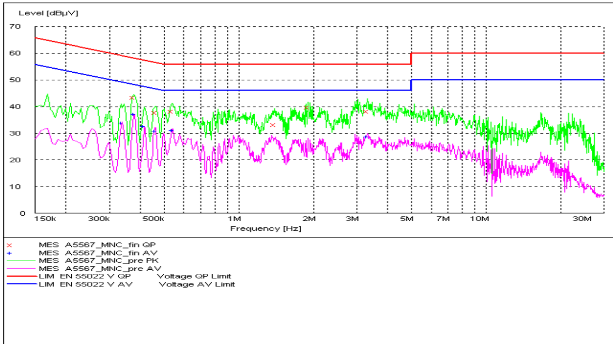
Fig. 79 AC Powerline Conducted Emission-802.11n-20MHz
