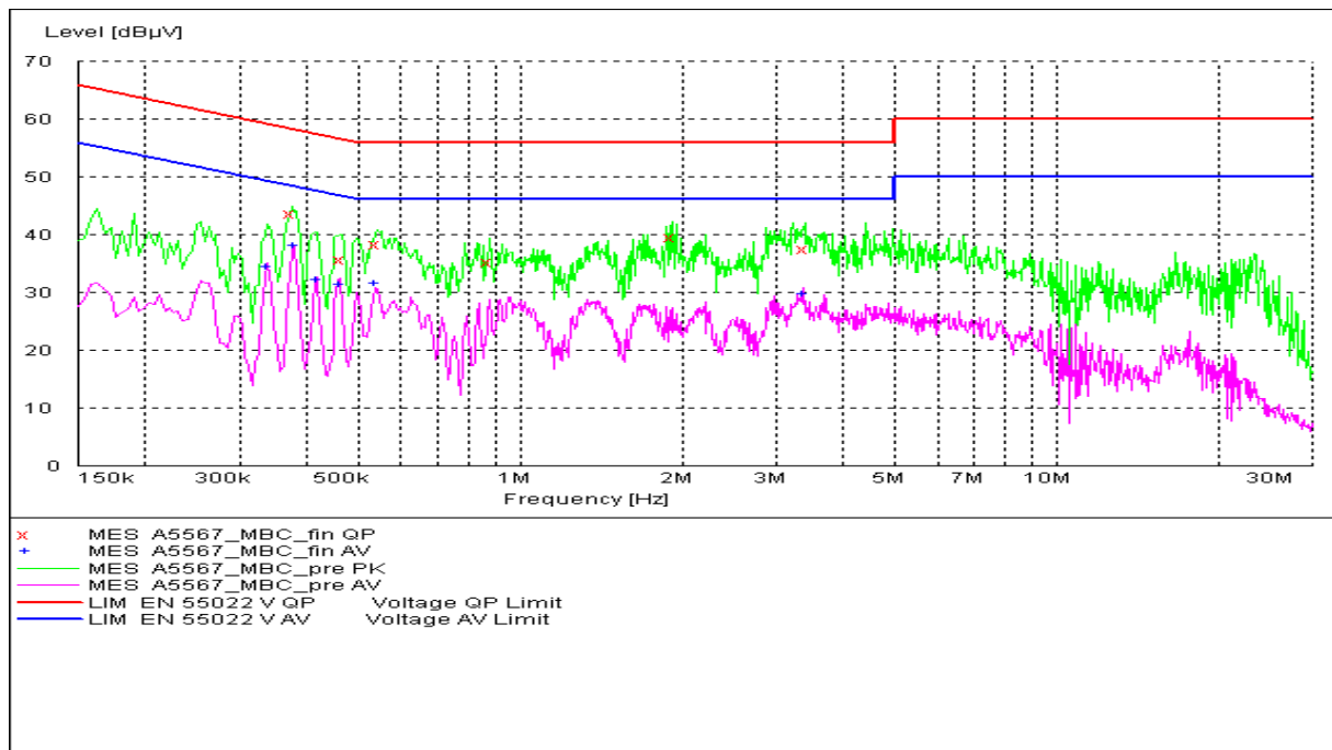
Fig. 77 AC Powerline Conducted Emission-802.11b
