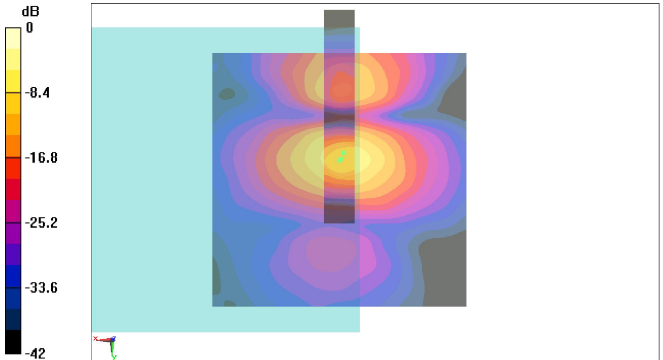
Fig B.2 T-Coil CDMA 835_Channel 777
