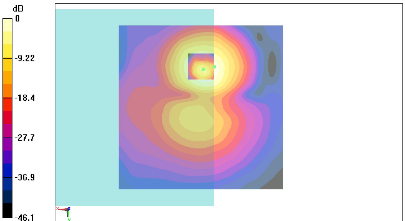
Fig B.3 T-Coil CDMA 835_Channel 777
