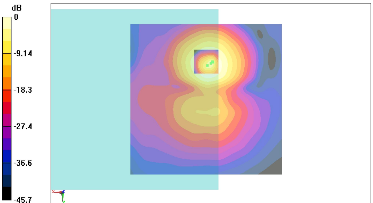
Fig B.9 T-Coil CDMA 835_Channel 1013
