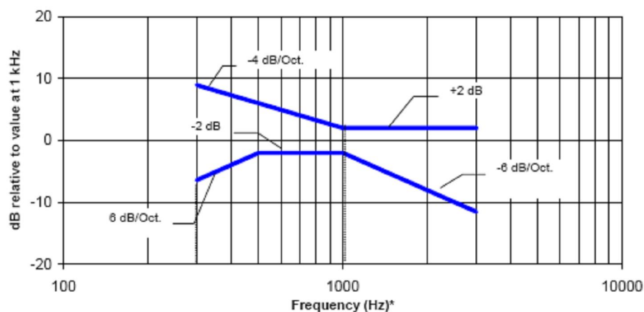
Figure 8.1—Magnetic field frequency response for WDs with a field -15 dB (A/m) at 1 kHz
