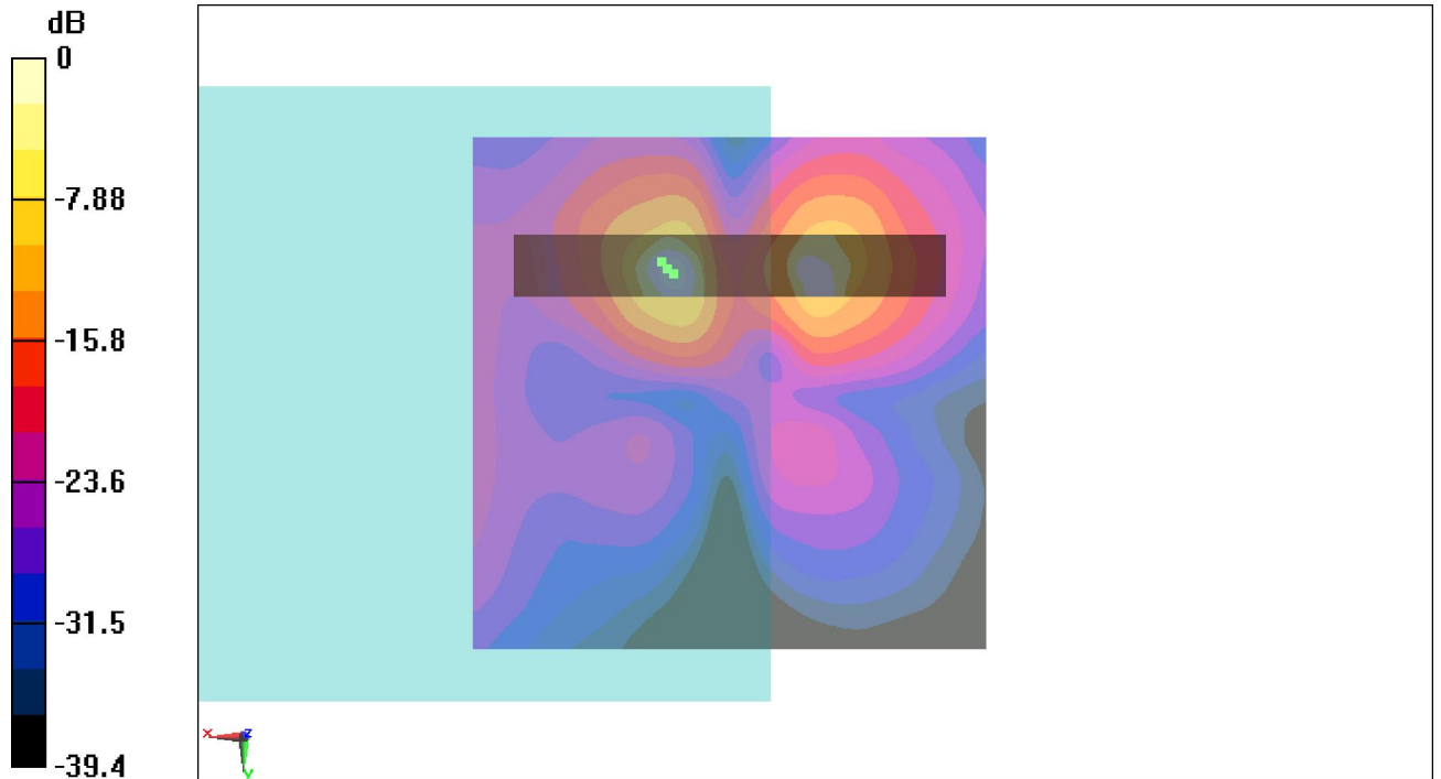
Fig B.1 T-Coil CDMA 835_Channel 777
