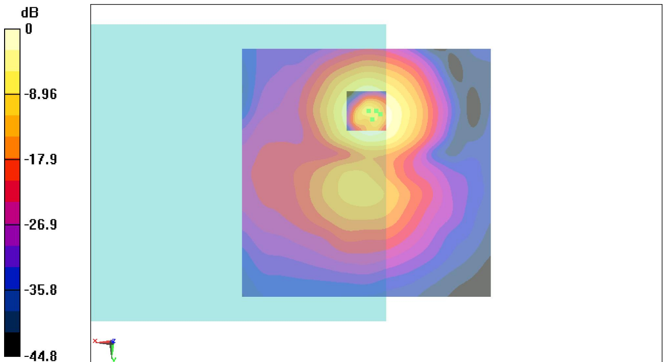
Fig B.15 T-Coil CDMA 1880_Channel 600
