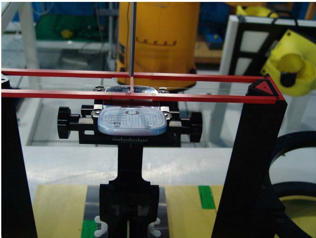
Picture 3: EUT Positioning for T-coil
