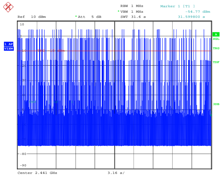
Fig.110. Time of occupancy (Dwell Time): Channel 39, Packet 3-DH5
