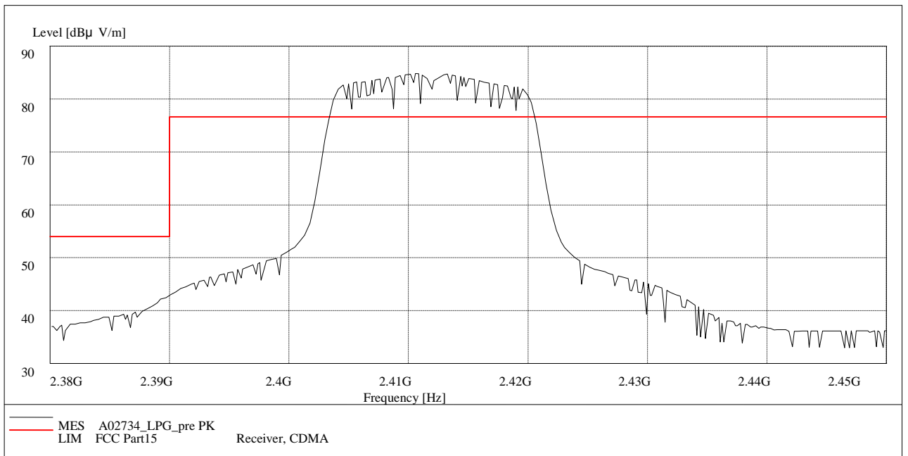
Fig. 76 Radiated Spurious Emission (Power): 802.11g, ch1, 2.38 GHz - 2.45GHz
