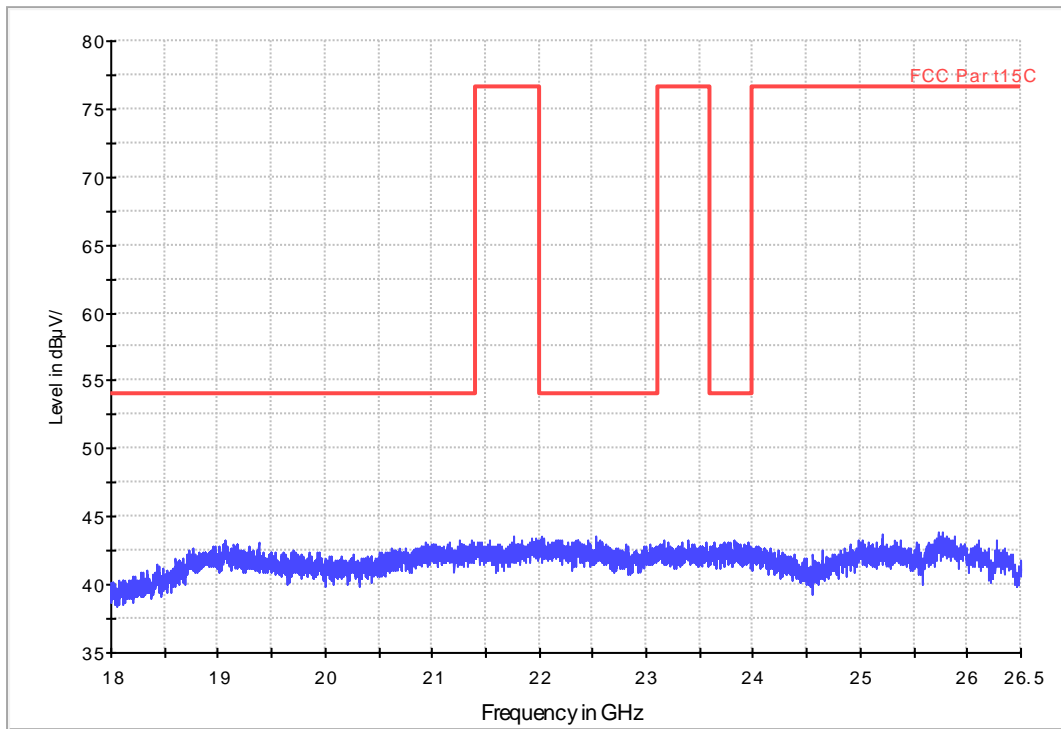
Fig. 87 Radiated emission: 18 GHz - 26.5 GHz
