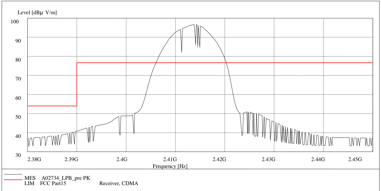
Fig. 65 Radiated Spurious Emission (Power): 802.11b, ch1, 2.38 GHz - 245GHz
