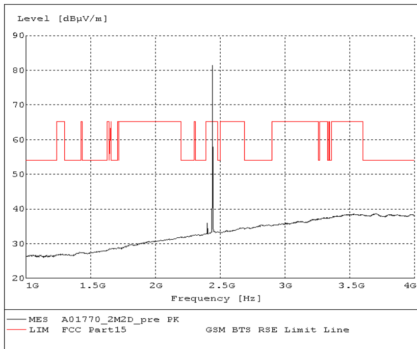
Fig.56. Radiated emission: \pi/4 DQPSK, Channel 39, 1 GHz - 4 GHz
