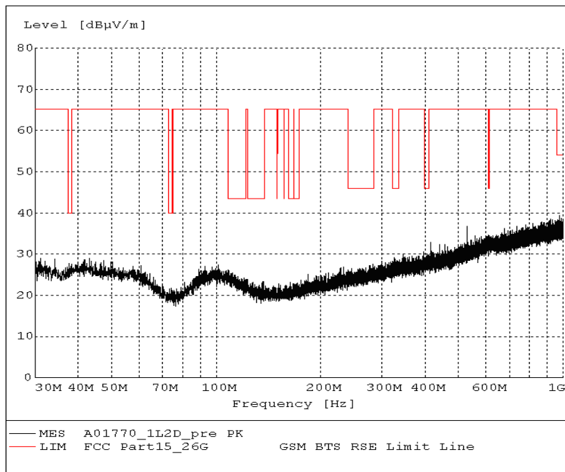
Fig.52. Radiated emission: \pi/4 DQPSK, Channel 0, 30 MHz - 1 GHz
