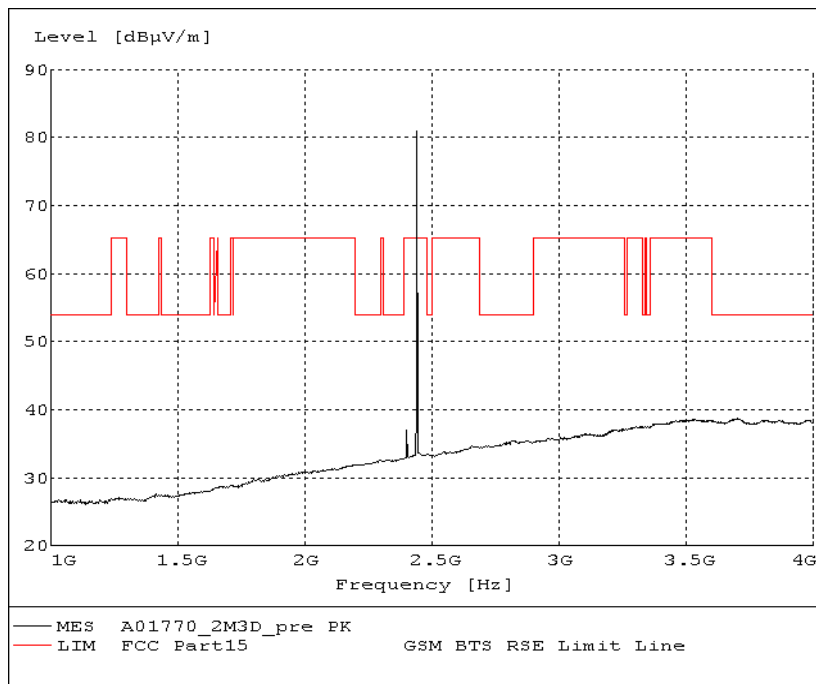
Fig.68. Radiated emission: 8DPSK, Channel 39, 1 GHz - 4 GHz
