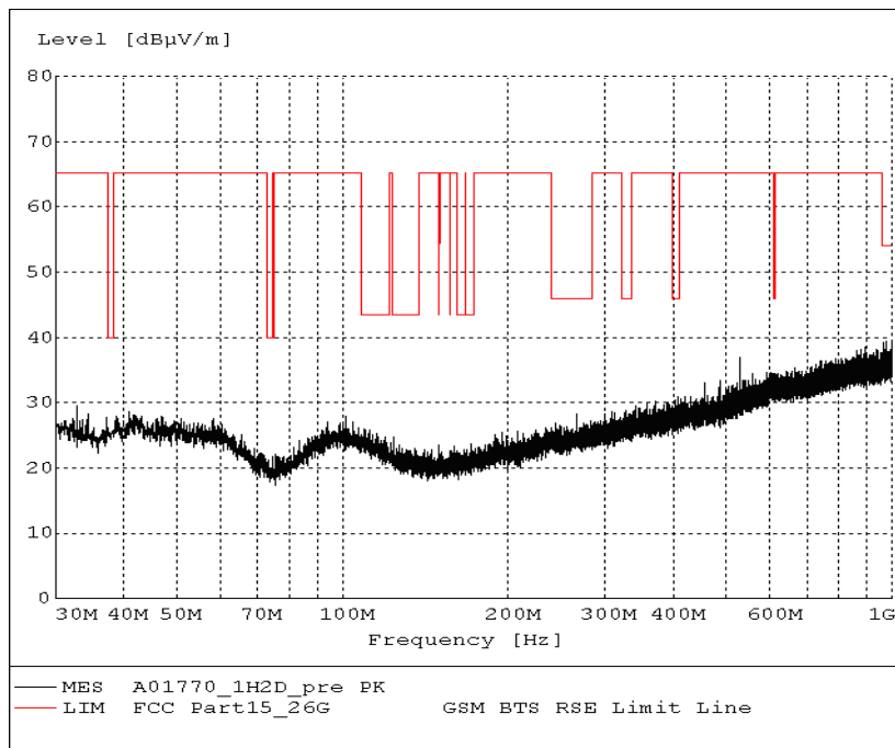
Fig.58. Radiated emission: \pi/4 DQPSK, Channel 78, 30 MHz - 1 GHz
