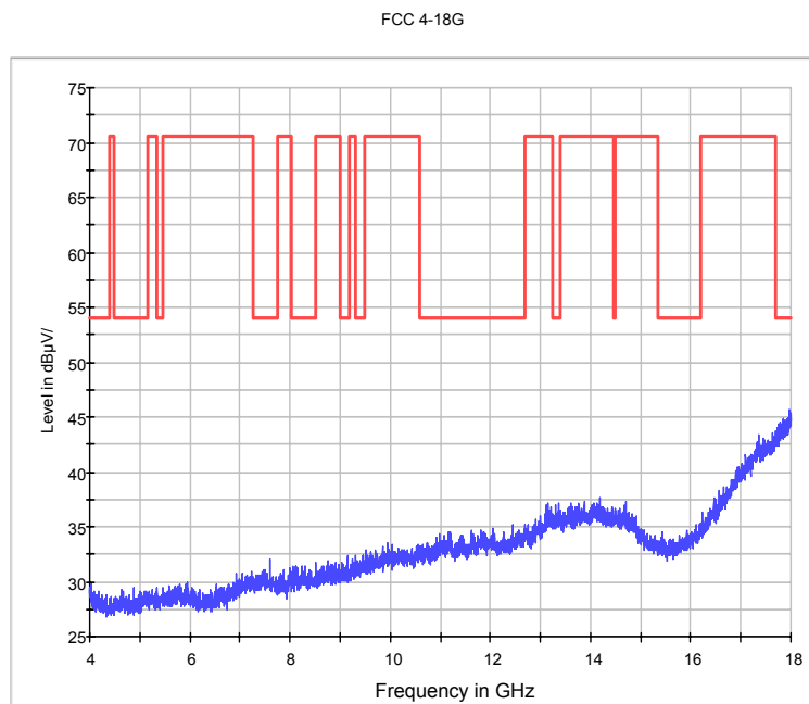
Fig.45. Radiated emission: GFSK, Channel 39, 4 GHz - 18 GHz
