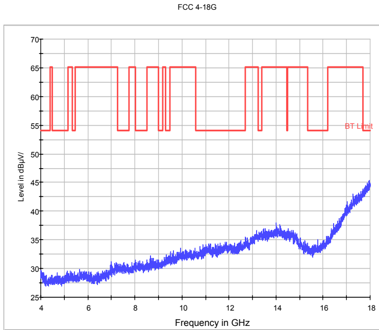
Fig.54. Radiated emission: \pi/4 DQPSK, Channel 0, 4 GHz - 18 GHz
