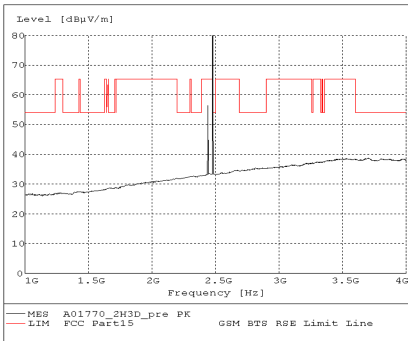
Fig.71. Radiated emission: 8DPSK, Channel 78, 1 GHz - 4 GHz
