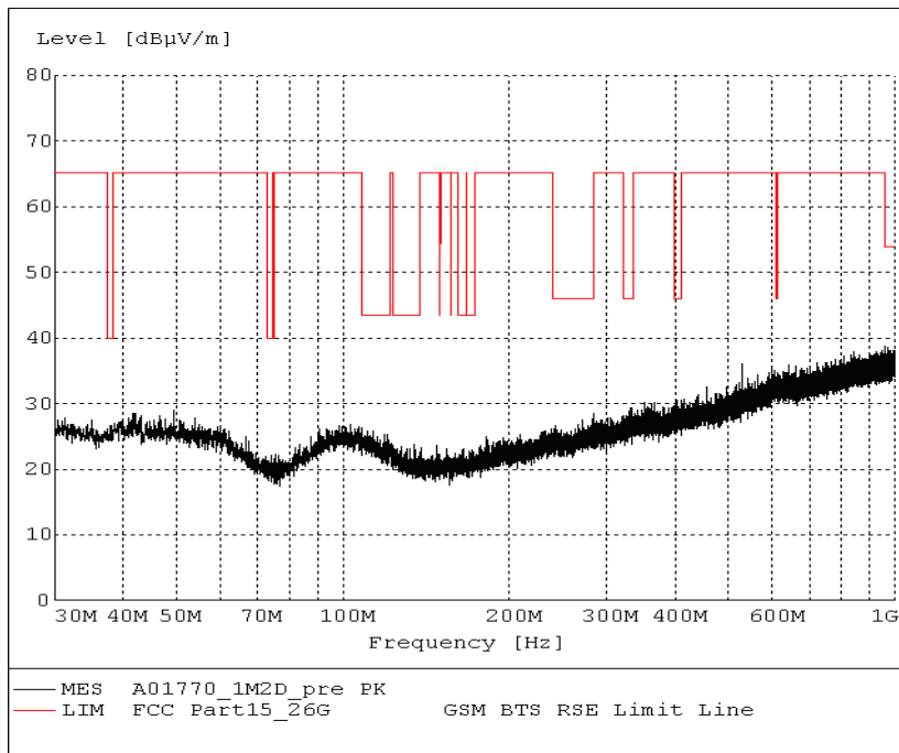
Fig.55. Radiated emission: \pi/4 DQPSK, Channel 39, 30 MHz - 1 GHz
