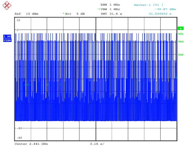
Fig.84 Time of occupancy (Dwell Time): Channel 39, Packet 2-DH3
