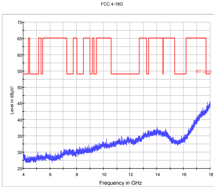
Fig.72. Radiated emission: 8DPSK, Channel 78, 4 GHz - 18 GHz
