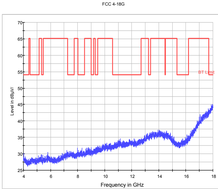
Fig.42. Radiated emission: GFSK, Channel 0, 4 GHz - 18 GHz
