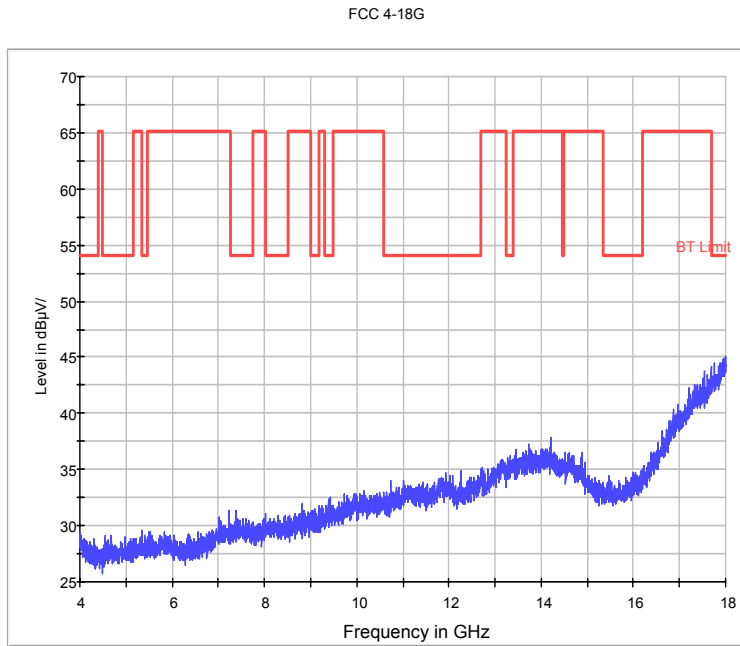
Fig.48. Radiated emission: GFSK, Channel 78, 4 GHz - 18 GHz
