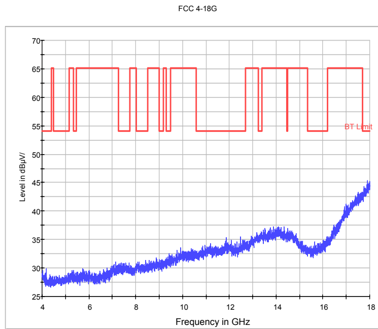
Fig.60. Radiated emission: \pi/4 DQPSK, Channel 78, 4 GHz - 18 GHz
