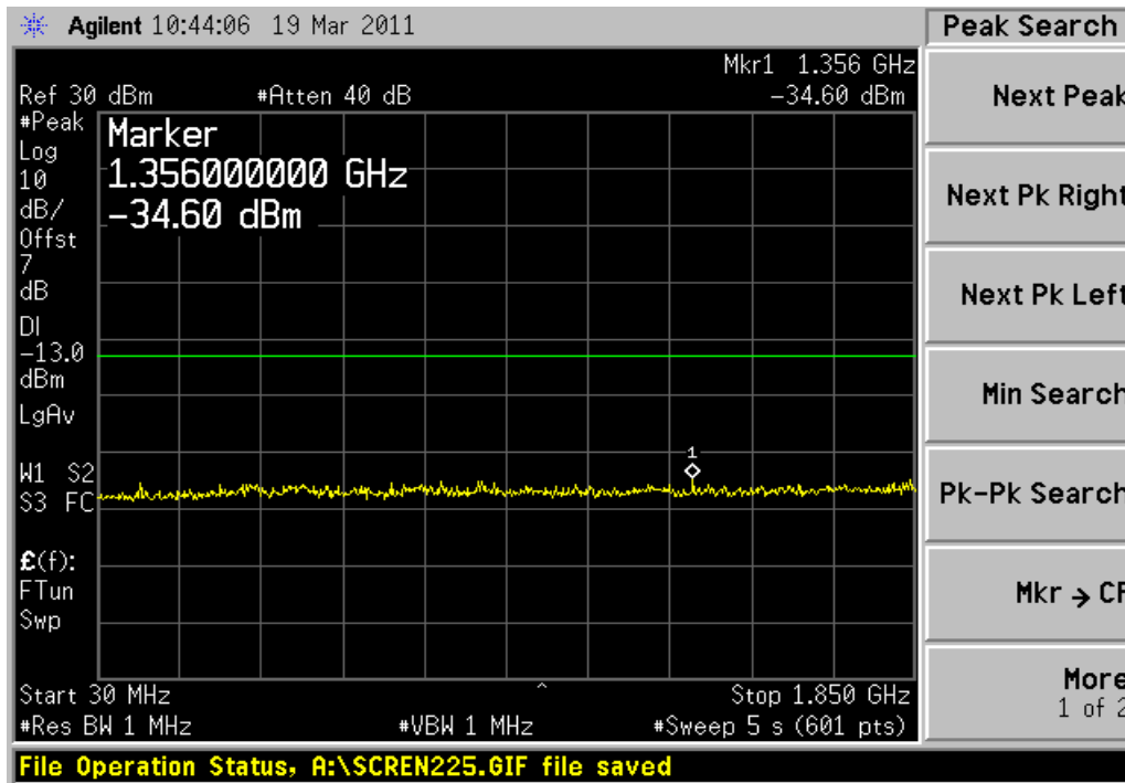
Channel 661, 30MHz~1850MHz
