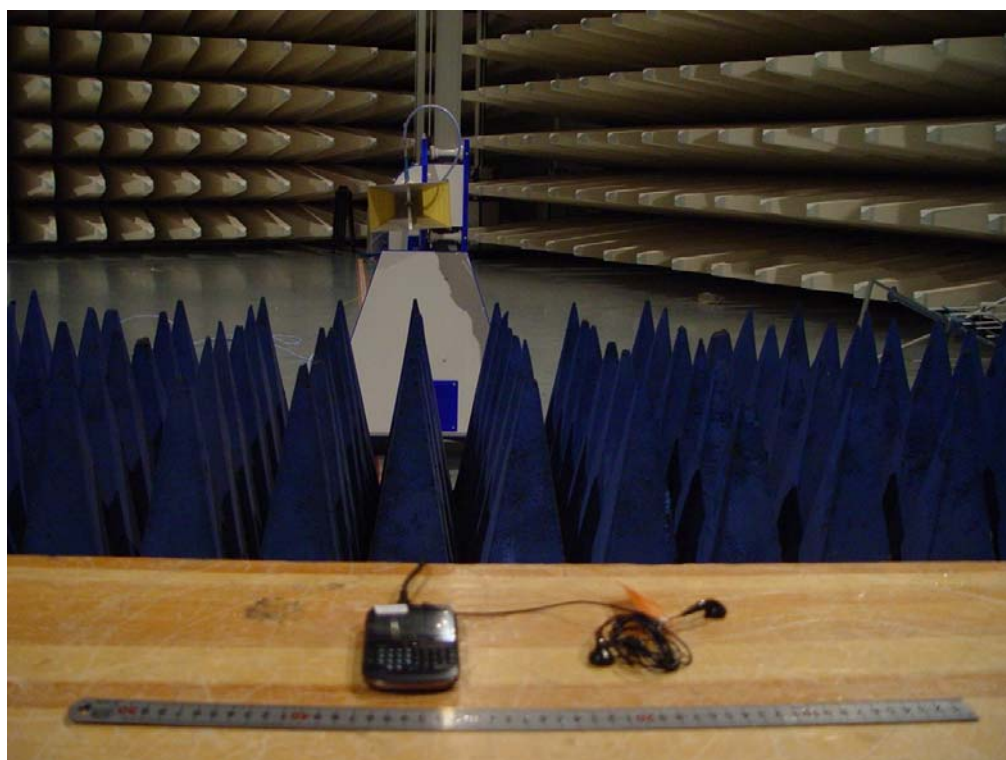
Spurious Radiated Emissions Test setup
