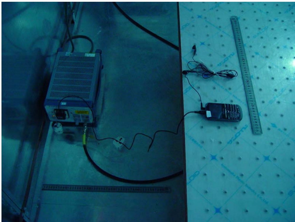
AC Power Line Conducted Emission Test setup
