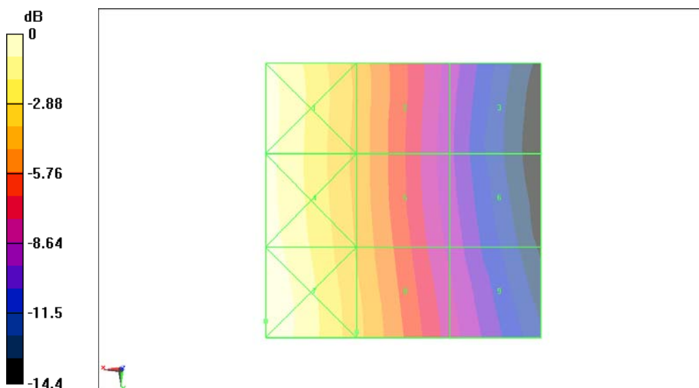
Fig B.14 HAC RF H-Field GSM 850 Middle
