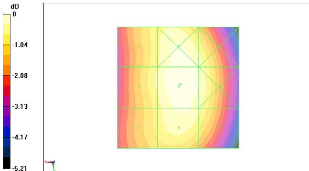
Fig B.7 HAC RF E-Field WCDMA 850 High
