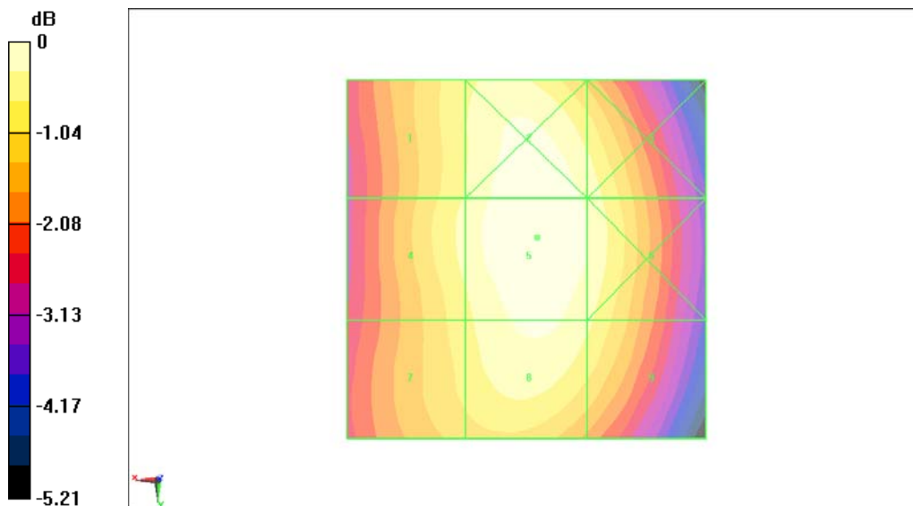
Fig B.8 HAC RF E-Field WCDMA 850 Middle
