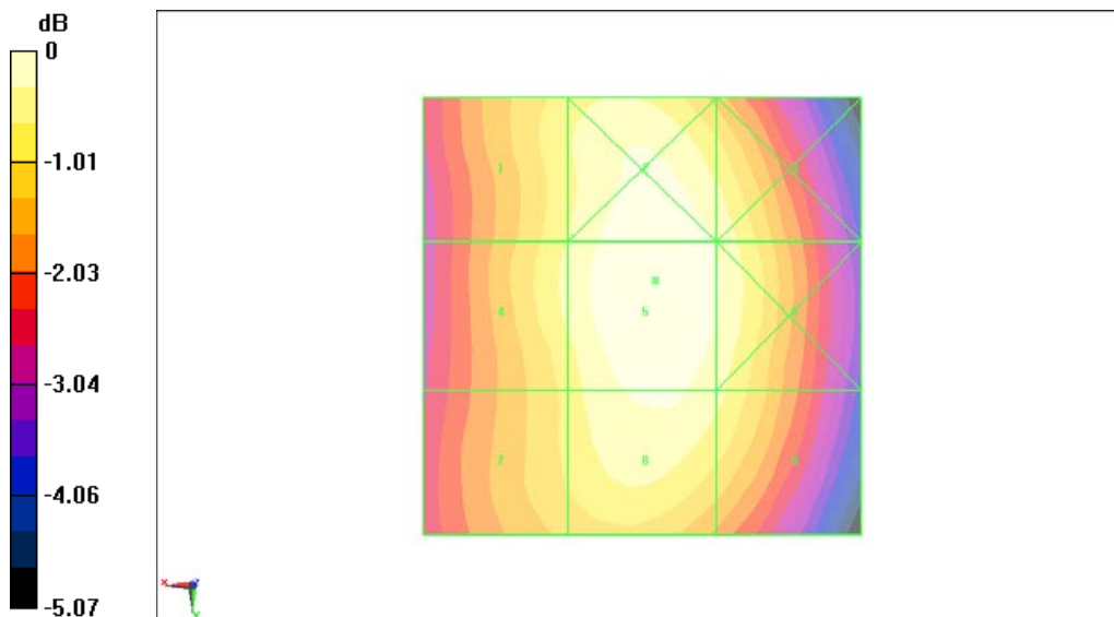
Fig B.9 HAC RF E-Field WCDMA 850 Low
