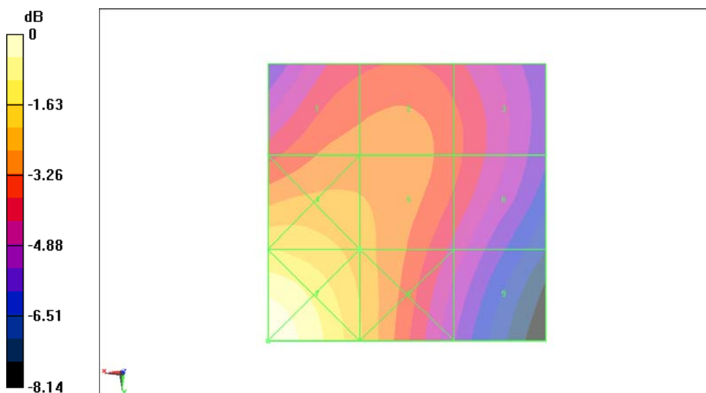
Fig B.24 HAC RF H-Field WCDMA 1900 Low
