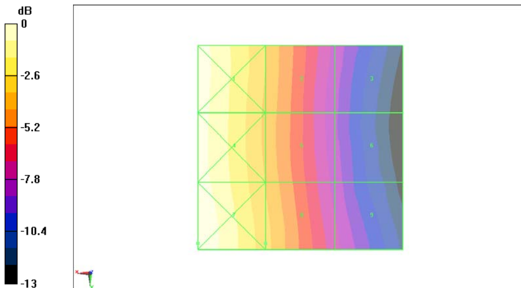
Fig B.21 HAC RF H-Field WCDMA 850 Low
