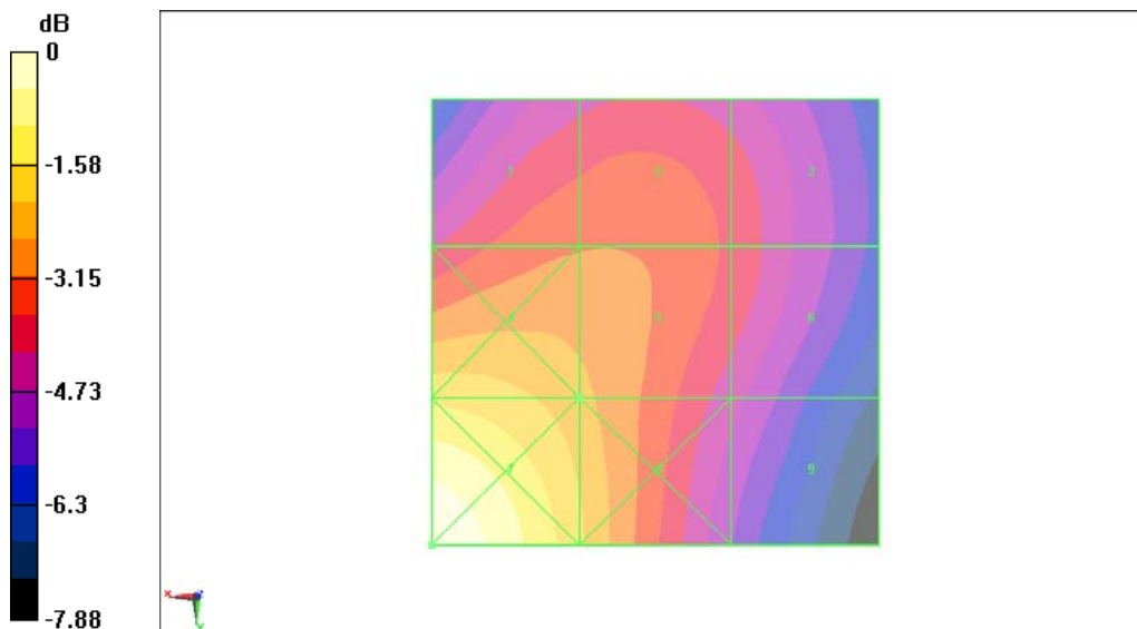
Fig B.23 HAC RF H-Field WCDMA 1900 Middle
