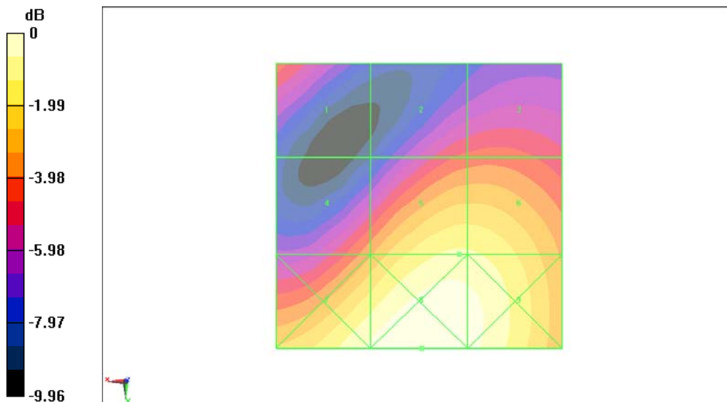
Fig B.11 HAC RF E-Field WCDMA 1900 Middle
