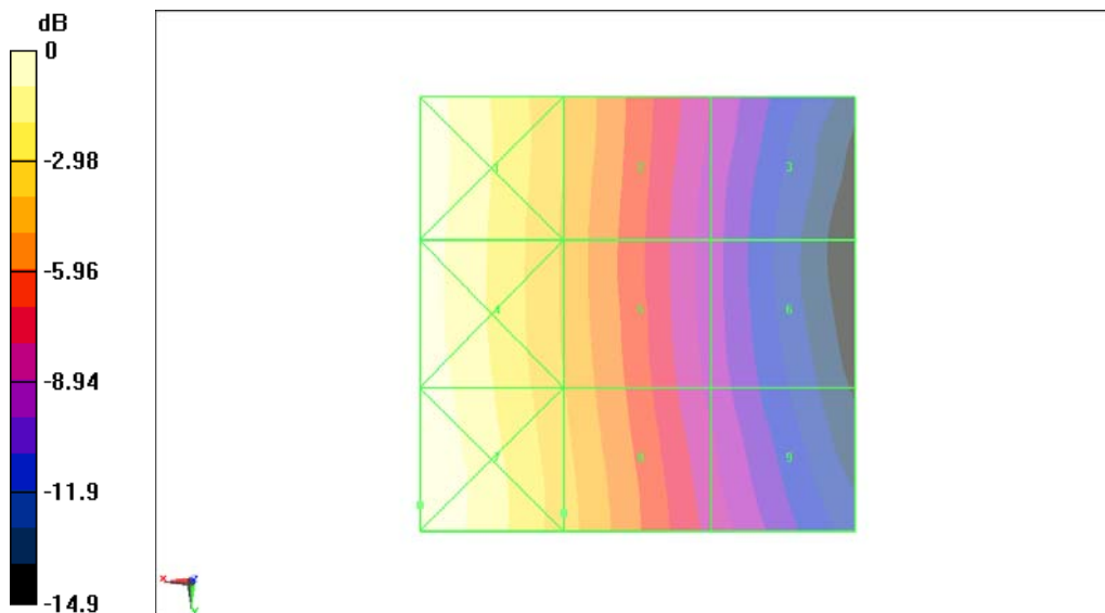
Fig B.15 HAC RF H-Field GSM 850 Low
