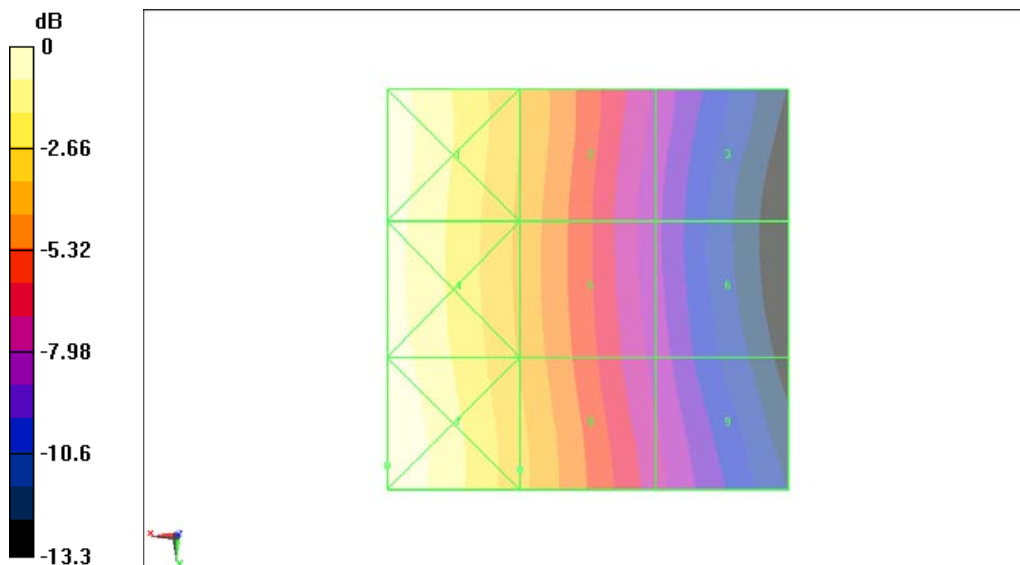
Fig B.19 HAC RF H-Field WCDMA 850 High
