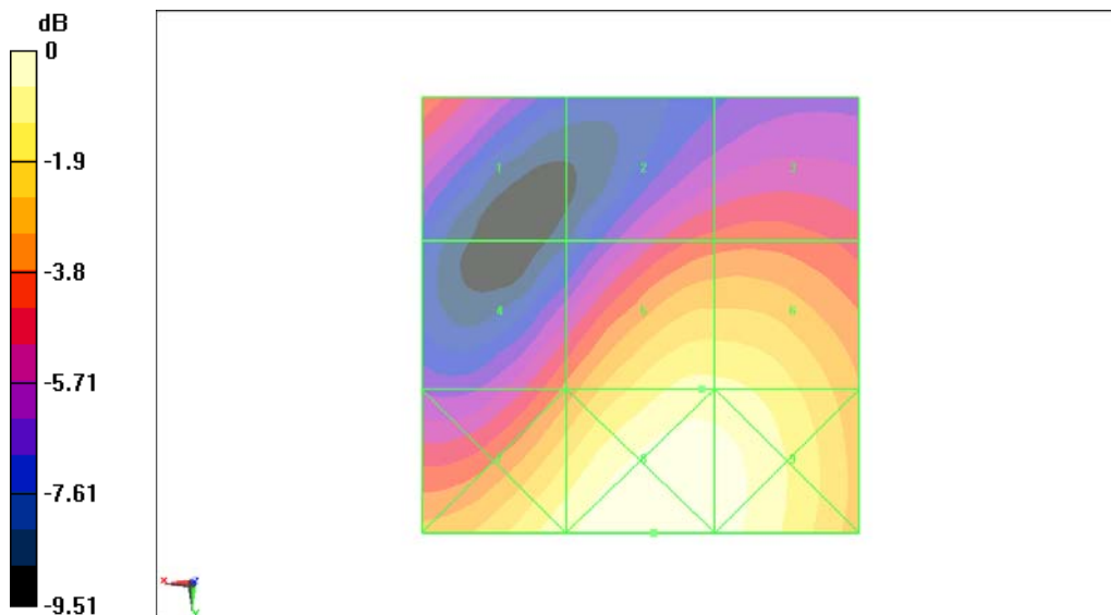
Fig B.10 HAC RF E-Field WCDMA 1900 High
