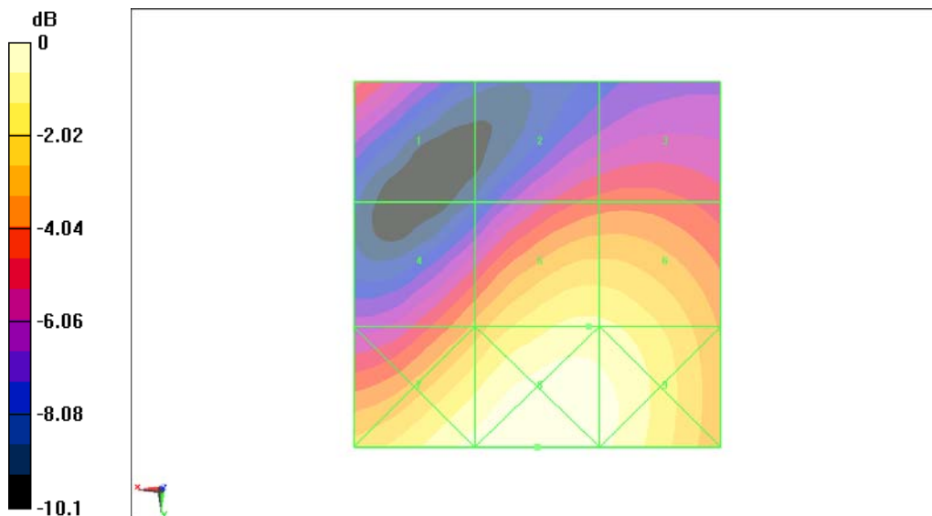
Fig B.12 HAC RF E-Field WCDMA 1900 Low
