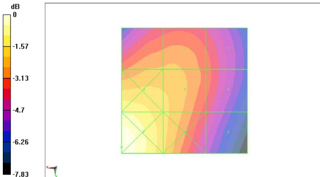
Fig B.18 HAC RF H-Field GSM 1900 Low
