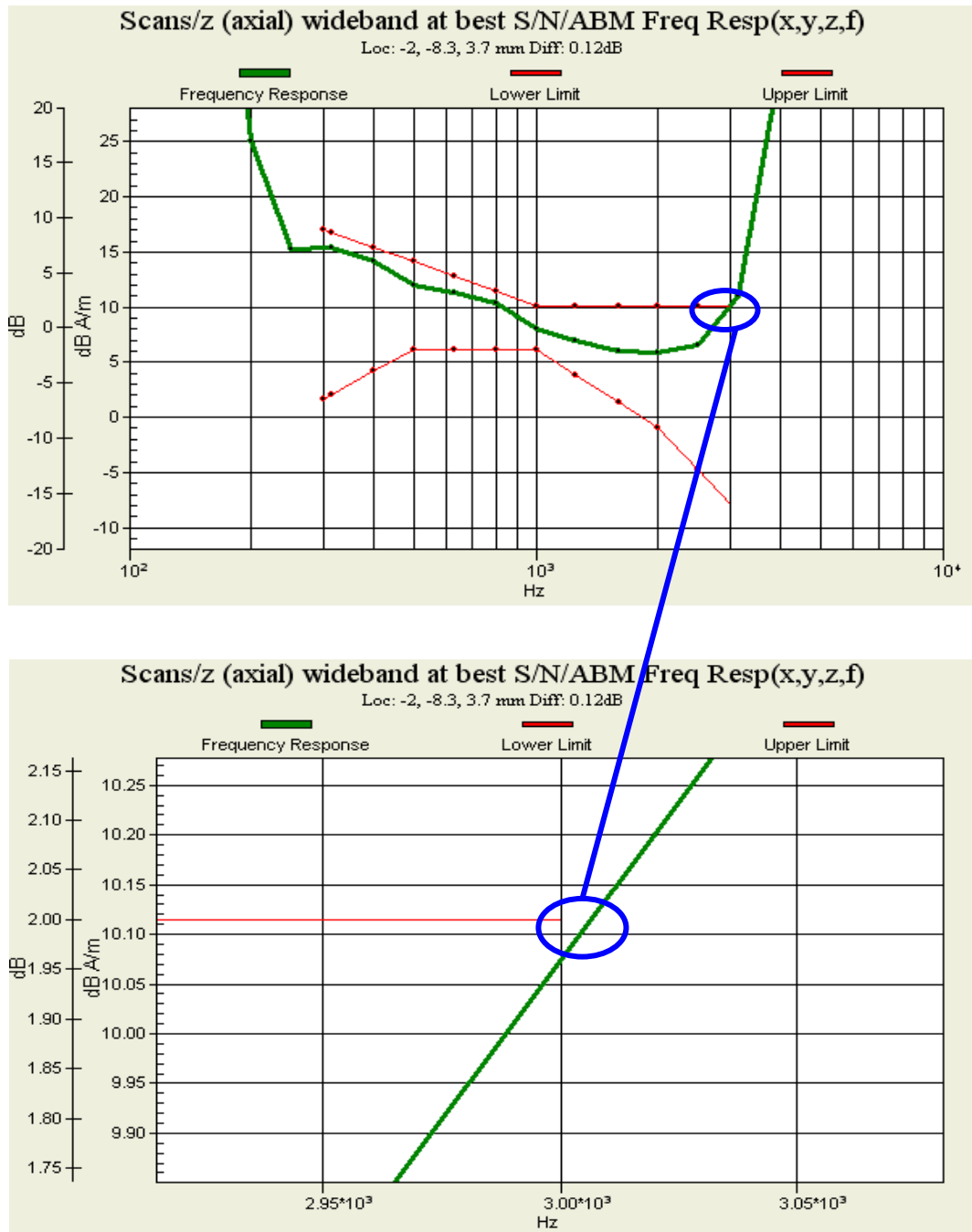
Figure 22 T-Coil WCDMA Band V Z Axial
