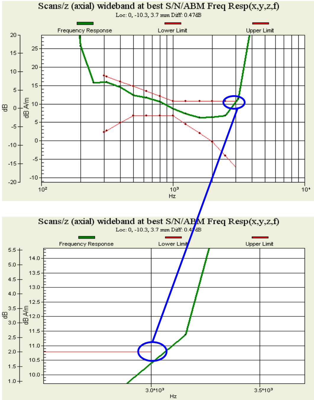
Figure 19 T-Coil WCDMA Band II Z Axial
