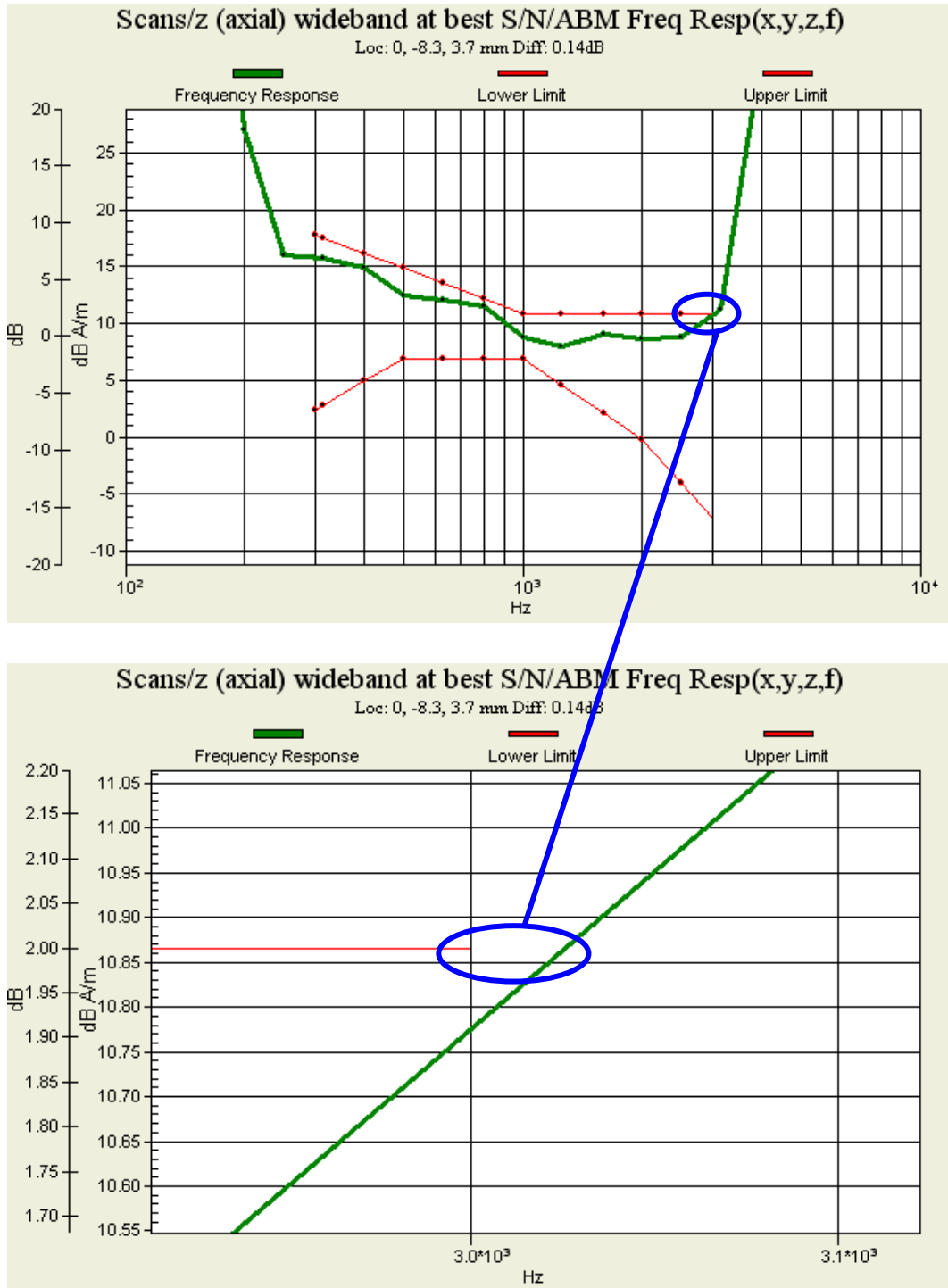
Figure 13 T-Coil GSM 850 Z Axial
