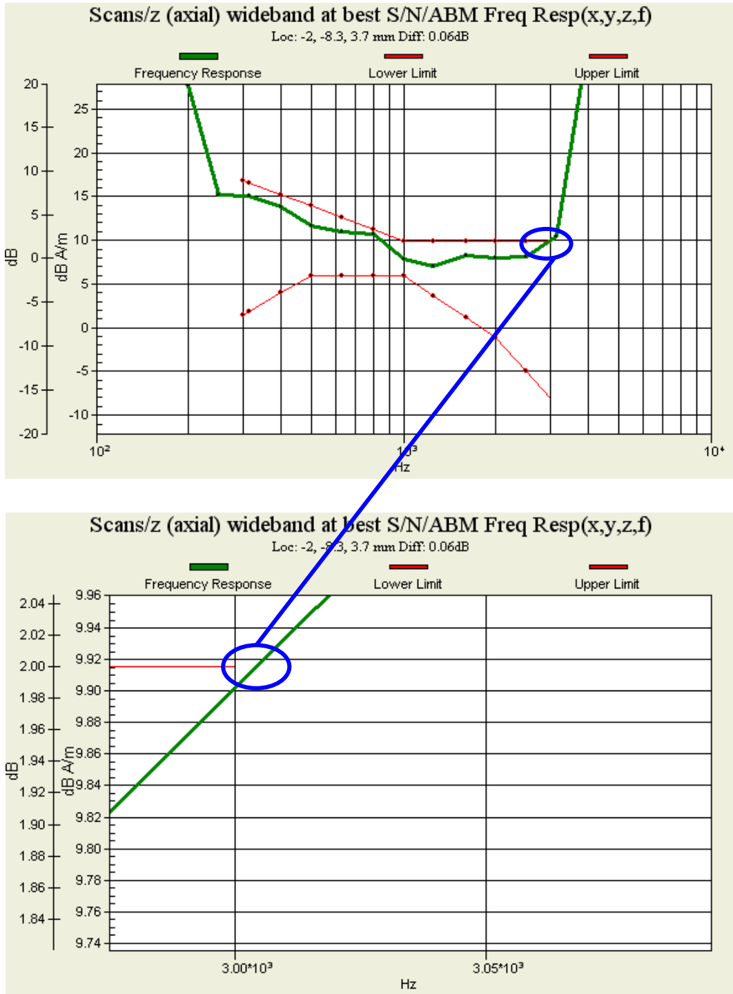
Figure 16 T-Coil GSM 1900 Z Axial
