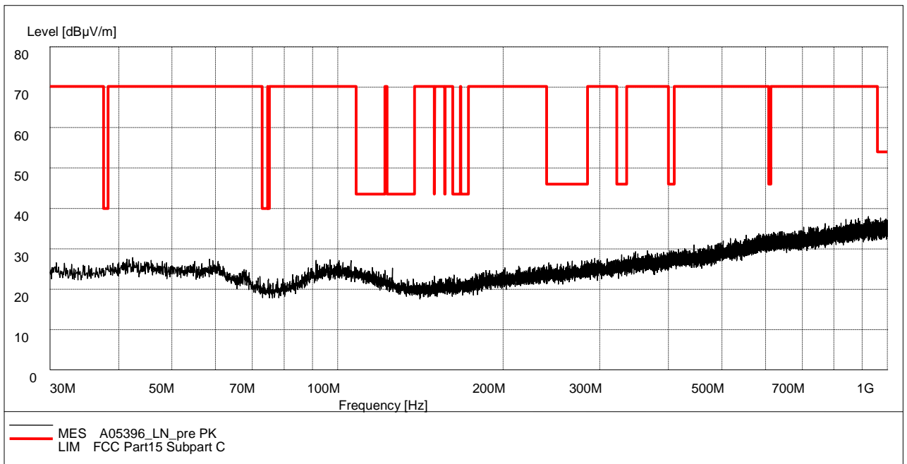
Fig. 66 Radiated Spurious Emission (802.11n-20MHz, Ch1, 30 MHz-1 GHz)
