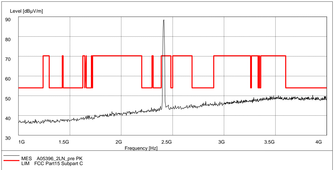
Fig. 67 Radiated Spurious Emission (802.11n-20MHz, Ch1, 1 GHz-4 GHz)
