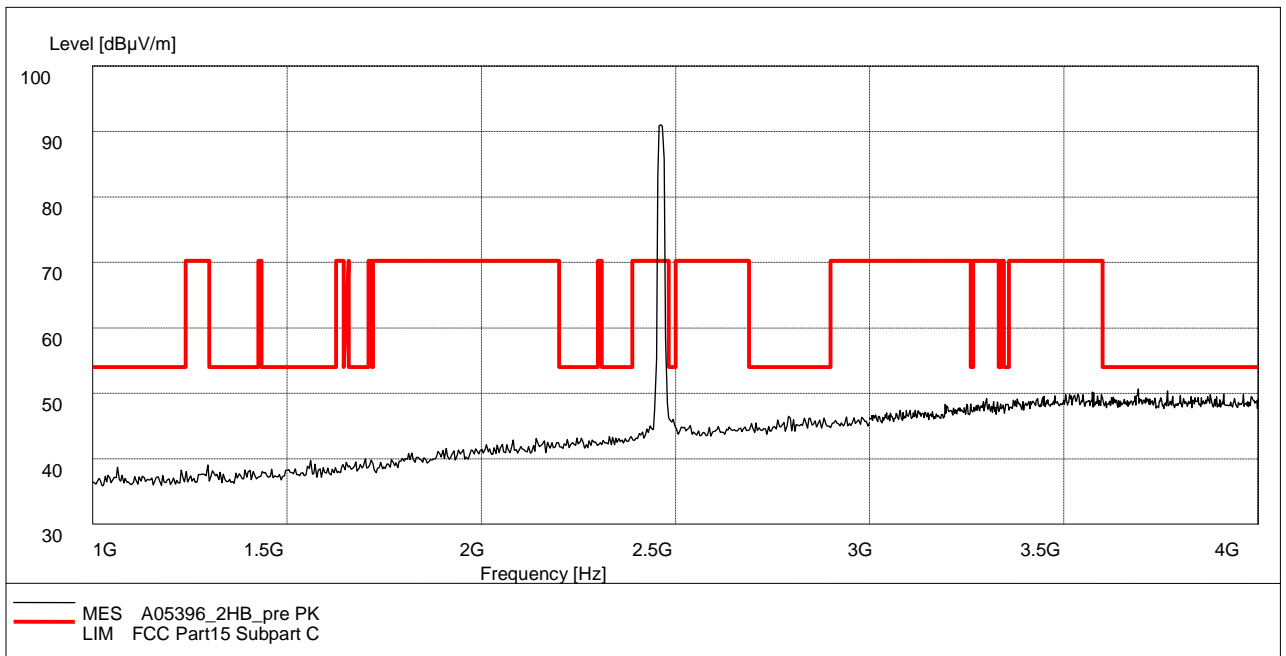
Fig. 52 Radiated Spurious Emission (802.11b, Ch11, 1 GHz-4 GHz)
