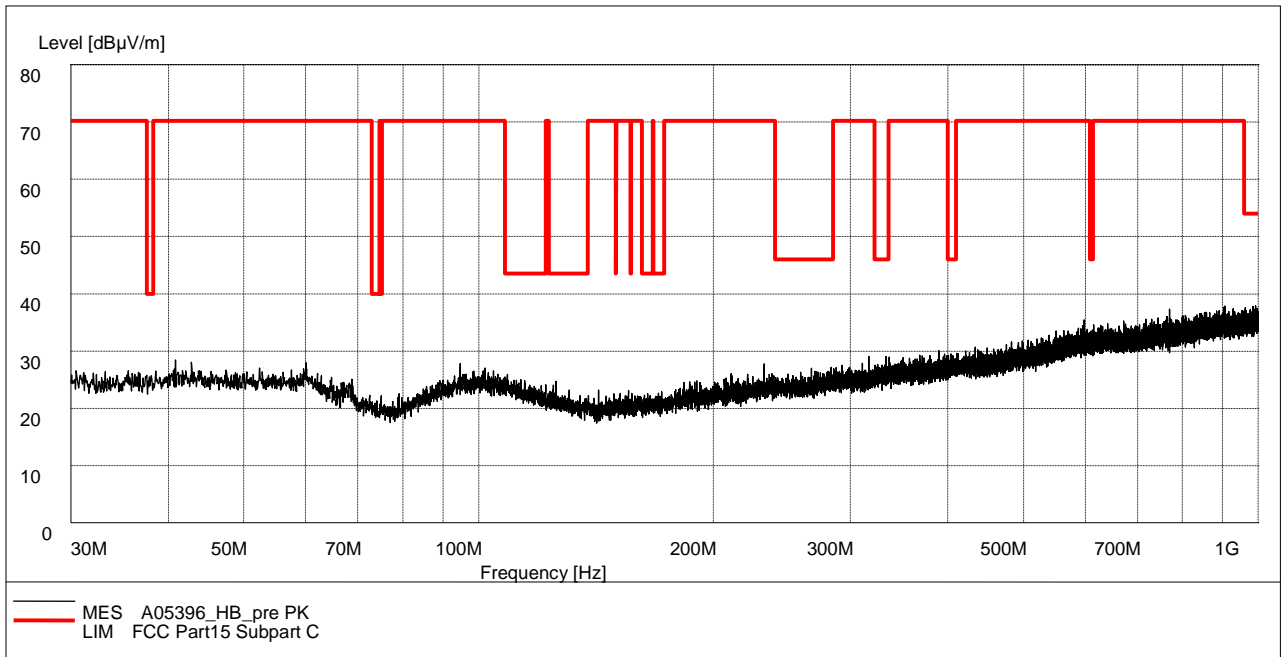
Fig. 51 Radiated Spurious Emission (802.11b, Ch11, 30 MHz-1 GHz)
