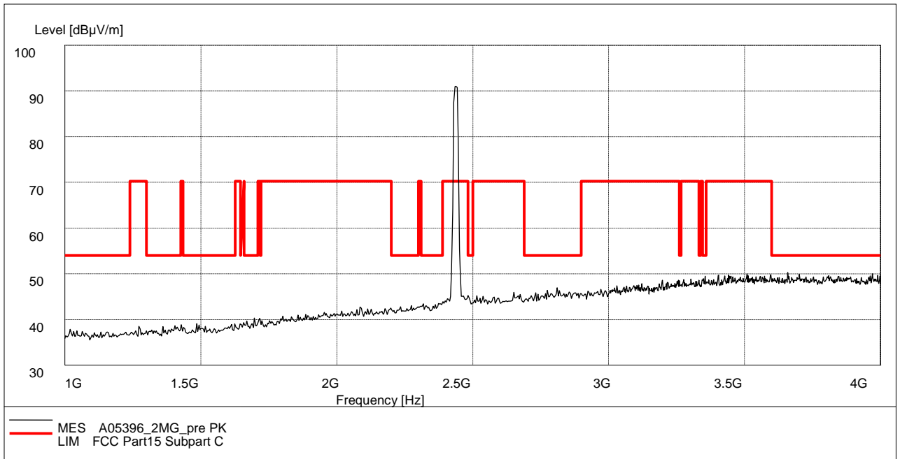
Fig. 59 Radiated Spurious Emission (802.11g, Ch6, 1 GHz-4 GHz)
