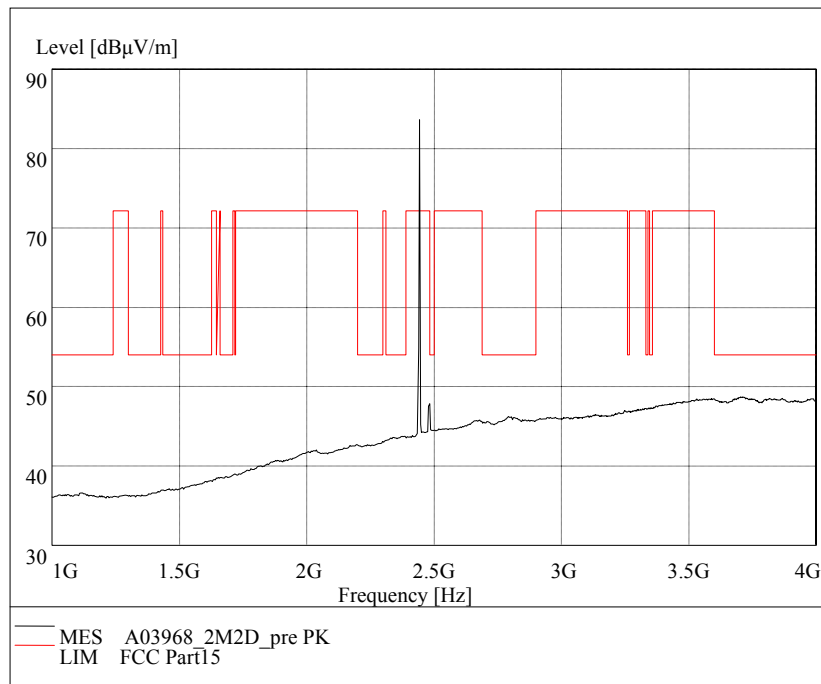
Fig.74. Radiated emission: \pi/4 DQPSK, Channel 39, 1 GHz - 4 GHz
