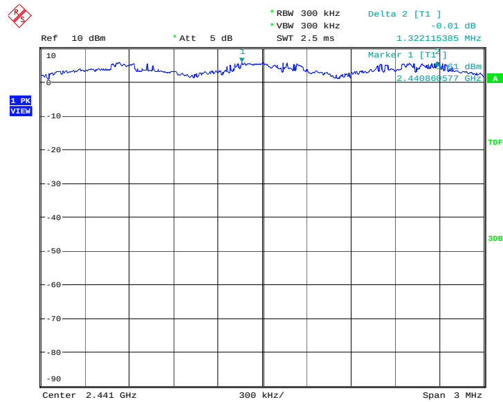
Fig.121. Carrier frequency separation measurement: GFSK, Channel 39
