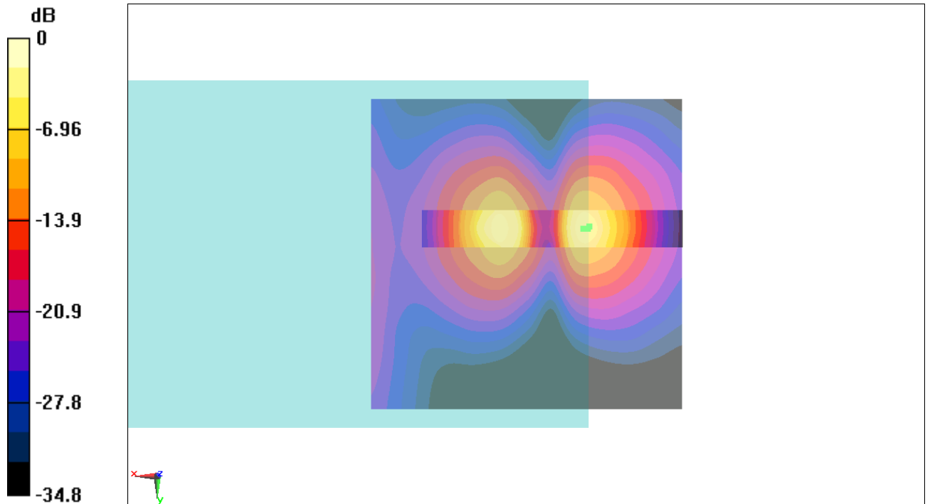
Fig B.1 T-Coil GSM 850
