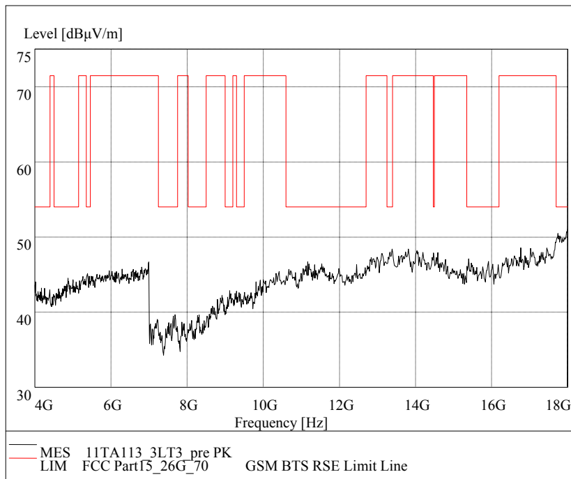
Fig.84. Radiated emission: 8DPSK, Channel 0, 4 GHz - 18 GHz
