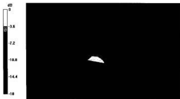
0 dB = 12.8mW/g
