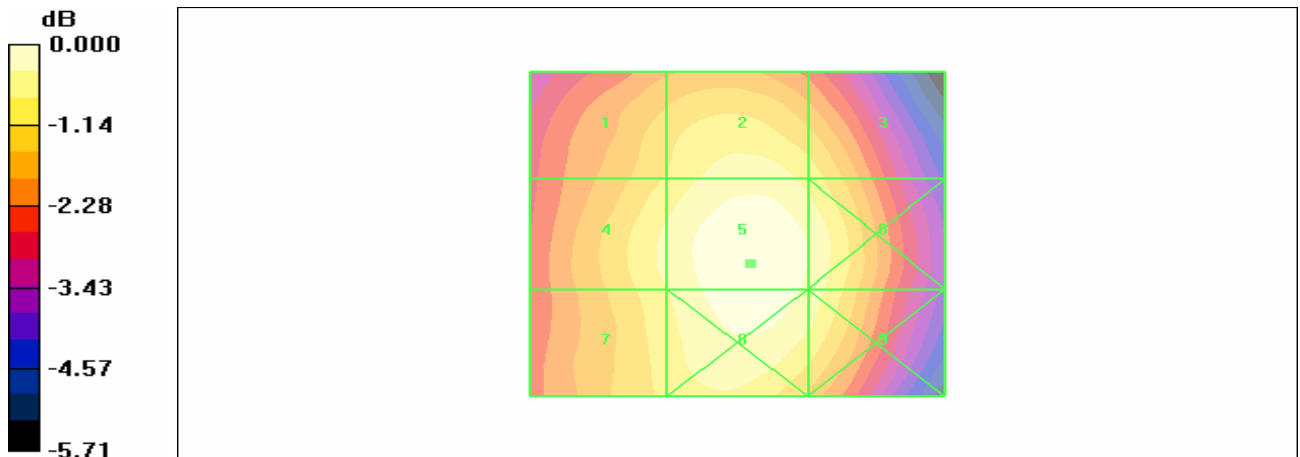
Figure 13 HAC RF E-Field GSM 850 Channel 190
