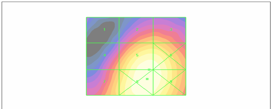
Figure 24 HAC RF E-Field WCDMA Band IV Channel 1513
