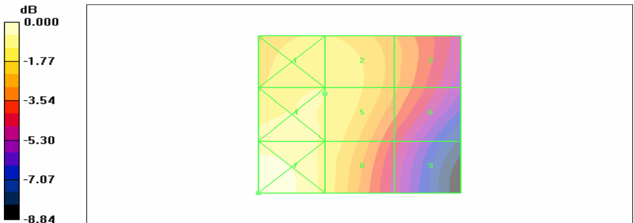
Figure 23 HAC RF H-Field GSM 1900 Channel 512
