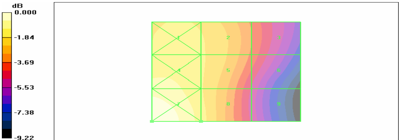
Figure 27 HAC RF H-Field WCDMA Band IV Channel 1513
