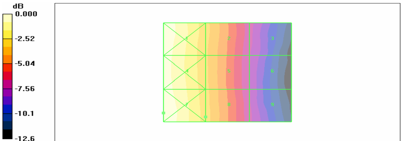
Figure 16 HAC RF H-Field GSM 850 Channel 190
