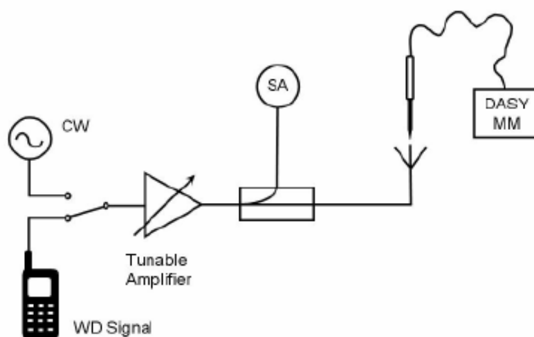
Figure 7 Probe Modulation Factor Test Setup
