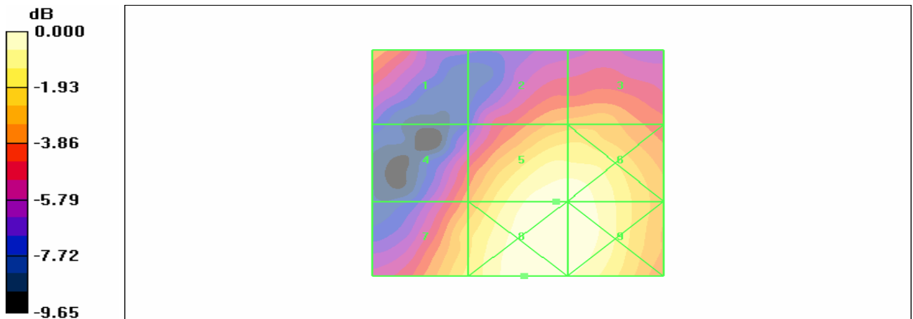
Figure 19 HAC RF E-Field GSM 1900 Channel 661
