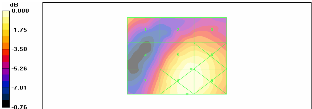
Figure 18 HAC RF E-Field GSM 1900 Channel 810
