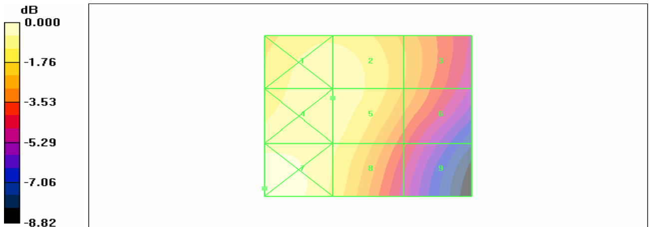
Figure 22 HAC RF H-Field GSM 1900 Channel 661
