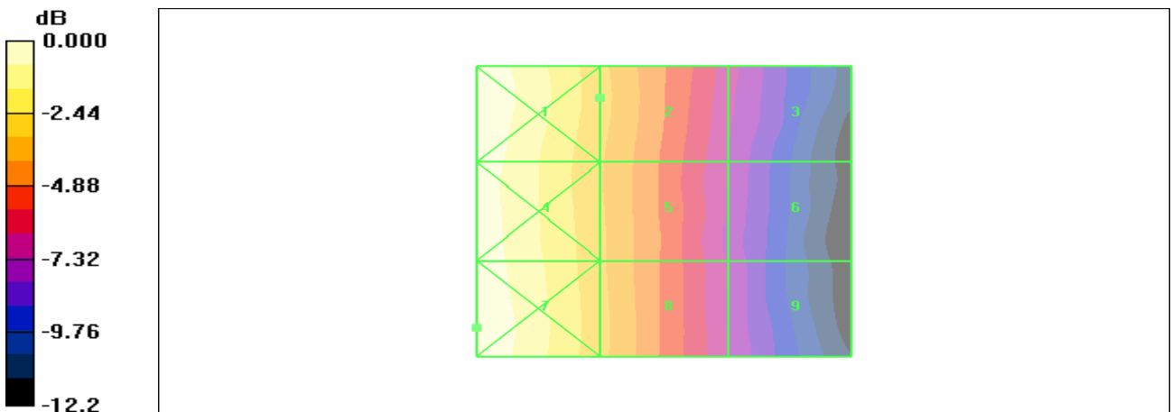
Figure 15 HAC RF H-Field GSM 850 Channel 251
