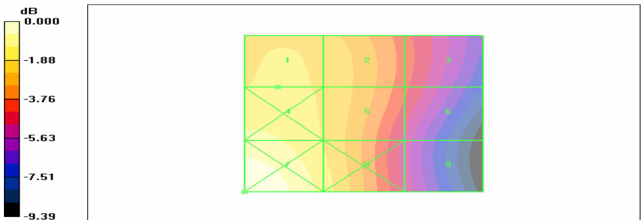
Figure 28 HAC RF H-Field WCDMA Band IV Channel 1413
