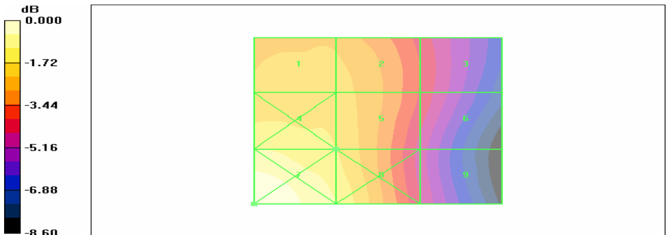
Figure 29 HAC RF H-Field WCDMA Band IV Channel 1312
