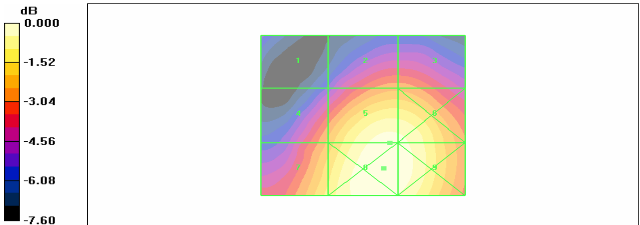
Figure 26 HAC RF E-Field WCDMA Band IV Channel 1312
