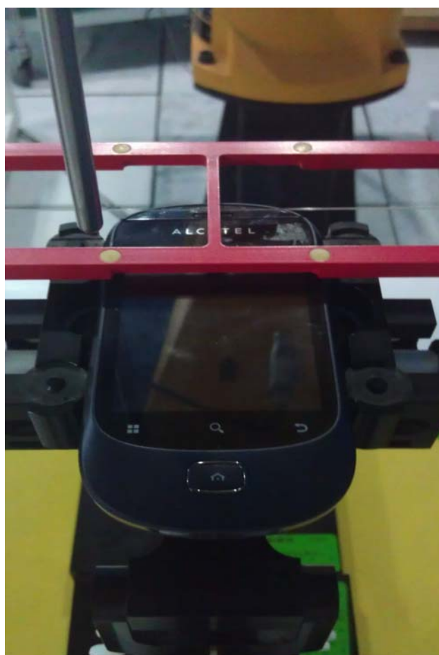
Picture 2: EUT Positioning for T-coil
