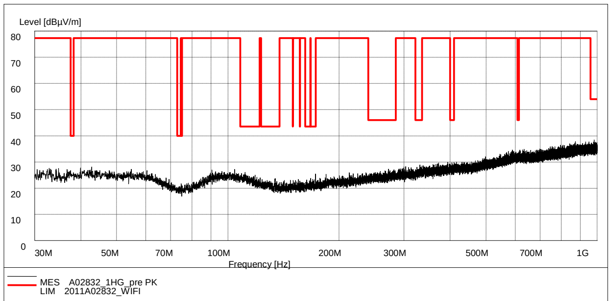
Fig. 116 Radiated Spurious Emission (802.11g, Ch11, 30 MHz-1 GHz)
