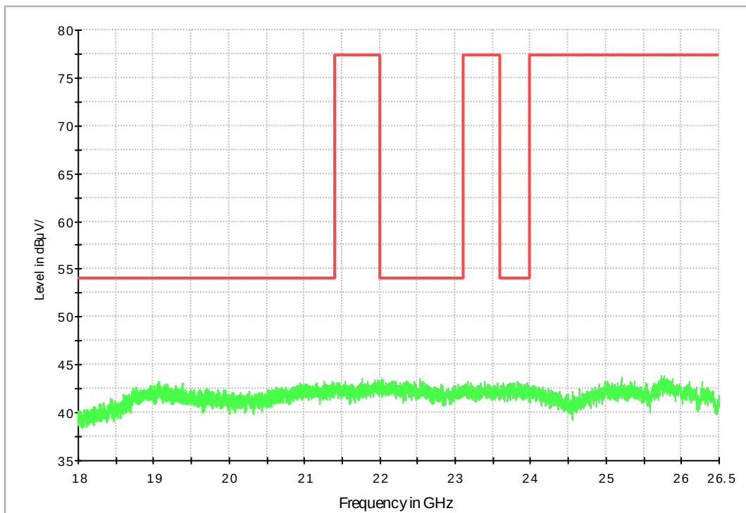
Fig. 130 Radiated emission: 18 GHz - 26.5 GHz
