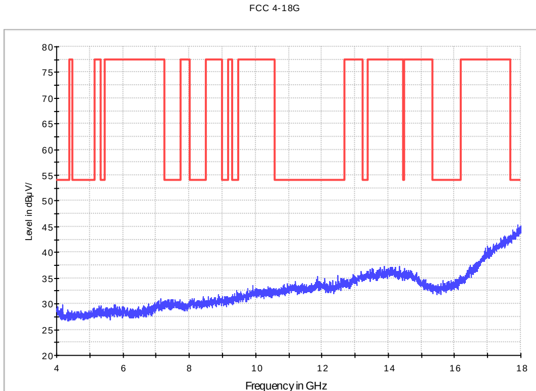
Fig. 118 Radiated Spurious Emission (802.11g, Ch11, 4 GHz-18 GHz)
