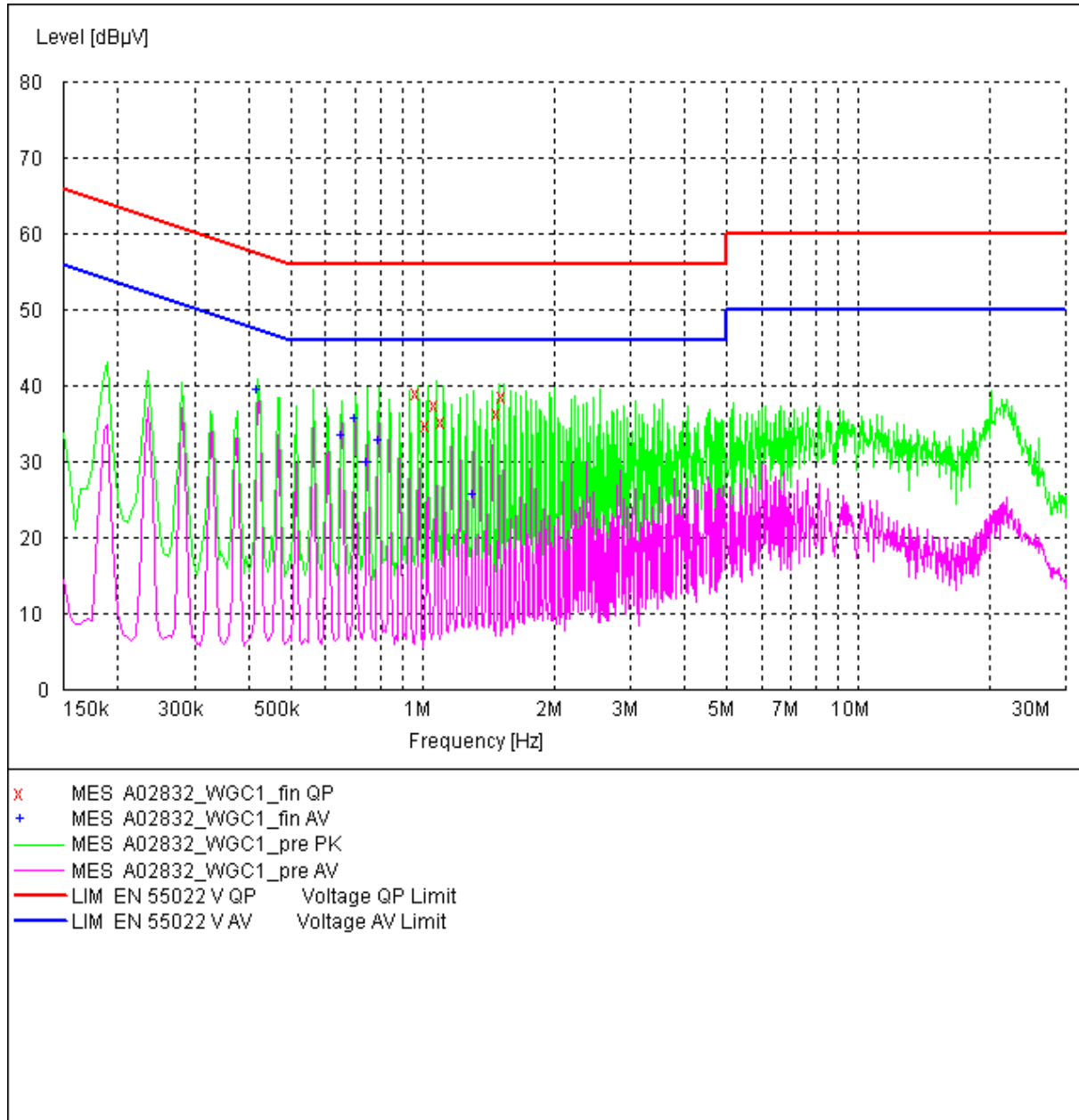
Fig. 132 AC Powerline Conducted Emission-802.11g
