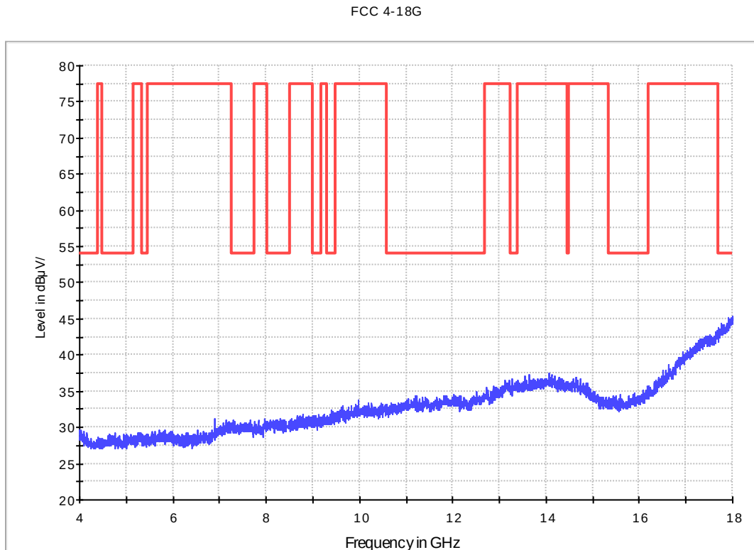
Fig. 100 Radiated Spurious Emission (802.11b, Ch1, 4 GHz-18 GHz)
