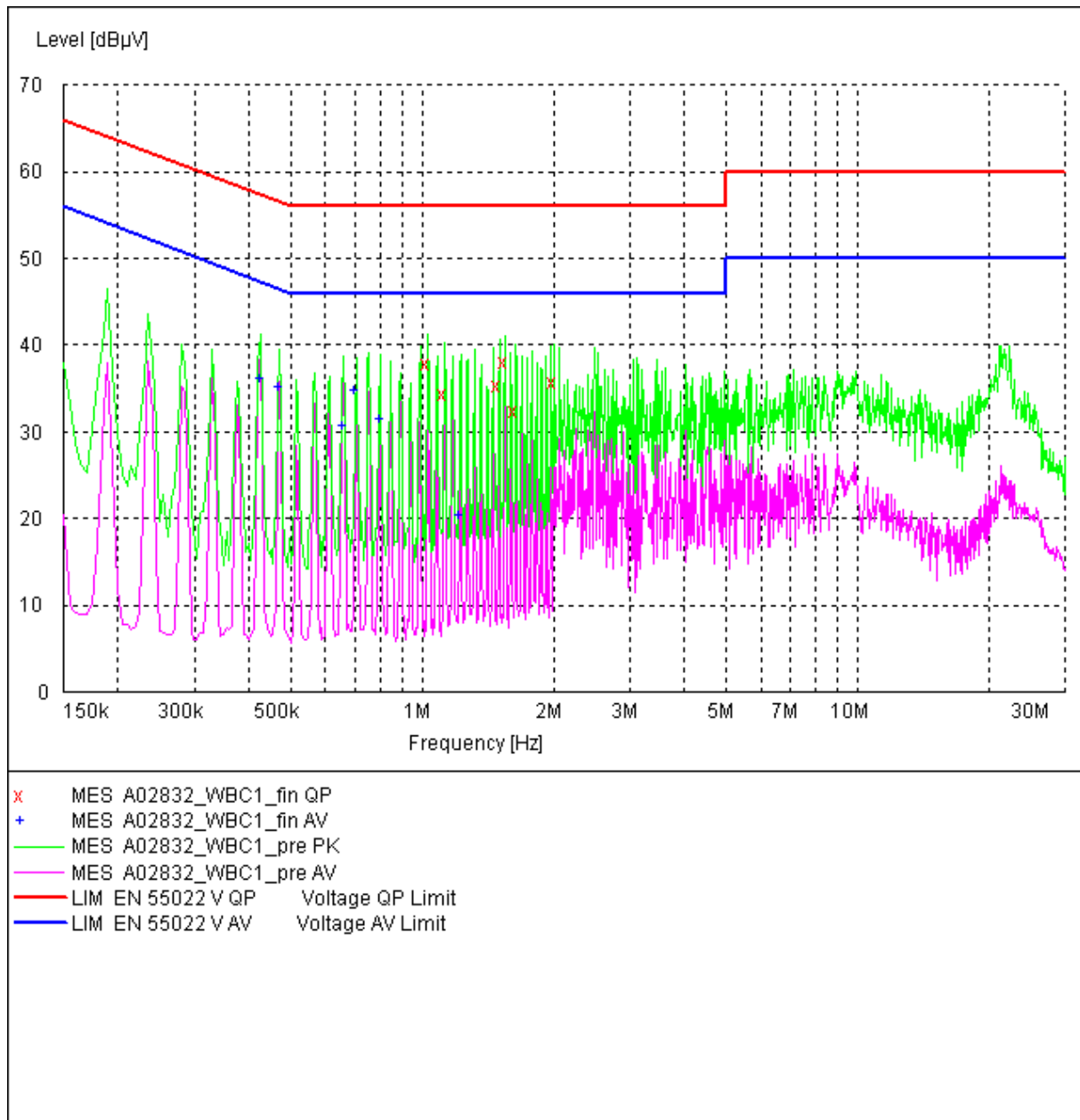
Fig. 131 AC Powerline Conducted Emission-802.11b
