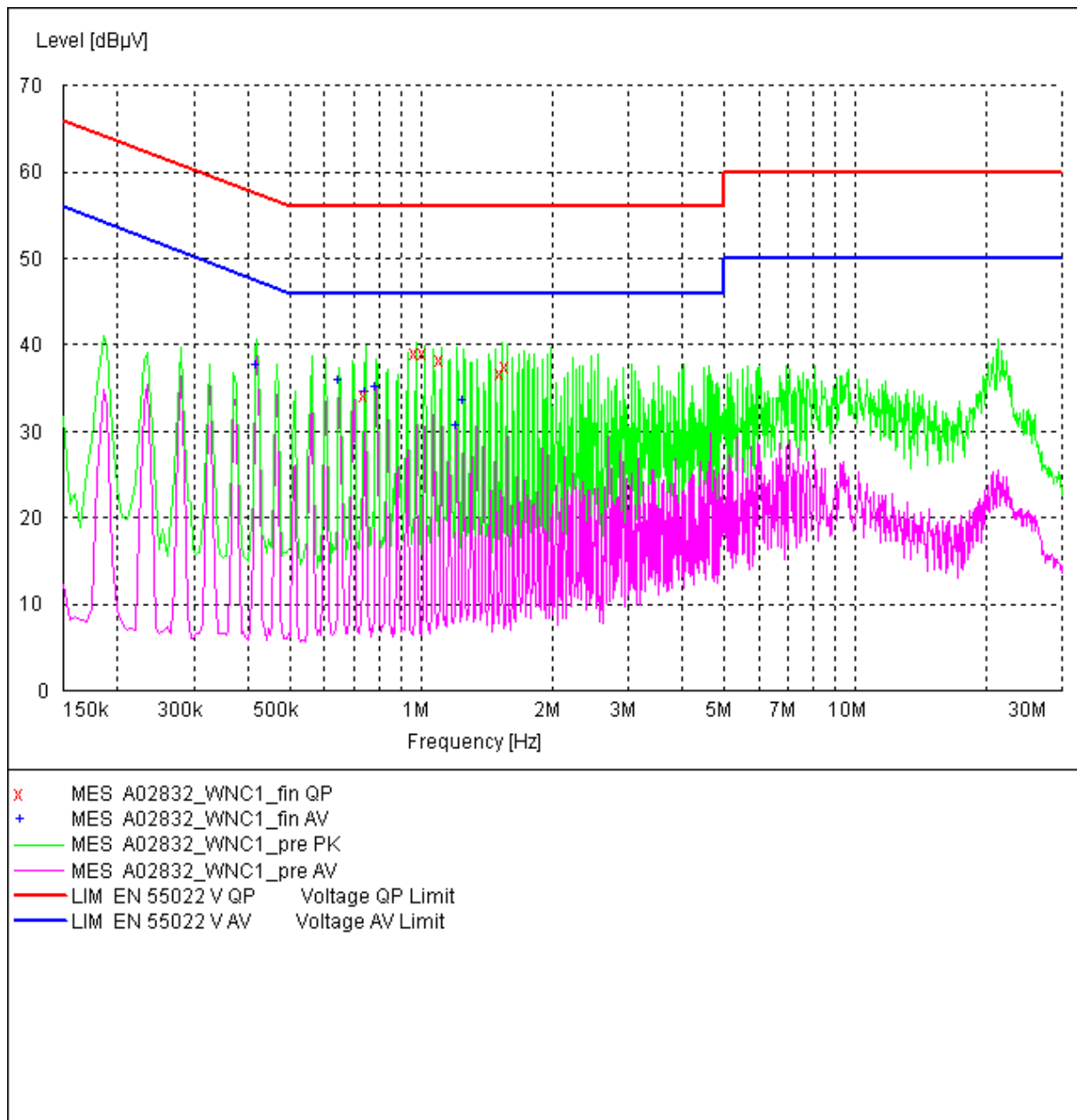
Fig. 133 AC Powerline Conducted Emission-802.11n-20MHz
