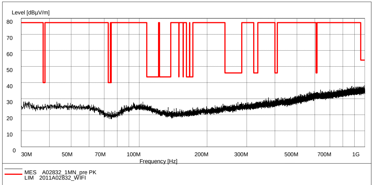
Fig. 123 Radiated Spurious Emission (802.11n-20MHz, Ch6, 30 MHz-1 GHz)
