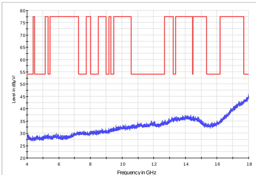
Fig. 122 Radiated Spurious Emission (802.11n-20MHz, Ch1, 4 GHz-18 GHz)
