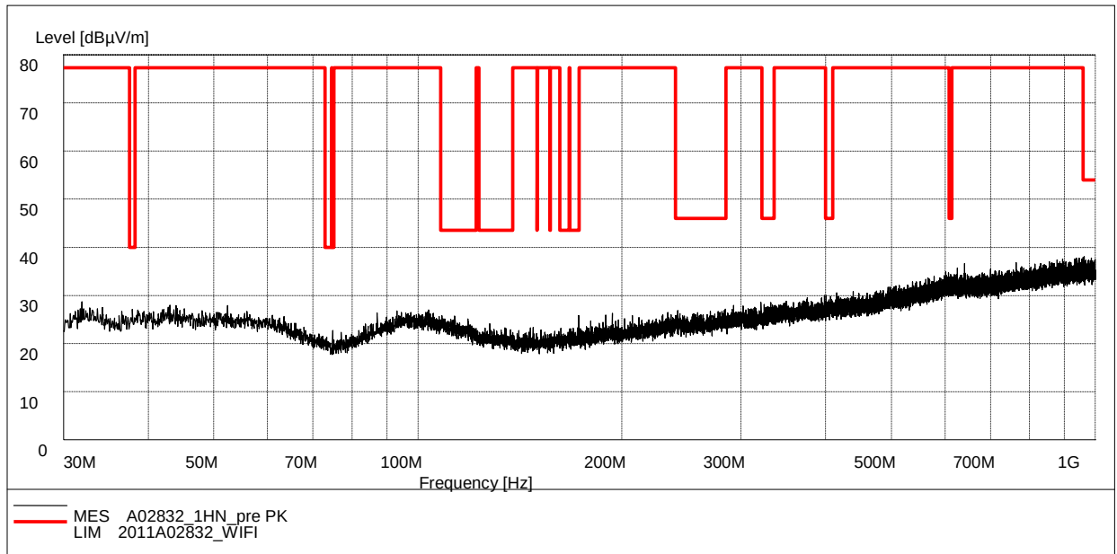
Fig. 127 Radiated Spurious Emission (802.11n-20MHz, Ch11, 30 MHz-1 GHz)
