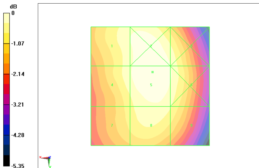
Fig B.2 HAC RF E-Field GSM 850 Middle
