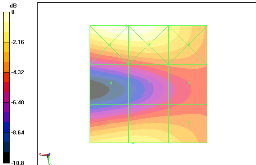
Fig B.6 HAC RF E-Field GSM 1900 Low
