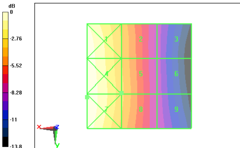
Fig B.9 HAC RF H-Field GSM 850 Low
