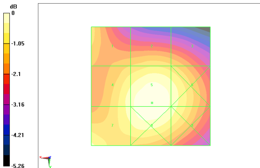
Fig B.12 HAC RF H-Field GSM 1900 Low
