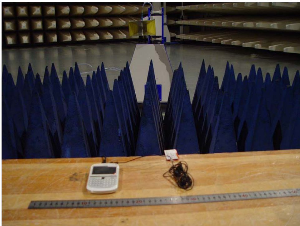
Field Strength Test setup
