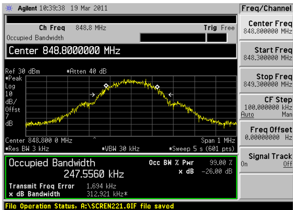
Channel 251
