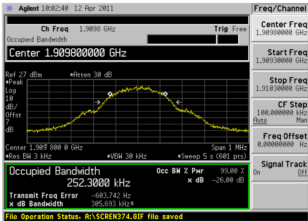
Channel 810
