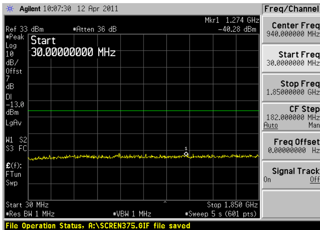
Channel 661, 30MHz~1850MHz
