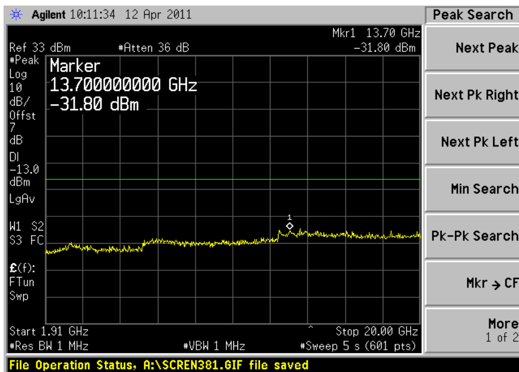
Channel 661, 1910MHz~20GHz
