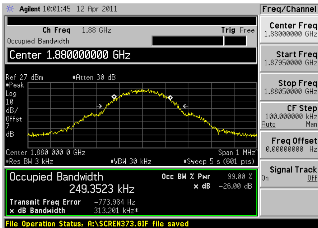
Channel 661
