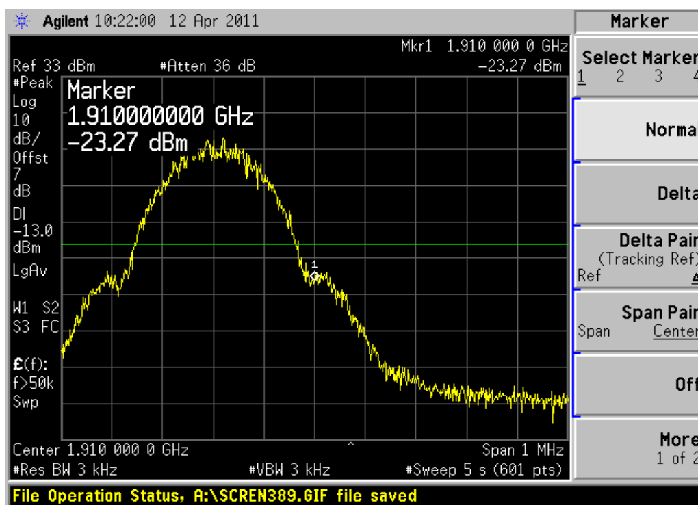
Channel 810
