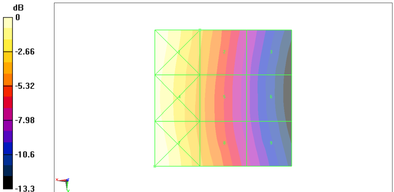
Fig B.11 HAC RF H-Field GSM 850 Middle
