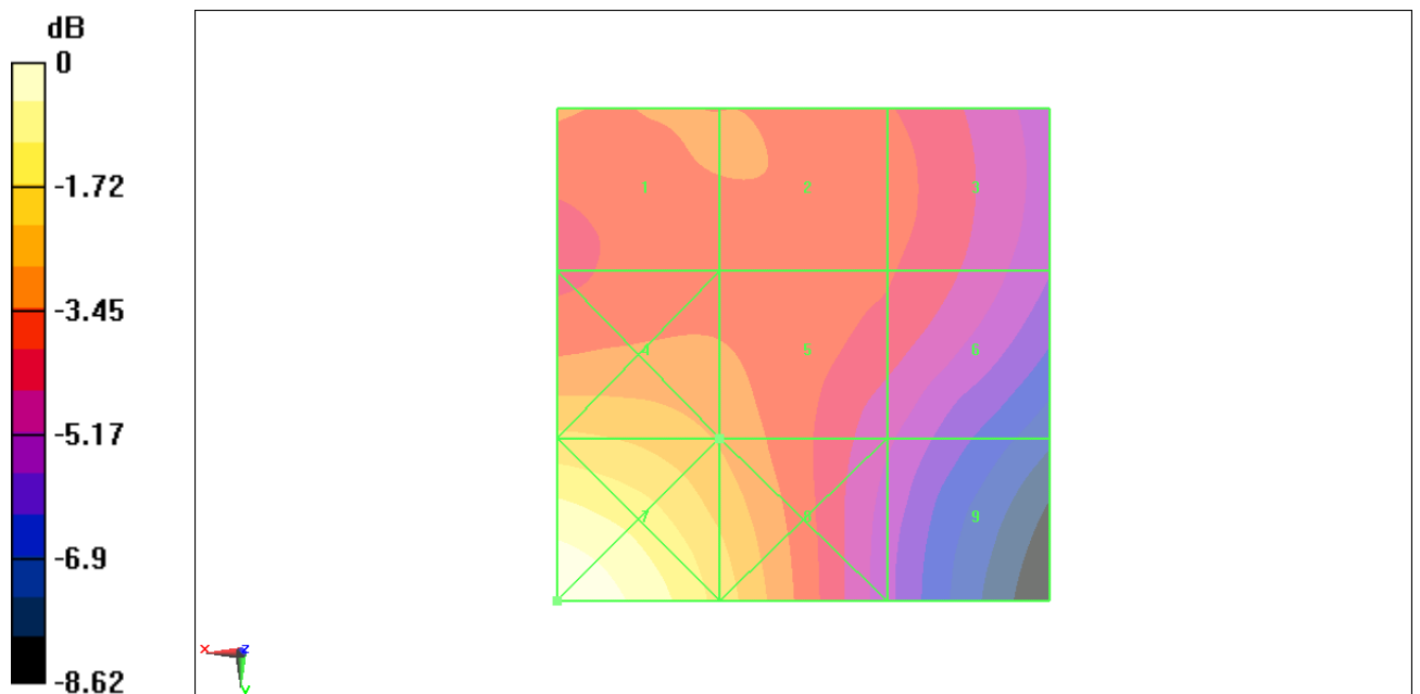
Fig B.14 HAC RF H-Field GSM 1900 Middle
