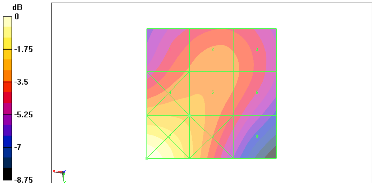
Fig B.17 HAC RF H-Field WCDMA 1700 Middle
