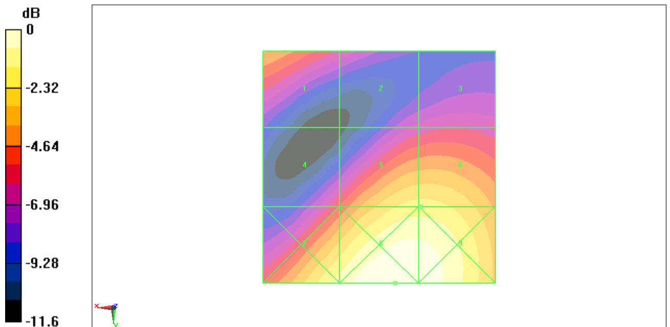
Fig B.8 HAC RF E-Field WCDMA 1700 Middle
