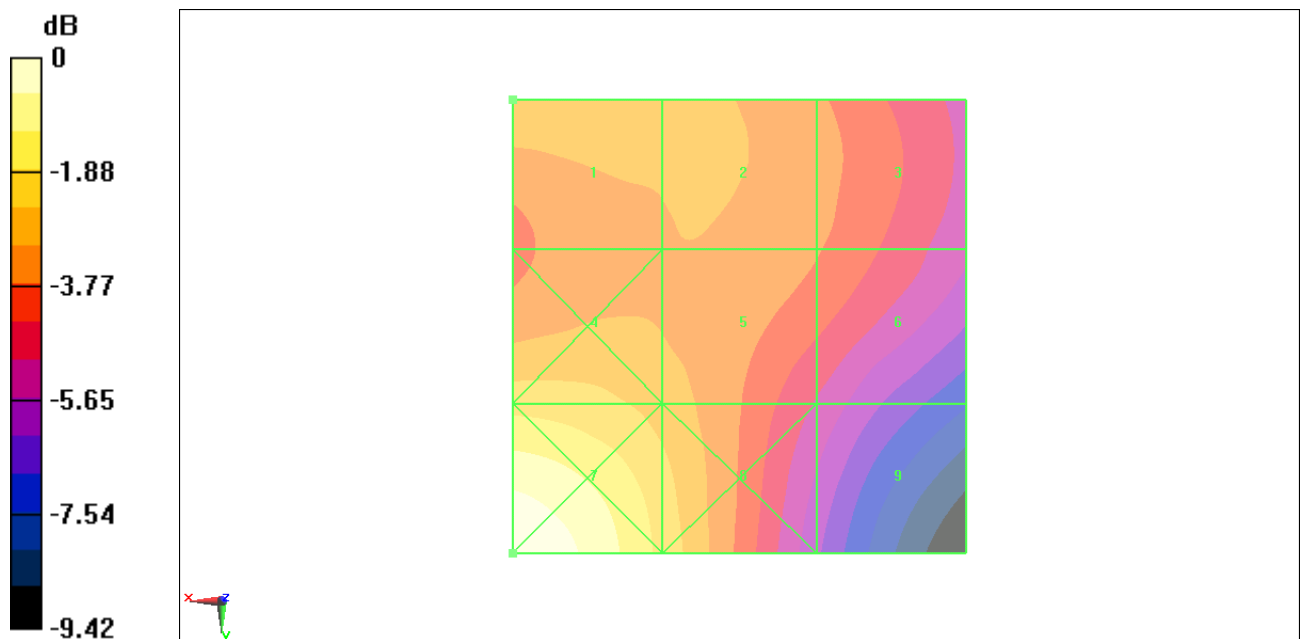
Fig B.13 HAC RF H-Field GSM 1900 High
