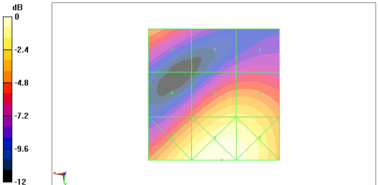
Fig B.9 HAC RF E-Field WCDMA 1700 Low
