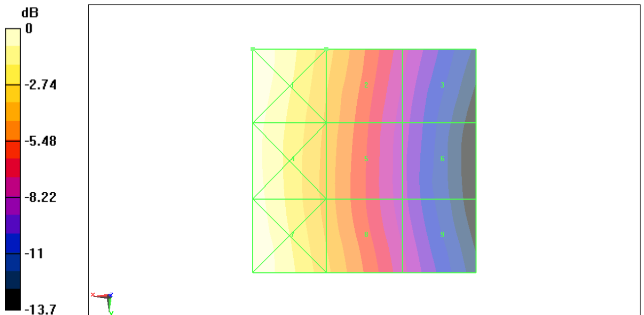
Fig B.10 HAC RF H-Field GSM 850 High
