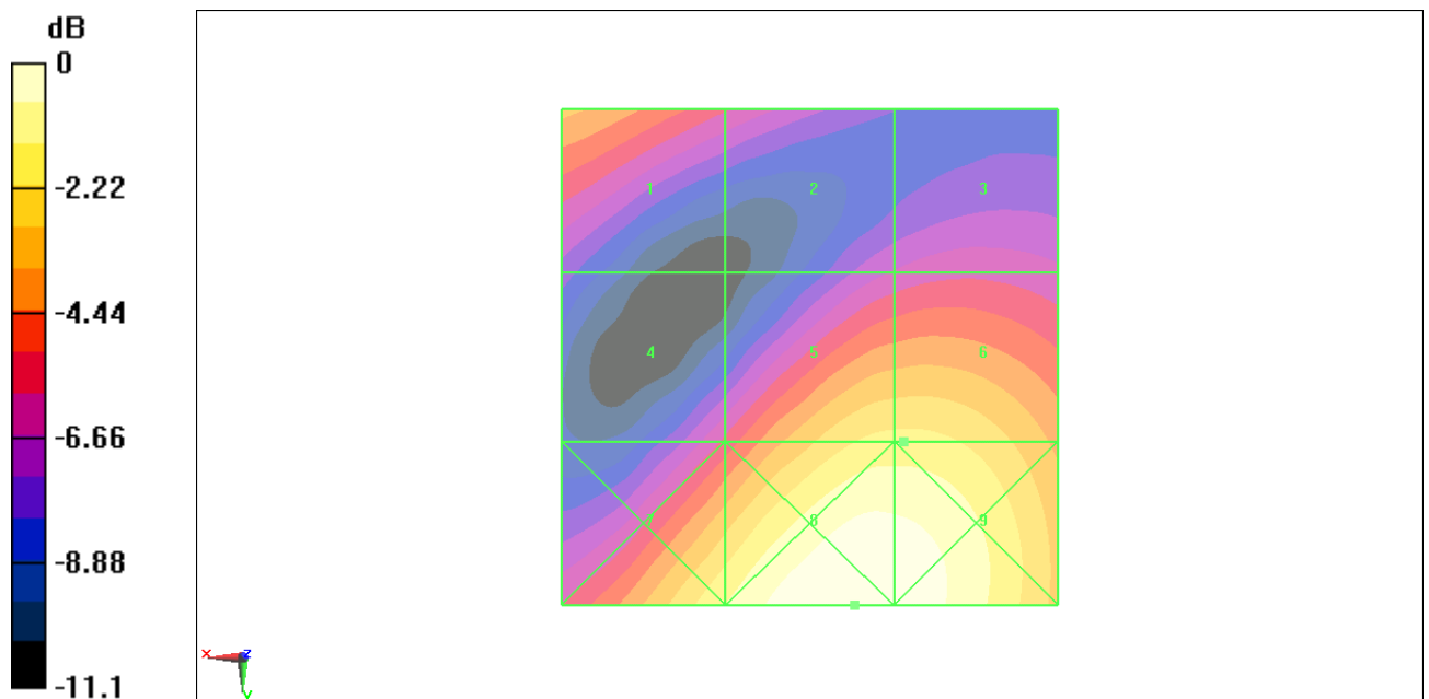
Fig B.7 HAC RF E-Field WCDMA 1700 High
