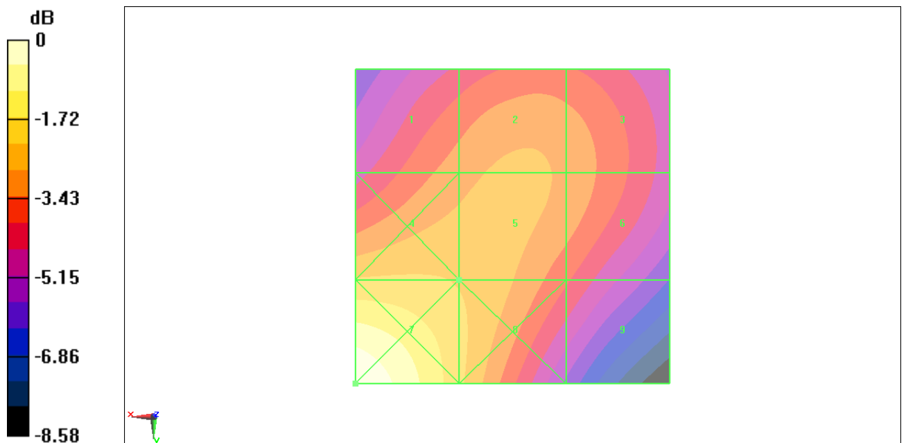
Fig B.18 HAC RF H-Field WCDMA 1700 Low
