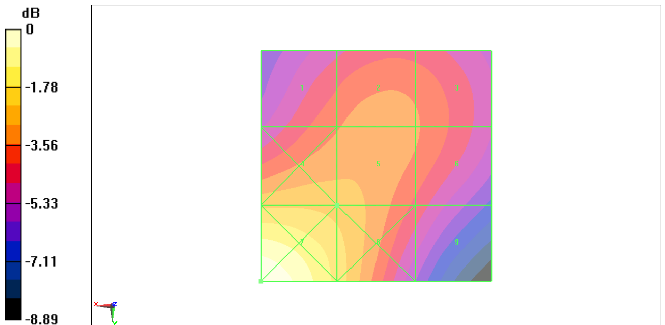
Fig B.16 HAC RF H-Field WCDMA 1700 High
