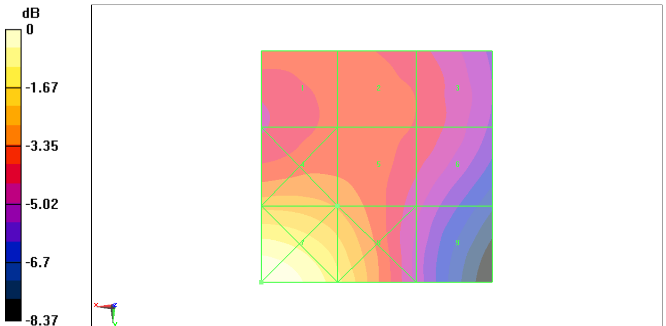
Fig B.15 HAC RF H-Field GSM 1900 Low
